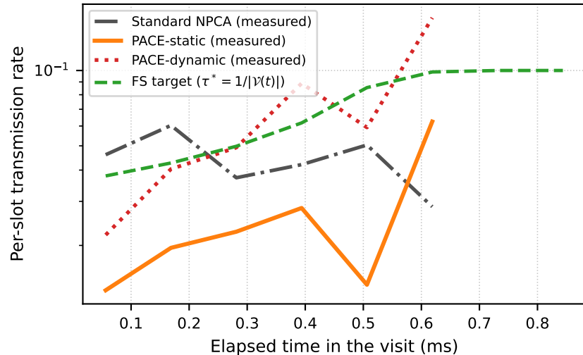
W_{\text{eff}} = 100 slots (0.90 ms): fixed c = 1.5 vs dynamic c = 2.76
