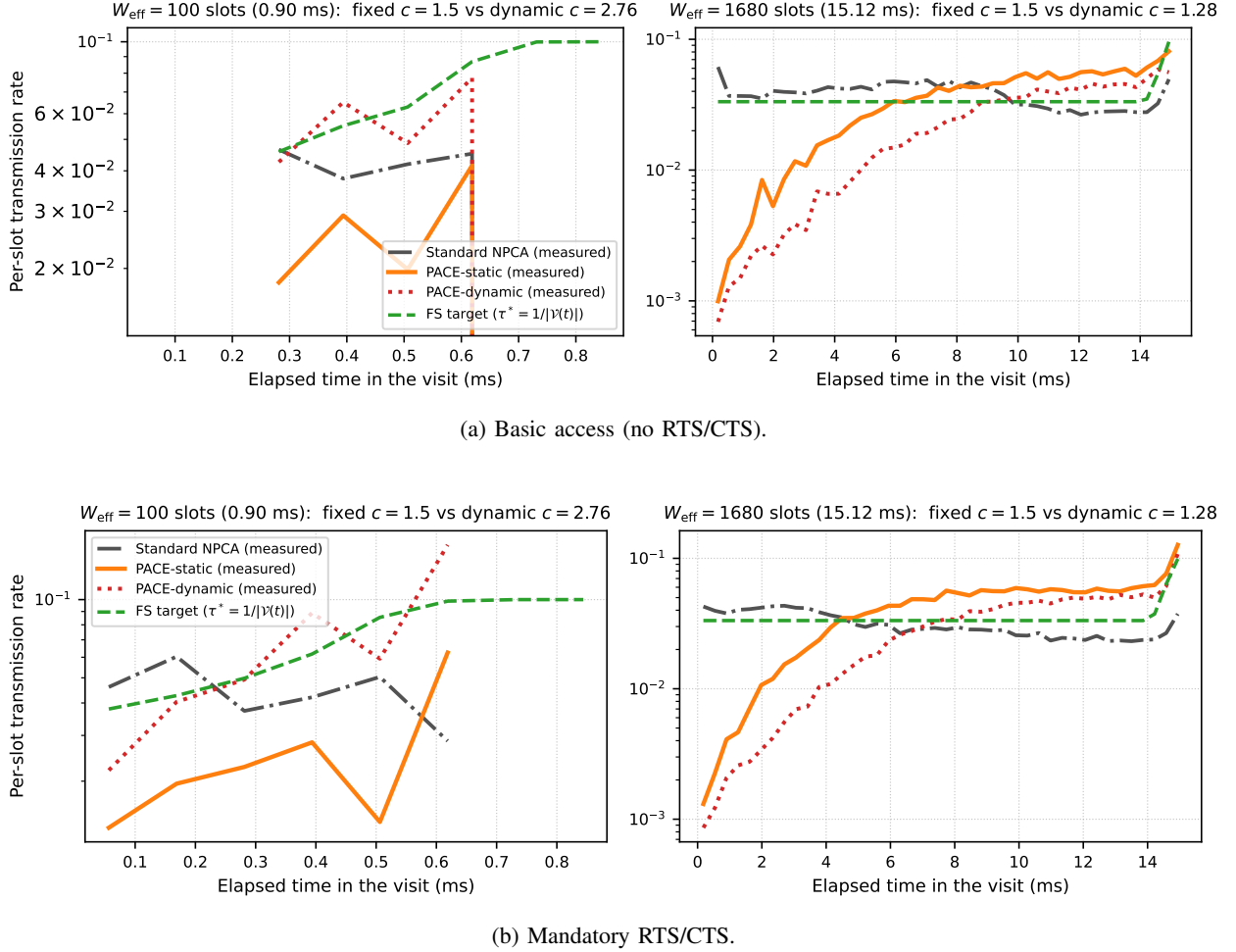
Fig. 9: Within-visit transmission dynamics at the two ends of the window sweep of Fig. 6 ( W_{\text{eff}} of 100 and 1680 slots, 0.9 and 15.1 ms, N_{\text{vis}} = 20 , N_{\text{nat}} = 10 ). PACE-static keeps the fixed factor c = 1.5 at both windows, while PACE-dynamic recomputes it per visit, c = 2.76 at the short window and c = 1.28 at the long one.
