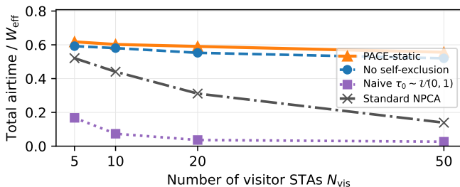
Fig. 10: Ablation study. Total useful airtime in the setting of Fig. 4 under basic access, with the RTS/CTS values quoted in the text.
