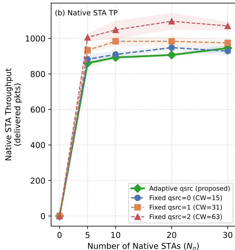
Fig. 9 Ext — Adaptive vs Fixed qsrc: Trans / Native / Total Throughput ( N_t=20 , OBSS occ.=30%)
