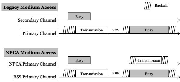
Fig. 1. The medium access process comparison between legacy and NPCA.
