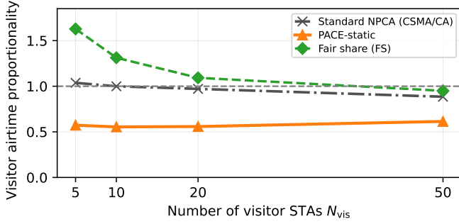
Fig. 5: Visitor airtime proportionality \rho = (\text{visitor airtime share}) / (N_{vis} / (N_{vis} + N_{nat})) versus the number of visitor STAs N_{vis} , in the same setting as Fig. 4. \rho = 1 is the proportional-fair reference. \rho > 1 means the visitors occupy more than their population share. Basic access, with the RTS/CTS values quoted in the text.
