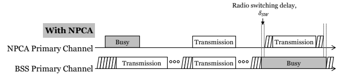
(b) With NPCA.
