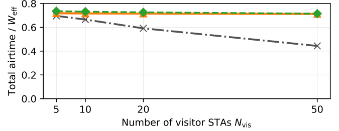
(b) RTS/CTS.
