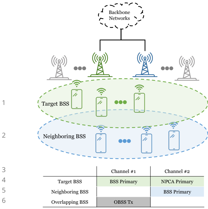
Fig. 1: Two-BSS topology and channel assignment. The STAs of the target BSS act as the visitors \mathcal{V} on Channel #2 during NPCA visits, while the STAs of the neighboring BSS are treated as natives \mathcal{N} .
