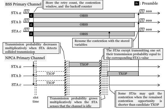
(b) Proposed PACE.
