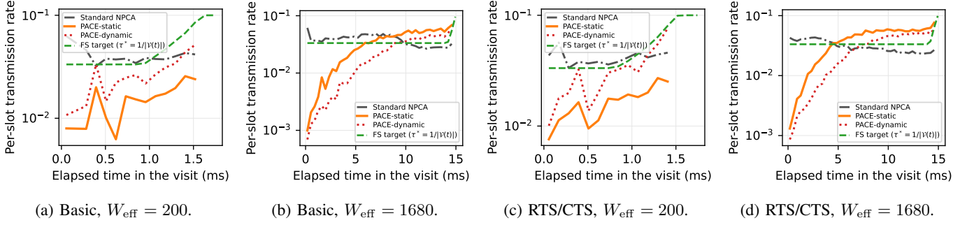
Fig. 8: Within-visit transmission dynamics at a short and a long window of the sweep of Fig. 7 ( W_{\text{eff}} of 200 and 1680 slots, 1.8 and 15.1 ms, N_{\text{vis}} = 20 , N_{\text{nat}} = 10 ), for both access modes, averaged over 500 visits. PACE-static keeps the fixed factor c = 1.5 at every window, while PACE-dynamic recomputes it per visit, c = 2.05 at the short window and c = 1.28 at the long one. Measured curves are drawn while more than two visitor frames on average still fit the remaining window. Under RTS/CTS the handshake must also fit, so this point arrives slightly earlier.
