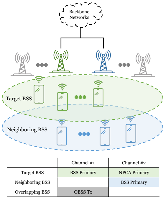
Fig. 1: Two-BSS topology and channel assignment. The STAs of the target BSS act as the visitors \mathcal{V} on Channel #2 during NPCA visits, while the STAs of the neighboring BSS are treated as natives \mathcal{N} .
