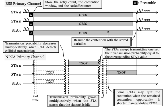
(b) Proposed PACE.
