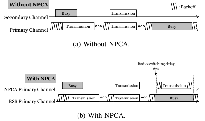
Fig. 2: The medium access process comparison with and without NPCA.
