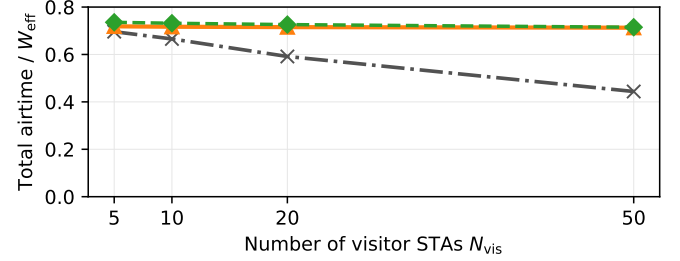
(b) RTS/CTS.
