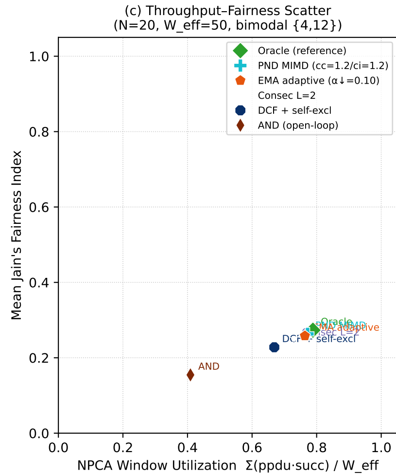
Fig. 20 Throughput-Fairness Tradeoff — PPDU-Class Fairness Analysis (bimodal {4,12}, N \in \{10, 20, 30, 50\} , PND cc=1.2/ci=1.2 ) (a) Jain's Fairness Index vs N (W_eff=50, bimodal {4,12}) (b) Per-Class success rate (N=20, W_eff=50, bimodal {4,12}) (c) Throughput-Fairness Scatter (N=20, W_eff=50, bimodal {4,12})
