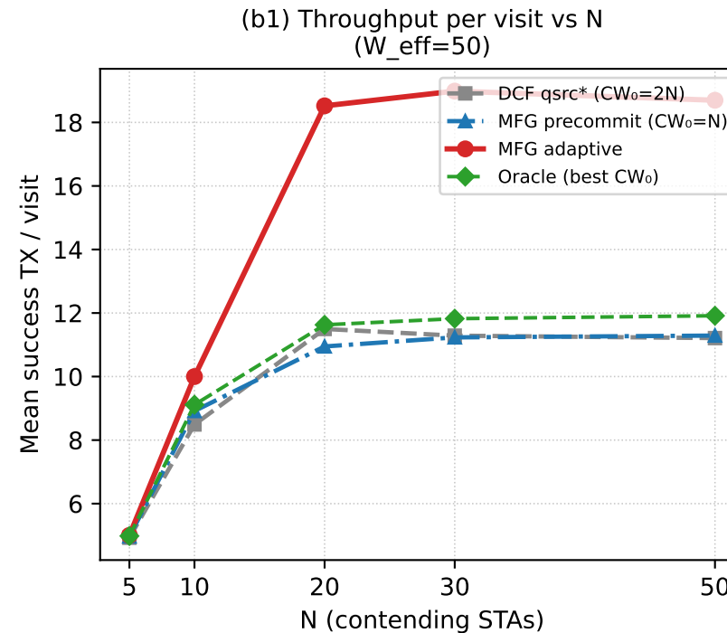
Fig. 15 MFG-Optimal vs DCF-Static Backoff — Finite-Horizon NPCA Contention (NPCA visit model: N STAs \times W_{\text{eff}} available slots, BEB retries within visit)
