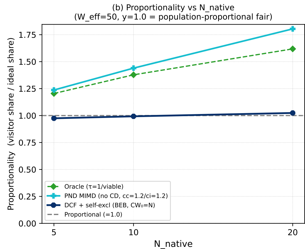
Fig. 21 Native vs. Visitor Fairness — Mixed NPCA Contention ( N_{\text{visitor}}=10 , N_{\text{native}} \in [0, 5, 10, 20] , bimodal visitor {4,12}, native ppdu=6, PND cc=1.2/ci=1.2)
