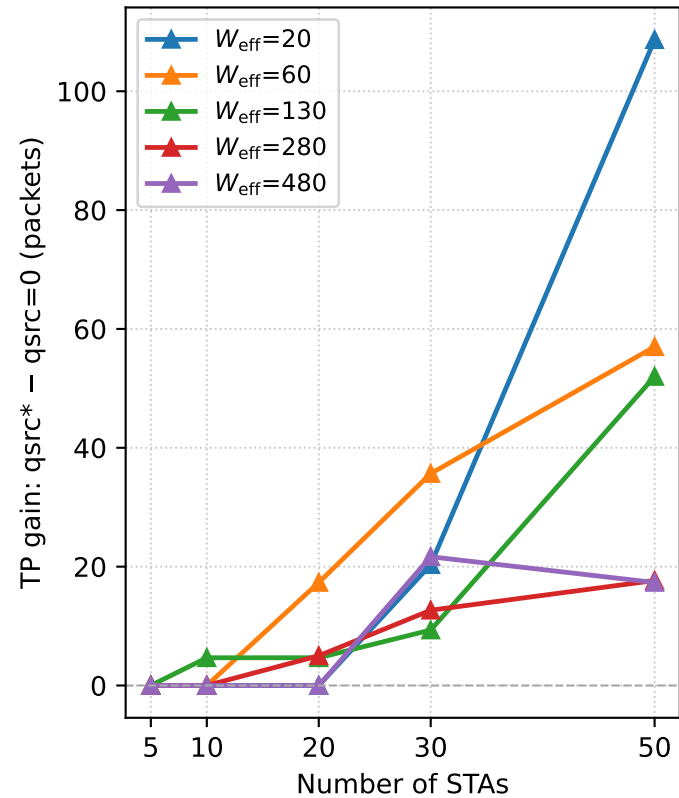
(c) Absolute gain from qsrc optimization largest at short W_{\text{eff}} + high N
