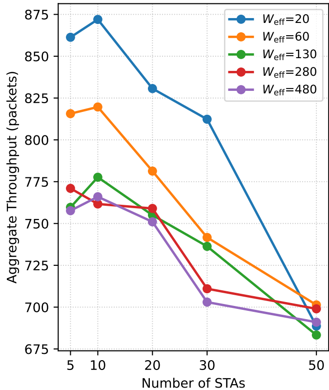
(a) Throughput vs N — qsrc = 0 short W_{\text{eff}} hurts at high N
