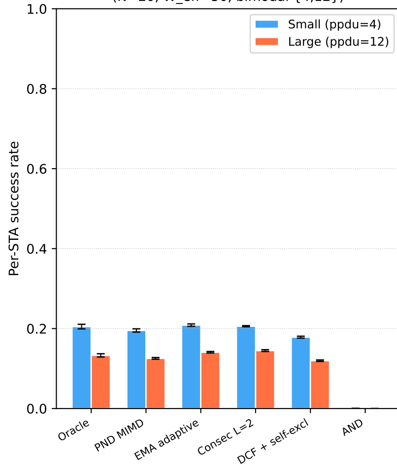
Fig. 20 Throughput-Fairness Tradeoff — PPDU-Class Fairness Analysis (bimodal {4,12}, N \in \{10, 20, 30, 50\} , PND cc=1.2/ci=1.2 ) (a) Jain's Fairness Index vs N (b) Per-Class success rate ( N=20, W_{\text{eff}}=50 , bimodal {4,12})
