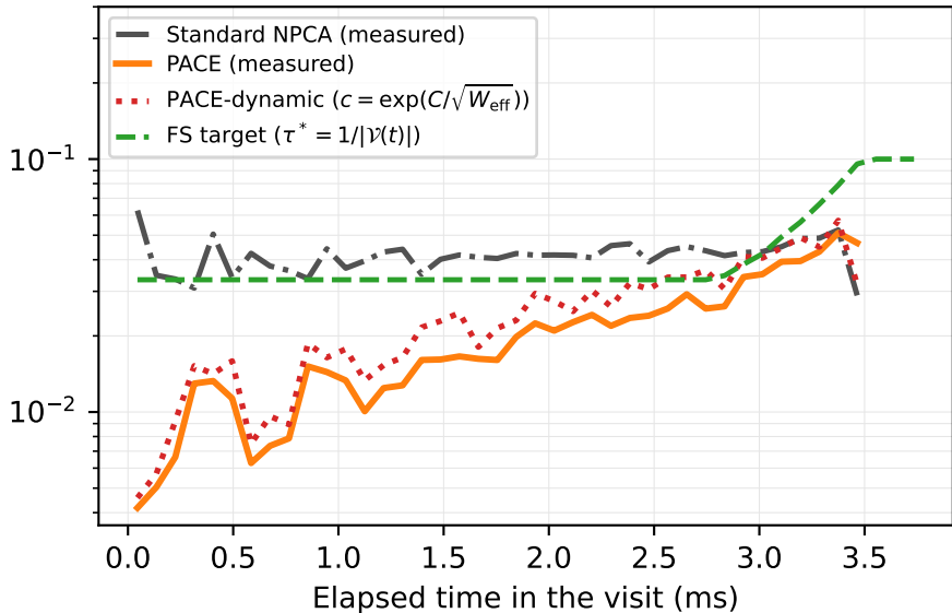
Per-slot transmission rate
