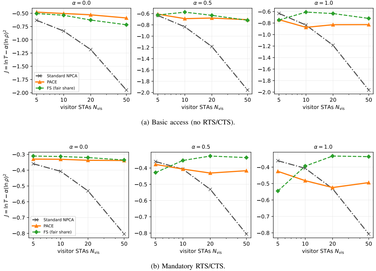
Fig. 6: The combined objective of Eq. (13) versus the number of visitor STAs, in the setting of Fig. 4, for proportionality weights \alpha \in \{0, 0.5, 1\} .
