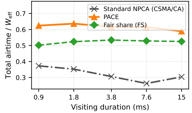
(a) Basic access (no RTS/CTS).
