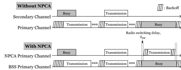
Figure 2: The medium access process comparison with and without NPCA.
