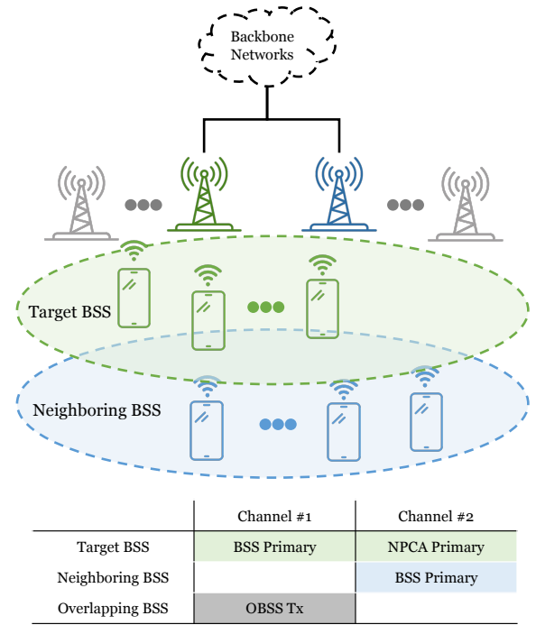
Figure 1: Two-BSS topology and channel assignment.
