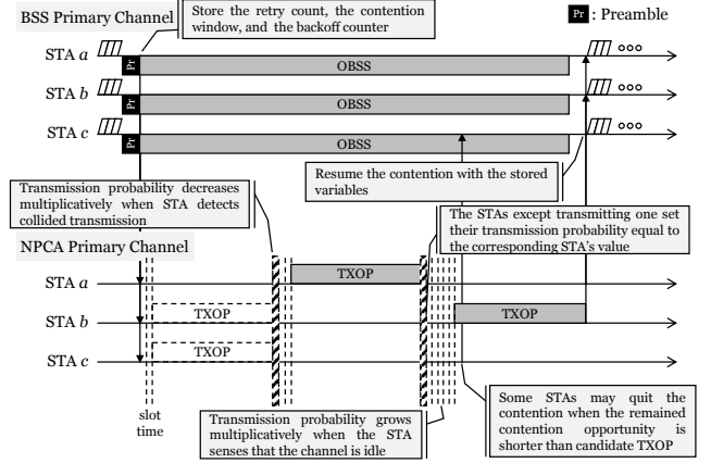
(b) Proposed PACE (probabilistic adaptive contention).
