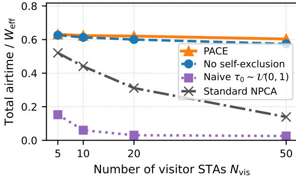
(a) Basic access (no RTS/CTS).
