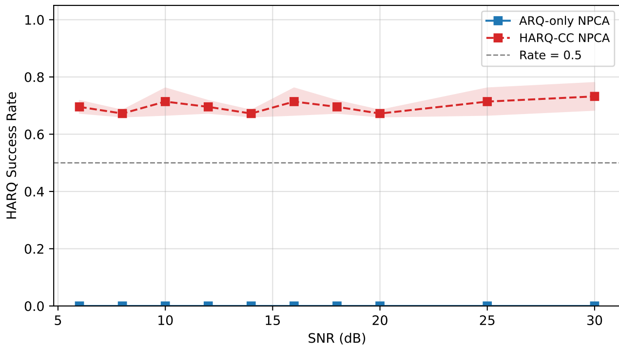
(b) HARQ Success Rate vs SNR
