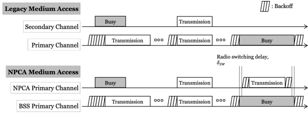
Fig. 1: The medium access process comparison between legacy and NPCA.
