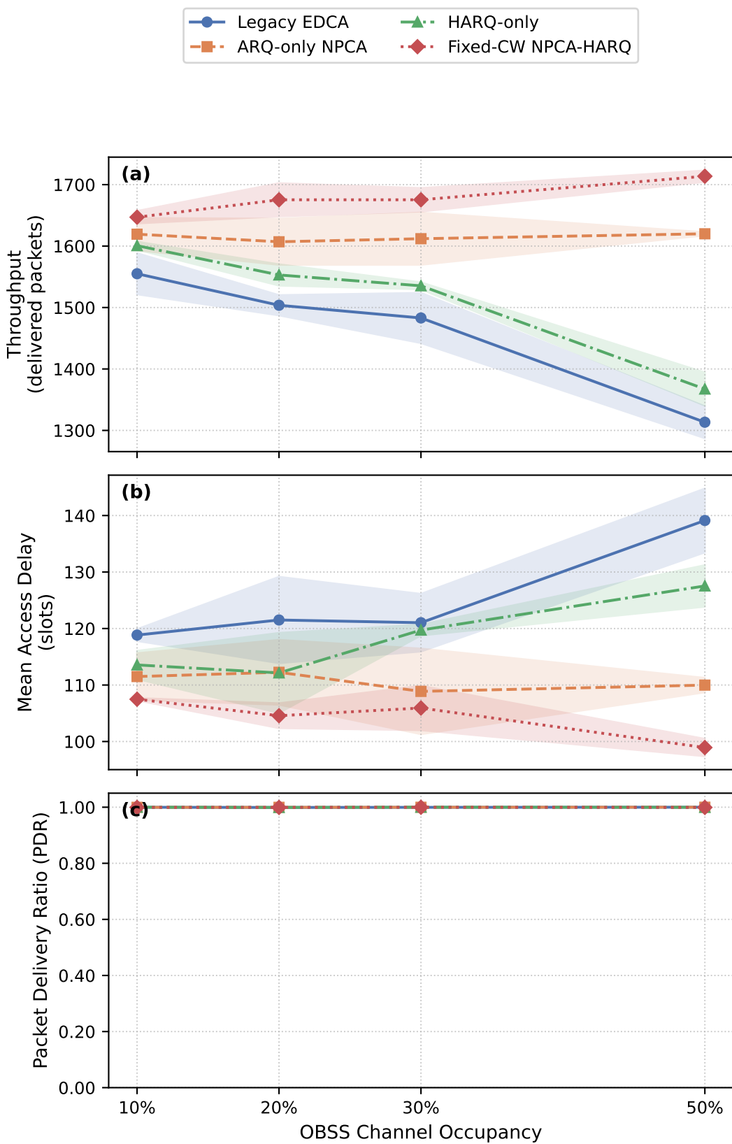
Fig. 1 NPCA-HARQ Combination Gain vs. Baselines
