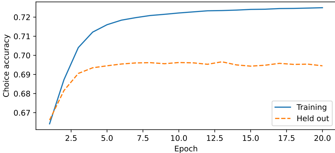
Flexible head, seed 101
