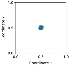
Epoch 0
