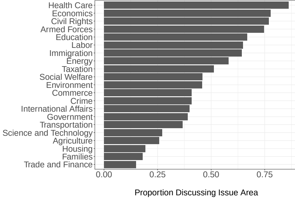
Figure 5: Proportion of Incoming Members Discussing Each Policy Category
