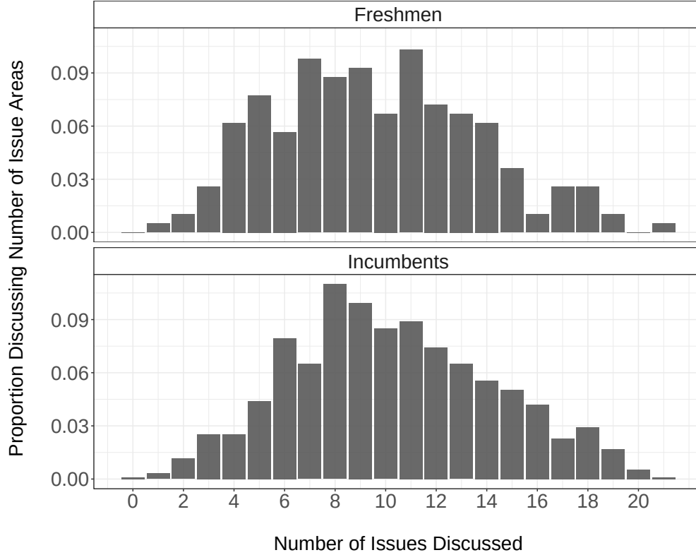
Figure 4: Number of Issue Areas Discussed by Incumbency Status
