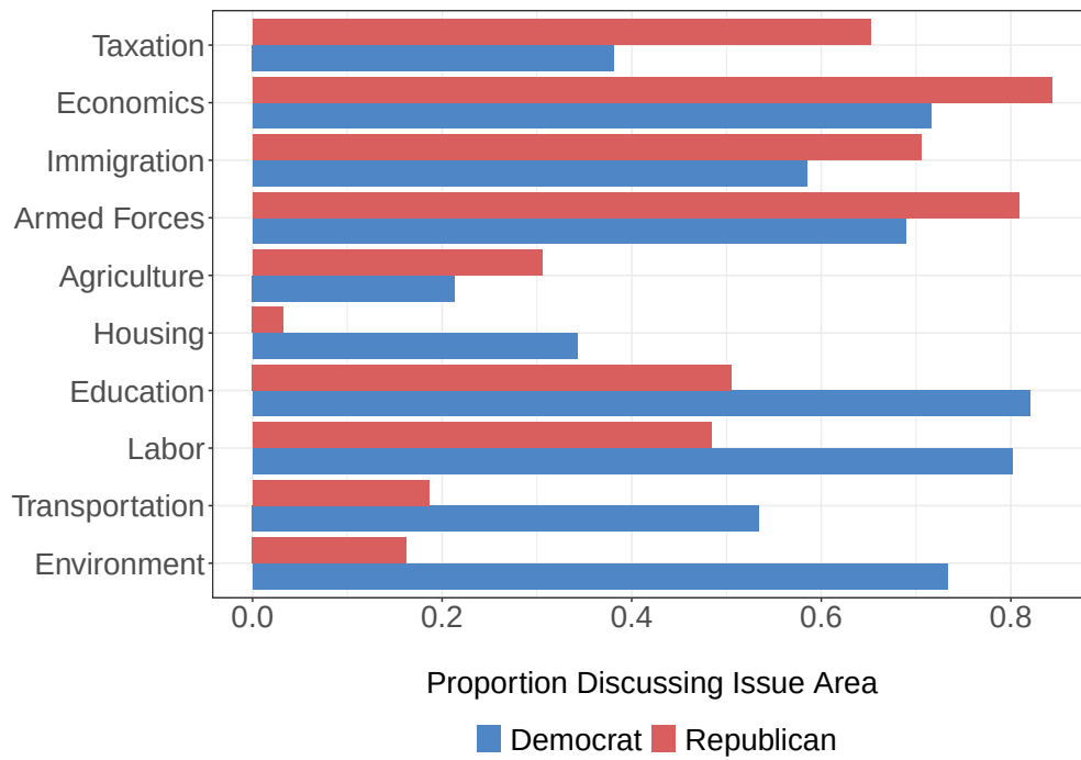
Figure 6: Proportion of Incoming Members Discussing Policy Areas, by Party
