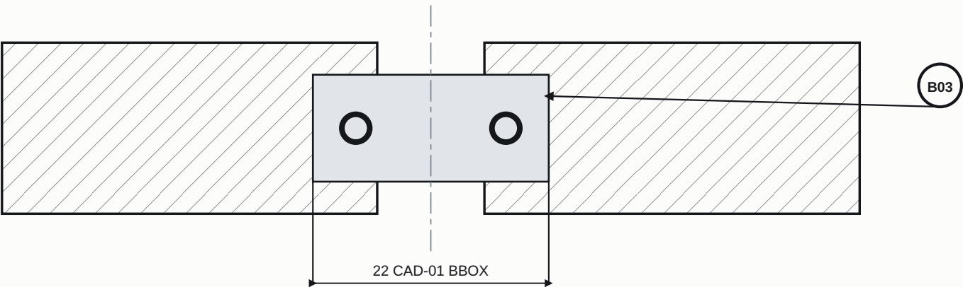
DETAIL A - 250 -> 500 SPAN JOINT SCALE NTS - DO NOT SCALE
