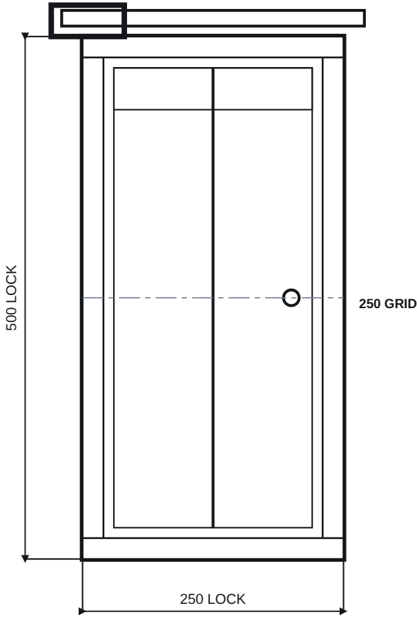
FRONT ELEVATION SCALE NTS - DO NOT SCALE
