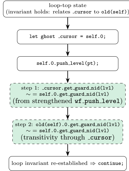
Figure 2: The step-fact/transitivity pattern applied at one push_level call site. The same shape, replacing the middle box with Entry::replace/alloc_if_none or a bare field write ( self.0.va = end; ), applies at every write and early-exit site enumerated in Table 3.
