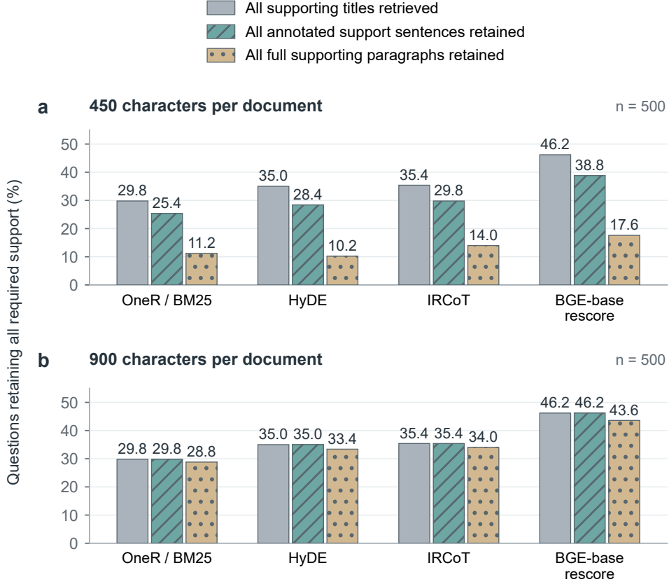
Fig. 4 Annotated evidence retention under (a) 450 and (b) 900 characters per document. Bars show complete-support question rates on 500 frozen HotpotQA IDs using the official retrospective sentence-audit labels consistently: all supporting titles retrieved, all annotated sentences retained and all full supporting paragraphs retained. One official title set differs from the primary labels; original scores remain unchanged (Online Resource 1, Section S22). BGE-base rescore is a bi-encoder, distinct from Figure 3. Coverage precedes global token clipping and does not establish human sufficiency. Bars are descriptive.
