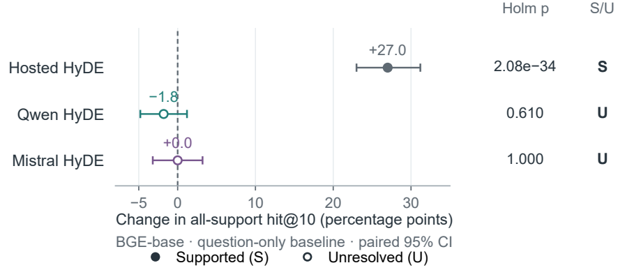
Fig. 2 Generator-conditioned retrieval contrasts. Standard HyDE minus question-only all-support hit@10 with BGE-base on the processed local (a) HotpotQA and (b) 2Wiki corpora, each with 500 questions. Points and bars show paired effects and reported 95% bootstrap intervals in percentage points. Filled (S) and hollow (U) points preserve supported and unresolved decisions from the original Holm families, not a newly pooled six-row family. All HotpotQA decisions remain unresolved despite intervals excluding zero. Hosted/local differences include implementation and output budgets.
