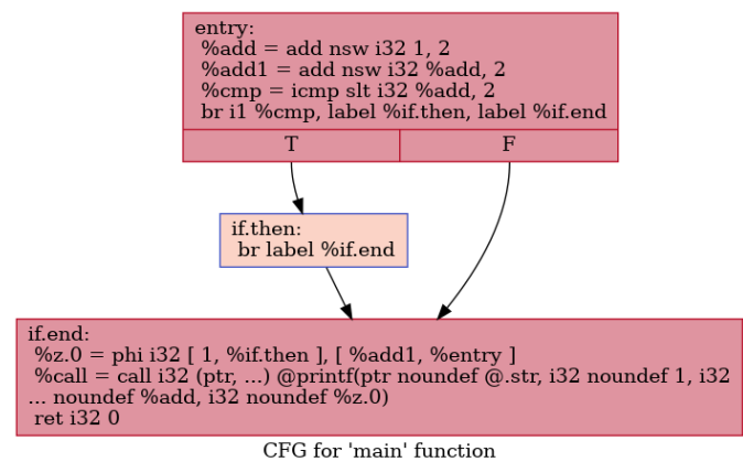
Figure 3: CFG of input.ll
