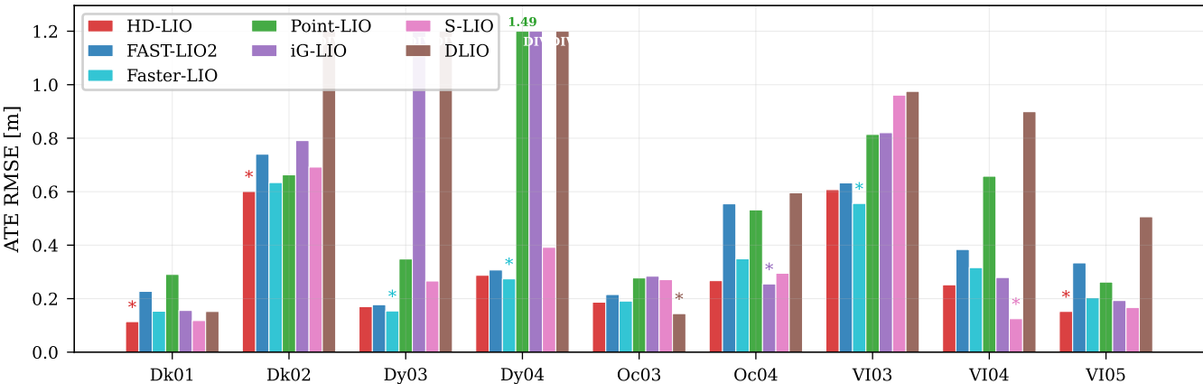
ATE RMSE Comparison — M3DGR (Avia)
