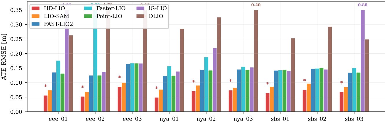
ATE RMSE Comparison — NTU VIRAL
