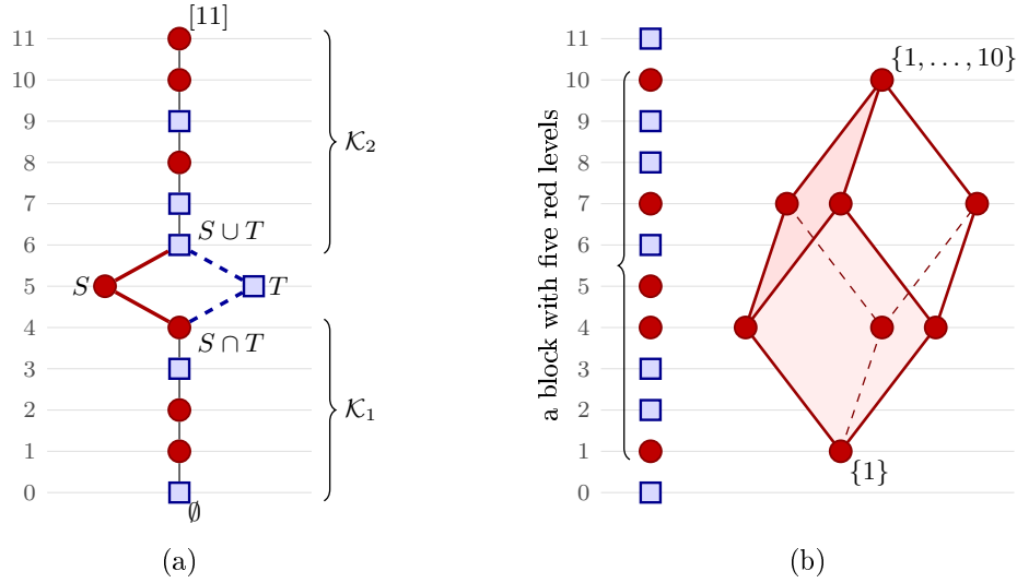
FIGURE 9. The two cases of Lemma 7.1, with red discs and blue squares and the levels of 2^{[11]} drawn horizontally. (a) Lemma 7.2: a maximal chain through S \cap T and S \cup T is shared by the two colours, S is added to the red sets and T to the blue sets, and the pair has 13 members. (b) The cardinality colouring given by the word BRBBRRBRBBRB . Its block RBBRRBRBBR at the levels 1, \dots, 10 has five red letters, while the cube \{\{1\} \cup X_I : I \subseteq [3]\} with X_1 = \{2, 3, 4\} , X_2 = \{5, 6, 7\} and X_3 = \{8, 9, 10\} has eight red members, at the levels 1, 4, 7 and 10.
