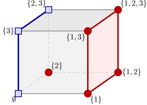
FIGURE 1. A 2-colouring of the subsets of \{1, 2, 3\} , drawn on the cube 2^3 . The five red sets (discs) form a union-closed family which is not a sublattice, since \{1\} \cap \{2\} = \emptyset is blue. The three blue sets (squares) form a chain.
