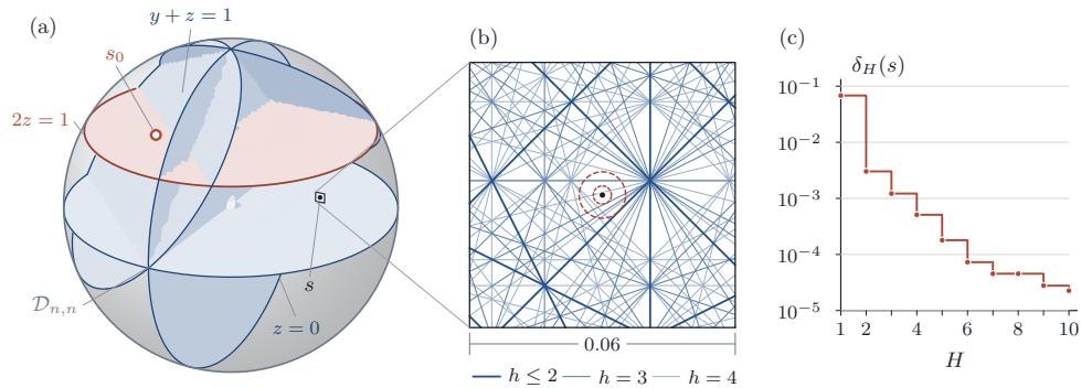
FIGURE 17. The dichotomy of Corollary 16.5. Each stratum \Sigma_{\underline{p}, \underline{q}} is Zariski closed by Theorem 16.4, and there are countably many of them; the base point s_0 of Theorem 15.27 lies on one. By Proposition 16.7 the union of the strata is dense, so every neighbourhood of a point s lying off all of them meets infinitely many strata. The conjecture for the family is the assertion that no such s exists, and by Corollary 16.5 it is enough that one stratum has nonempty interior.
