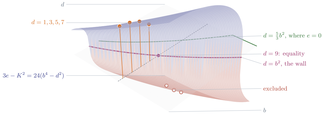
FIGURE 25. Theorem 14.159 over the quarter plane of (b, d) . The height of the surface is the defect 3e(S) - K_S^2 = 24(b^4 - d^2) in the Bogomolov–Miyaoka–Yau inequality for the surface the theorem attaches to the pair, compressed by a signed cube root so that four orders of magnitude fit one frame; the compression is odd and monotone, so the zero locus and the sign are the true ones. The surface is drawn indigo where the defect is positive and clay where it is negative, and it crosses zero along d = b^2 , which is therefore the whole content of the inequality. The weaker wall d = \frac{5}{3}b^2 , where e(S) itself changes sign, is drawn dashed and lies above it. On the line b = 3 , which is the value Proposition 14.144(iii) forces on the fourfold, the four squarefree discriminants d = 1, 3, 5, 7 with N an integer sit above the wall and are marked with their drop lines; d = 9 sits exactly on it, the equality case, and d = 11, 13, 15 sit below and are excluded.
