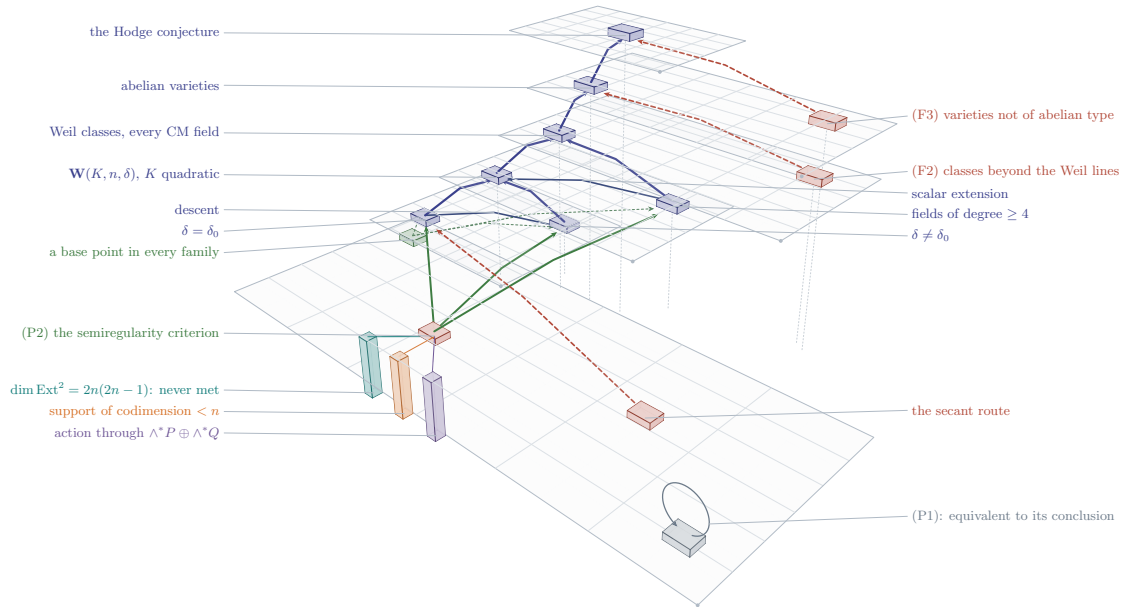
FIGURE 31. The route of this paper in Theorem 16.40 , drawn as a stack of plates, one per level of the derivation; the other routes of the literature are drawn in Figure 30 . The spine in indigo runs from the Weil families at the bottom to the conjecture at the top. The two statements (F2) and (F3) enter in clay from the right, each at the level where it is needed; (F2) is the conjecture for a class of Hodge classes that no Weil line reaches, not a reduction, and (F3) is the whole conjecture ( Proposition 16.35 ), so the route drawn is minimal only with (F3) replaced by (F3') of Definition 16.36 . From below, the propagation statement (P2) in grass reaches the two discriminant cases of the quadratic fields and the fields of higher degree alike, because Theorem 14.48 and Theorem 15.4 put a base point in every family; it is read in the corrected form of Remark 14.100 . The two edges inside the levels are Proposition 16.13 : descent from the trivial discriminant to the others, and scalar extension from the fields of degree at least four to the quadratic fields; with them (P2) is needed only for the split families of the fields of higher degree. The three pillars under the grass node are the results of Theorem 14.89 , Theorem 14.91 and Corollary 14.87 on the first form, in which the Chern character is exactly a Weil class; by Theorem 14.99 that form is never met, so the number on the first pillar is attained by no complex. The secant route in clay reaches the trivial discriminant, since the member it is built on is split, and through descent the rest of the quadratic case; it has no edge to the fields of higher degree. The bounded criterion (P1) is drawn apart, in slate, closed on itself: it is equivalent to its own conclusion.
