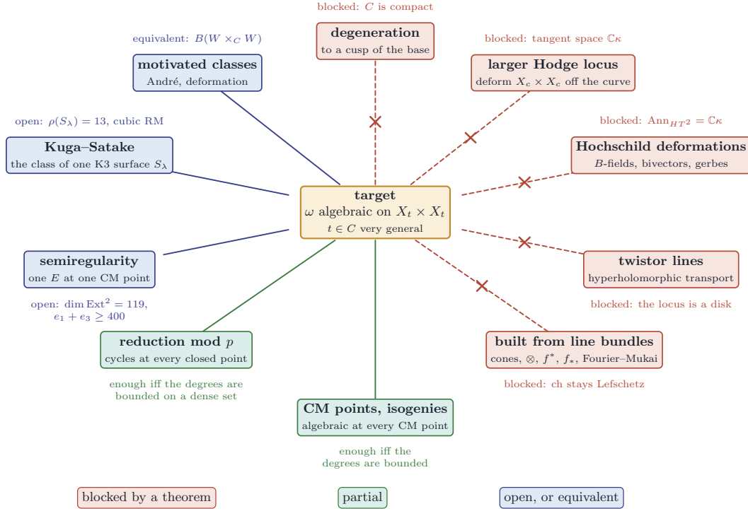
FIGURE 34. Remark 16.76: the ten routes to the Mumford target that avoid the Lefschetz standard conjecture. Clay, with a crossed dashed spoke: a route closed off by a theorem of Section 16.11 or Section 16.12 . Grass: a route that works at special points only, at the CM points or at the closed points of the reductions modulo p , and suffices exactly when a degree bound holds ( Corollary 16.75 , Theorem 16.85 ). Indigo: a route reduced to one open statement, of the same kind as the target or equivalent to it.
