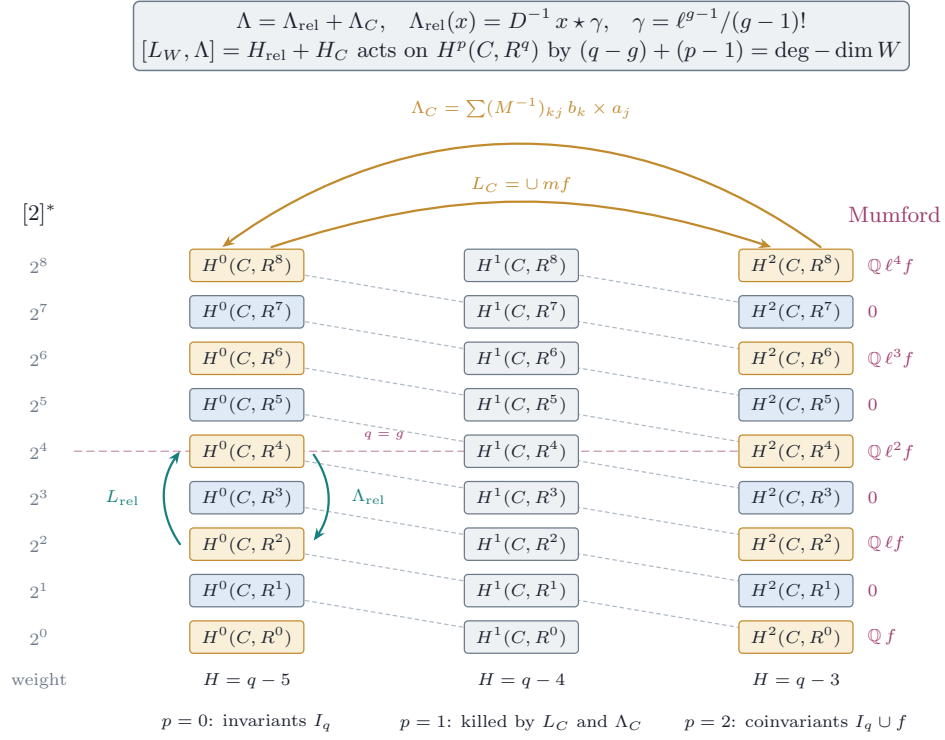
FIGURE 28. The proof of Theorem 16.22 for relative dimension four. The boxes are the summands H^p(C, R^q \pi_* \mathbb{Q}) of H^*(W, \mathbb{Q}) , split off by the eigenvalue 2^q of [2]^* shown on the left; the dotted diagonals join the summands of one H^k(W, \mathbb{Q}) , k = p + q , and the dashed magenta line is the axis q = g of hard Lefschetz on the fibres. The relative operators L_{\text{rel}} and \Lambda_{\text{rel}} , in teal, move within a column; \Lambda_{\text{rel}} is a Pontryagin product with an algebraic class on every abelian scheme ( Proposition 16.21 ). The base operators L_C and \Lambda_C , in ochre, move along a row between the outer columns and kill the middle one; \Lambda_C is the displayed cycle built from bases (a_j) , (b_k) of the invariant summands, and is algebraic exactly when the invariant cycles are. Below each column is the weight of H = [L_W, \Lambda] on it, and the panel at the top is Step 6 of the proof. The ochre boxes carry the invariant cycles and their images under L_C ; for a Mumford family they are the lines listed in magenta on the right, spanned by \ell^i f (and by \ell^i in the left column), and the other boxes of the outer columns are zero ( Corollary 16.23 ).
