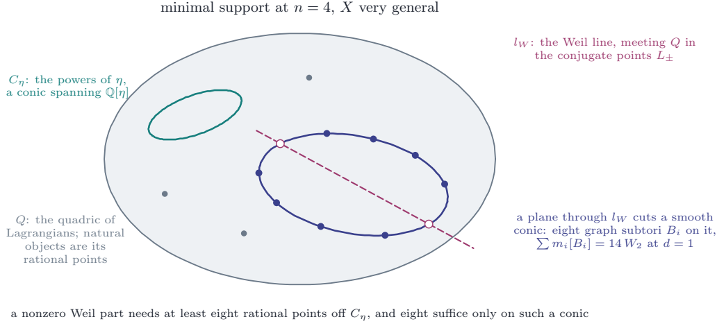
FIGURE 21. Theorem 14.117 . The quadric Q of Lagrangians; the rational points are the Chern characters of the natural objects on the split member at n = 4 , up to the Veronese map \nu_4 . The powers of the polarisation fill the conic C_\eta (teal), and the Weil line is spanned by the conjugate points L_\pm (open circles) in which the line l_W (dashed) meets Q . A combination of natural characters with a nonzero Weil part needs at least eight rational points off C_\eta , and with eight they lie on one conic cut out by a plane through l_W (indigo), such as the eight graph subvarieties B_i of Example 14.118 ; the grey points are natural objects off any such conic, which no relation of this size can use.
