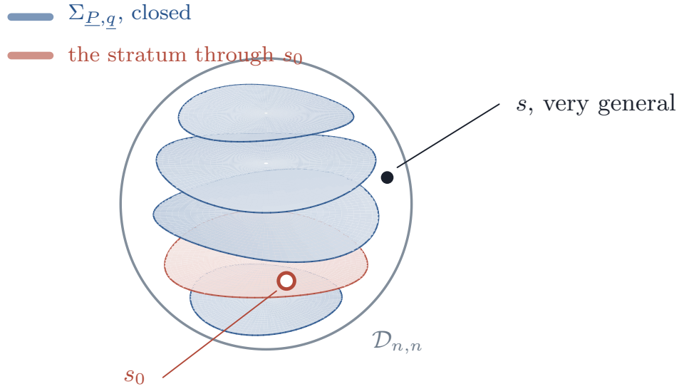
FIGURE 16. The dichotomy of Corollary 14.58 . Each stratum \Sigma_{\underline{p}, \underline{q}} is Zariski closed by Theorem 14.57 , and there are countably many of them; the base point s_0 of Theorem 14.48 lies on one. By Proposition 14.60 the union of the strata is dense, so a point s off all of them is squeezed between strata however small a neighbourhood is taken. The conjecture for the family is the assertion that no such s exists, and by Corollary 14.58 it is enough that one stratum has nonempty interior.
