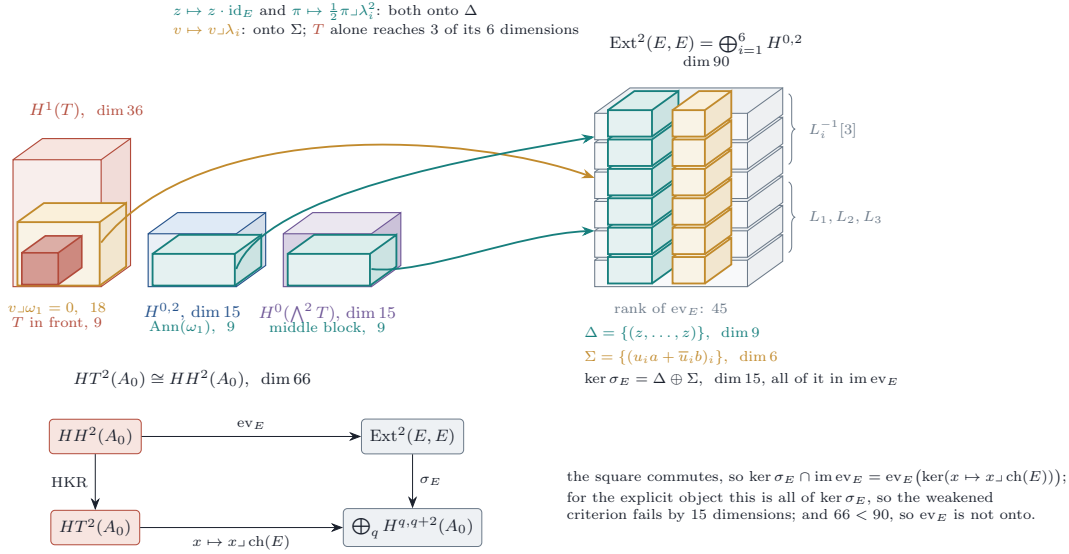
FIGURE 23. Proposition 18.18 for the explicit object at n = 3 . Left: the three summands of HT^2(A_0) , drawn with heights proportional to their dimensions, and inside each the part that preserves \text{ch}(E) to first order: the annihilator of \omega_1 , the deformations killing \omega_1 with the polarised K -commuting tangent space T in front, and the middle block of bivectors. Right: \text{Ext}^2(E, E) as six stacked copies of H^{0,2} , one per summand of E , and inside it the kernel of \sigma_E : the column \Delta , one and the same class in every layer, and the column \Sigma , whose entries depend on the summand through u_i . The three arrows are the evaluation map on the three kernels; the two teal ones both land on \Delta , the ochre one on \Sigma , and together they cover the kernel. Below, the commutative square that makes this a statement about the weakened criterion of [Mar25b, Question 11.4] .
