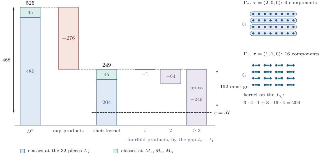
FIGURE 25. The 525 diagonal classes of degree two at n = 3 (Proposition 18.31 and Theorem 18.32). The cup products remove 276 of them for general components, and at most that many in any case, leaving 204 at the pieces L_\zeta and the 45 at the M_i ; when the t_i lie on one side of p , the fourfold products of the surviving path remove at most (t_2 - t_1)^6 more, which is 1 or 64 for the gaps 1 and 2 and no constraint from the third gap on. The criterion asks for 57, so 468 classes must disappear in all and 192 after the cup products. On the right, the graphs \Gamma_\tau on the 32 pieces, one row for each value of \zeta_1 : for \tau = (2, 0, 0) each row is a component, for \tau = (1, 1, 0) the components are the pairs differing in the sign of \zeta_3 ; a class constant on the components of every \Gamma_\tau has vanishing cup products.
