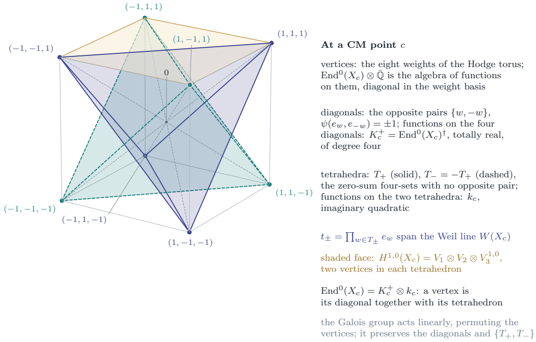
FIGURE 45. Proposition 21.29(i) . The eight weights (\pm 1, \pm 1, \pm 1) of the Hodge torus at a CM point are the vertices of a cube. The four diagonals are the pairs of opposite weights, paired by the polarisation; the two inscribed tetrahedra T_+ (an even number of entries -1 ) and T_- = -T_+ are the only zero-sum four-sets without an opposite pair, and t_{\pm} = \prod_{w \in T_{\pm}} e_w span the Weil line. The Galois group acts by linear maps permuting the vertices, so it preserves the diagonals and the pair of tetrahedra: the functions constant on the tetrahedra form the imaginary quadratic Weil field k_c , those constant on the diagonals the totally real quartic algebra K_c^+ of Rosati-fixed endomorphisms, and \text{End}^0(X_c) = K_c^+ \otimes k_c because a vertex is determined by its diagonal and its tetrahedron.
