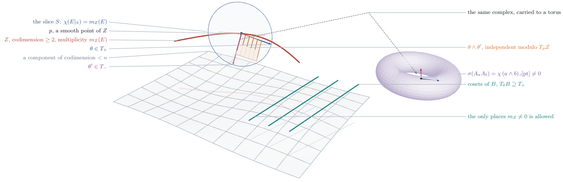
FIGURE 21. The proof of Theorem 16.39 . The grey sheet stands for a component of the support of codimension less than n , which the theorem forces to exist; the clay curve Z for a component of codimension at least two. At a smooth point p of Z the directions \theta \in T_+ and \theta' \in T_- span the slice S , transverse to Z , on which E restricts to a complex of finite length with Euler characteristic m_Z(E) ; the amber parallelogram is the bivector \theta \wedge \theta' , independent modulo T_p Z . Carried to a torus of the same dimension, the product of the two jet classes is seen by the semiregularity map as m_Z(E) times the class of a point contracted with the bivector, which is not zero, so m_Z(E) = 0 or the bivector degenerates. The teal lines are cosets of an abelian subvariety B tangent to T_+ , the only components of codimension at least two on which a nonzero multiplicity survives. The scene is schematic in the dimensions and exact in the incidences.
