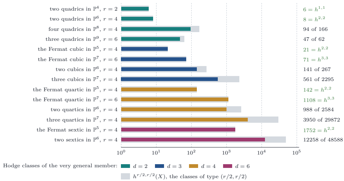
FIGURE 48. The dimension of the space of Hodge classes of degree r on the very general member, from Theorem 20.66(iii), against the Hodge number h^{r/2, r/2} , on a logarithmic scale. Where the two agree, the space H^{r/2, r/2} is spanned by Hodge classes at every configuration; elsewhere the very general member has fewer Hodge classes, and the members with more lie over a countable union of proper closed subsets of the space of configurations.
