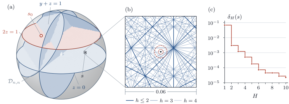
FIGURE 19. The dichotomy of Corollary 16.5. Each stratum \Sigma_{\underline{p},\underline{q}} is Zariski closed by Theorem 16.4, and there are countably many of them; the base point s_0 of Theorem 15.27 lies on one. By Proposition 16.7 the union of the strata is dense, so every neighbourhood of a point s lying off all of them meets infinitely many strata. The conjecture for the family is the assertion that no such s exists, and by Corollary 16.5 it is enough that one stratum has nonempty interior.
