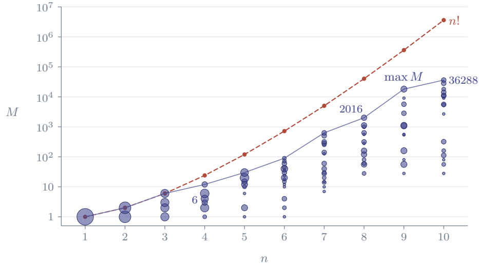
FIGURE 14. Remark 14.14. The least multiple M of Theorem 14.13 for 1 \leq n \leq 10 , over the seventy-two cases d \in \{1, 2, 3, 5, 7, 11\} , a \in \{1, 2, 3\} , b \in \{\pm 1, \pm 2\} for each n , read off from the solution of the Vandermonde system, on a logarithmic scale; the area of a disc counts the cases with that value. The solid line joins the largest values and the dashed one is n! , which every M divides by the remark: the quotient of \mathbb{Z}^{n+1} by the lattice of the characters (1, j, \dots, j^n) of the powers of a line bundle is dual to the integer-valued polynomials of degree at most n , spanned by the \binom{x}{k} , whose coefficients have denominators dividing n! .
