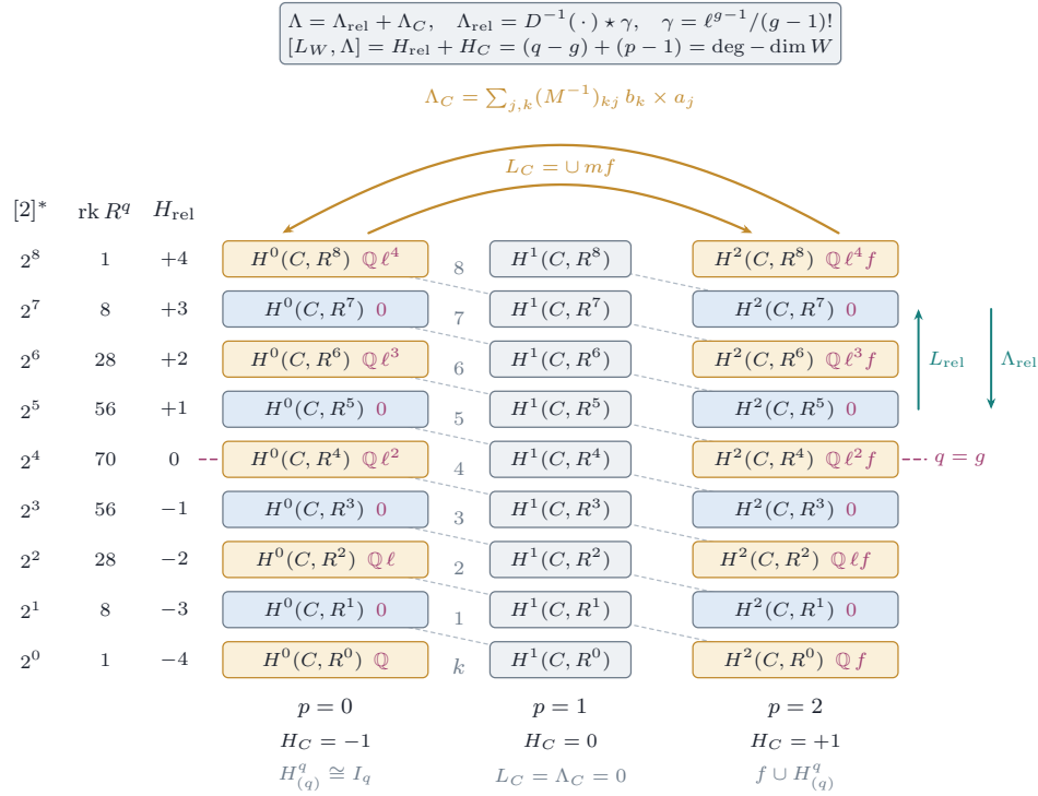
FIGURE 32. The proof of Theorem 20.22 for relative dimension four. The boxes are the summands H^p(C, R^q \pi_* \mathbb{Q}) of H^*(W, \mathbb{Q}) , split off by the eigenvalue 2^q of [2]^* shown on the left; the dotted diagonals join the summands of one H^k(W, \mathbb{Q}) , k = p + q , and the dashed magenta line is the axis q = g of hard Lefschetz on the fibres. The relative operators L_{\text{rel}} and \Lambda_{\text{rel}} , in teal, move within a column; \Lambda_{\text{rel}} is a Pontryagin product with an algebraic class on every abelian scheme ( Proposition 20.21 ). The base operators L_C and \Lambda_C , in ochre, move along a row between the outer columns and kill the middle one; \Lambda_C is the displayed cycle built from bases (a_j) , (b_k) of the invariant summands, and is algebraic exactly when the invariant cycles are. Below each column is the weight of H = [L_W, \Lambda] on it, and the panel at the top is Step 6 of the proof. The ochre boxes carry the invariant cycles and their images under L_C ; for a Mumford family they are the lines listed in magenta on the right, spanned by \ell^i f (and by \ell^i in the left column), and the other boxes of the outer columns are zero ( Corollary 20.23 ).
