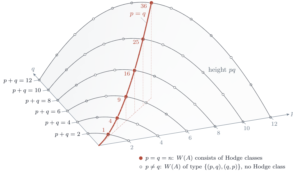
FIGURE 48. The signatures (p, q) of an imaginary quadratic action, with p + q = \dim A , drawn on the surface of height pq , which is the dimension of the family of abelian varieties carrying that action, the unitary Shimura variety of signature (p, q) . Each curve on the surface collects the signatures available in one dimension, and on it the diagonal point is the highest. The divisibility conditions of Theorem C.3 put no constraint on which of them occur when \text{End}^0(A) = K , by Proposition C.9(i) . By Proposition C.7 the Weil line consists of Hodge classes exactly at the filled points on the ridge p = q , and at every open point it is a rational sub-Hodge structure of type \{(p, 2n - p), (2n - p, p)\} carrying no Hodge class at all. The diagonal is the locus that Corollary B.9 shows to be an algebraic subvariety of the moduli.
