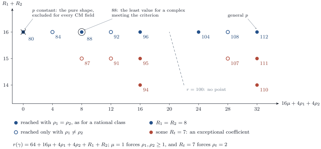
FIGURE 28. The rank r(\gamma) of Theorem 19.24, over the plane of the Hankel part 16\mu + 4\rho_1 + 4\rho_2 and of R_1 + R_2 . The fifteen points are the tuples allowed by the two conditions of the theorem, and each carries its value. Filled points are reached with \rho_1 = \rho_2 , as the character of a complex with rational coefficients is (Corollary 19.25(ii)); red points need an exceptional coefficient at one place at least. The value 80 is the pure shape, excluded for every CM field by Theorem 19.14; so 88 is the least rank a complex meeting the criterion can have. The level r = 100 meets no point.
