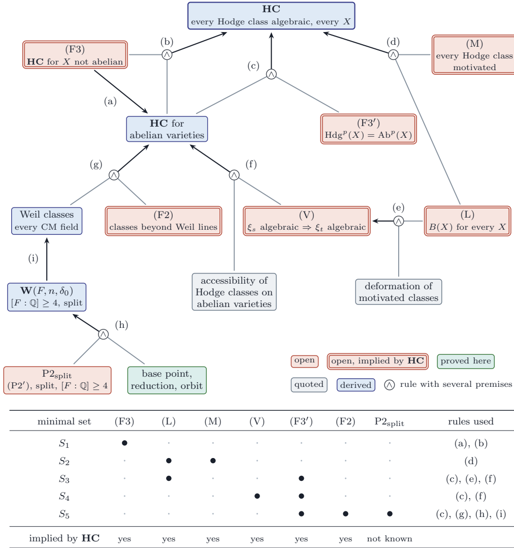
FIGURE 38. The rule set of Setup 20.57 with the rules of Section 20.6 , drawn as a hypergraph. A rule with several premises is a junction marked \wedge , joined to its premises and with one arrow to its conclusion. The letters name the results that prove the rules: (a) is Proposition 20.35 ; (b) and (g) are the closure map of Section 20.5 ; (c) is Proposition 20.37(i) ; (d) is Proposition 20.17 ; (e) is Proposition 20.18 ; (f) is Theorem 20.19 ; (h) is Theorem 19.7 ; and (i) is the chain of Proposition 20.13 , Proposition 20.12 , Proposition 19.3 and Appendix C . Clay marks a hypothesis, a double frame a hypothesis that the conjecture implies, grass what this paper proves, slate what it quotes, and indigo a derived statement. The table lists the five minimal sufficient sets of Theorem 20.58(ii) , the rules each of them uses, and which of the hypotheses the conjecture implies; only P2 split , which asks for a particular complex, is drawn without that frame. The secant route, which reaches the imaginary quadratic families only, is drawn in Figure 39 .
