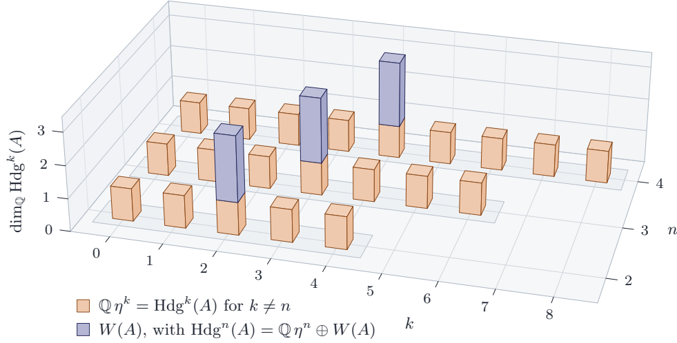
FIGURE 3. The dimensions of \text{Hdg}^k(A) for a general abelian variety of (K, -1, n) -Weil type, 0 \leq k \leq 2n , at n = 2, 3, 4 , as computed in Theorem 4.14 . Every degree carries the line \mathbb{Q}\eta^k ; the middle degree k = n carries in addition the two dimensions of the Weil line W(A) , and nothing else occurs. The profile is the same for every n .
