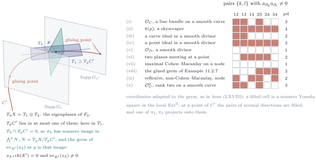
FIGURE 29. Theorem 19.39 and Corollary 19.41. Left: the support of Markman's sheaf E' near a point p of the glued curve C' , between two of the translated supports that the curve crosses at its gluing points. The tangent space at p is the sum of the eigenplanes T_1 and T_2 of the real multiplication; the tangent line of C' lies in at most one of them, here in T_1 , so \pi_2 has nonzero image in \wedge^2 N , N = T_p X / T_p C' , which is the germ of \text{ev}_{E'}(x_2) at p is that image: x_2 \lrcorner \text{ch}(E') = 0 and \text{ev}_{E'}(x_2) \neq 0 . Right: for ten germs at the origin of \mathbb{C}^4 , the pairs \{k, l\} of coordinate directions whose jet classes have nonzero product in the local \text{Ext}^2 , and the projective dimension; rows (i), (ii) and (x) are Lemma 19.37, row (iii) is Lemma 19.38, row (vi) is Lemma 18.33.
