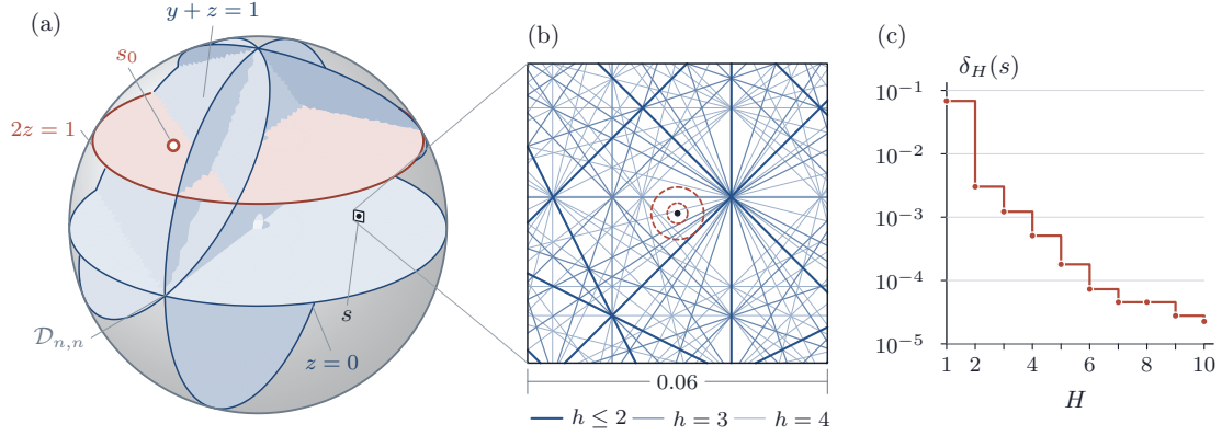
FIGURE 1. The algebraic locus of Theorem 1.1 , drawn over a real slice of the period domain \mathcal{D}_F . The explicit base point s_0 of part (i) lies on the stratum \Sigma_{\underline{P}, \underline{q}} of one tuple of Hilbert polynomials; the Hecke orbit G_F(\mathbb{Q}) \cdot s_0 is dense (part (ii)); and every stratum is closed and algebraic (part (iii)). The locus is the union of the strata. By part (iv) it is closed exactly when one stratum is the whole domain, and then the Hodge conjecture holds at every point off the countably many Noether–Lefschetz loci, one of which is shaded.
