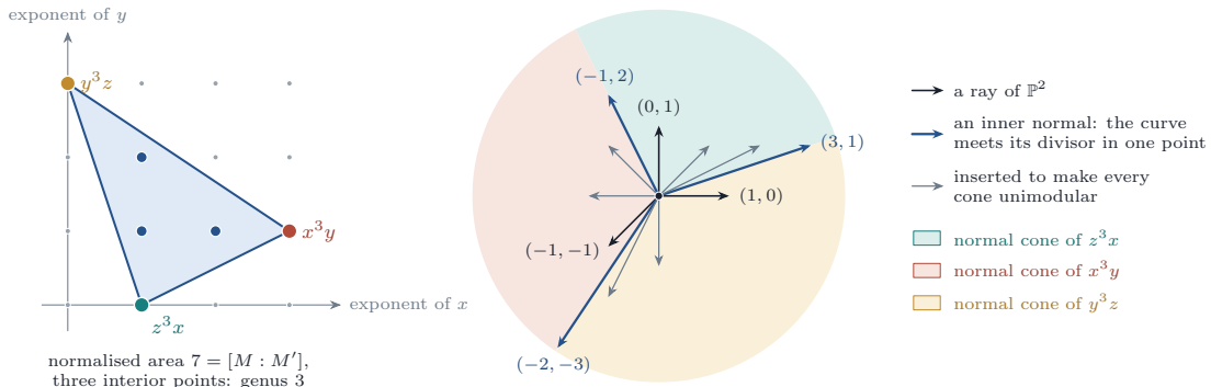
FIGURE 36. The Klein quartic x^3y + y^3z + z^3x in the proof of Theorem 20.53 . Left: its Newton triangle in the lattice M of the torus of \mathbb{P}^2 , in the chart z = 1 , with normalised area 7 = [M : M'] and three interior points, the genus. Right: the rays of a smooth fan adapted to it, the three rays of \mathbb{P}^2 , the three inner normals of the triangle and the six rays inserted to make every cone unimodular. The curve meets only the three divisors of the inner normals, in one point each, the lattice length of the edge, so its Euler number is -7 + 3 = -4 . With e_A = 7 the isogeny of the proof makes it the quotient of the Fermat septic by a group of order seven.
