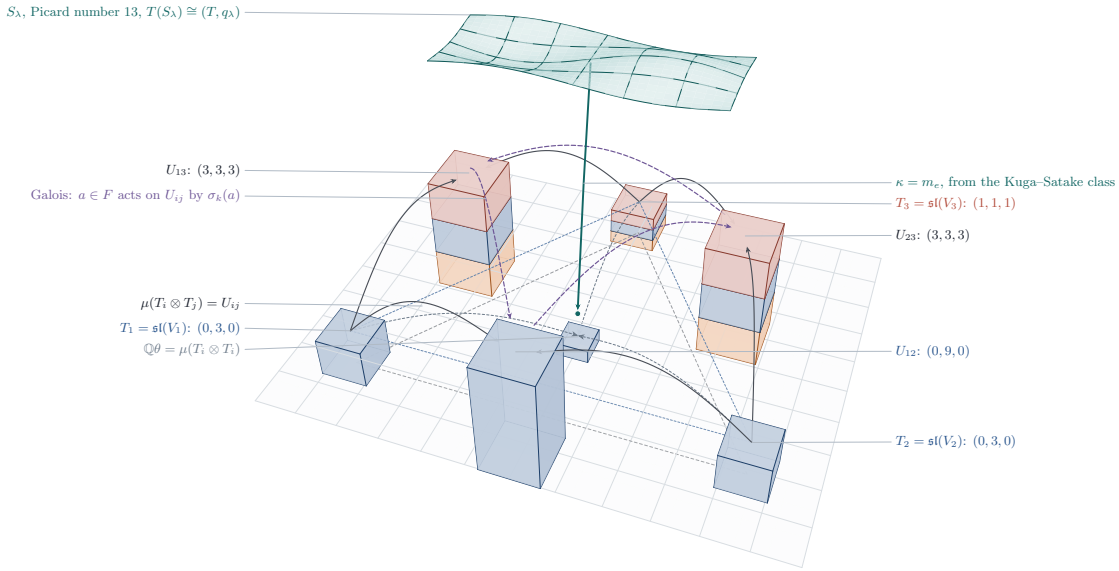
FIGURE 32. Proposition 21.2 and Lemma 21.3 , drawn over the triangle of the three factors of the Hodge group; every height is a dimension. At the corners stand the summands T_i = \mathfrak{sl}(V_i) of T = \text{Lie } G , banded by Hodge type after the Tate twist T(-1) : blue for (1, 1) , clay for (2, 0) and amber for (0, 2) , so that only T_3 carries the K3 type. On the edges stand the three summands U_{ij} of the primitive part of H^2(X) , of dimension nine, U_{12} of pure type (1, 1) and the other two in three bands of three; in the middle is the line of \theta . The solid arcs are the product map \mu , which carries T_i \otimes T_j onto U_{ij} , and the dashed ones carry T_i \otimes T_i to \mathbb{Q}\theta . The violet arcs are the Galois group permuting the U_{ij} as it permutes the embeddings of F , which is why the two exceptional classes may be taken to be the trace-zero part of a cubic field. Above, the K3 surface S_\lambda of Theorem 21.4 , whose Kuga–Satake class, if algebraic, comes down to T as the map \kappa = m_e .
