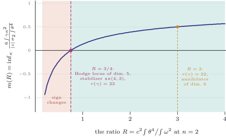
FIGURE 23. The exceptional ratio of Remark 17.12. By the identity displayed there, which is linear in \gamma , the infimum over the Kähler cone of 6 \int \gamma \kappa^2 / (|c| \sigma_2(h) \int \theta^4) is m(R) = 1 - \sqrt{3/(4R)} , approached at the boundary of the cone by a positive hermitian form of rank two whose Plücker coordinates satisfy |\xi_{01}\xi_{23}| = \frac{1}{4} . It is negative exactly for R < 3/4 , and R = 3/4 is also where the Hodge locus of \gamma jumps from dimension 4 to 5 and its stabiliser becomes \mathfrak{so}(4, 3) .
