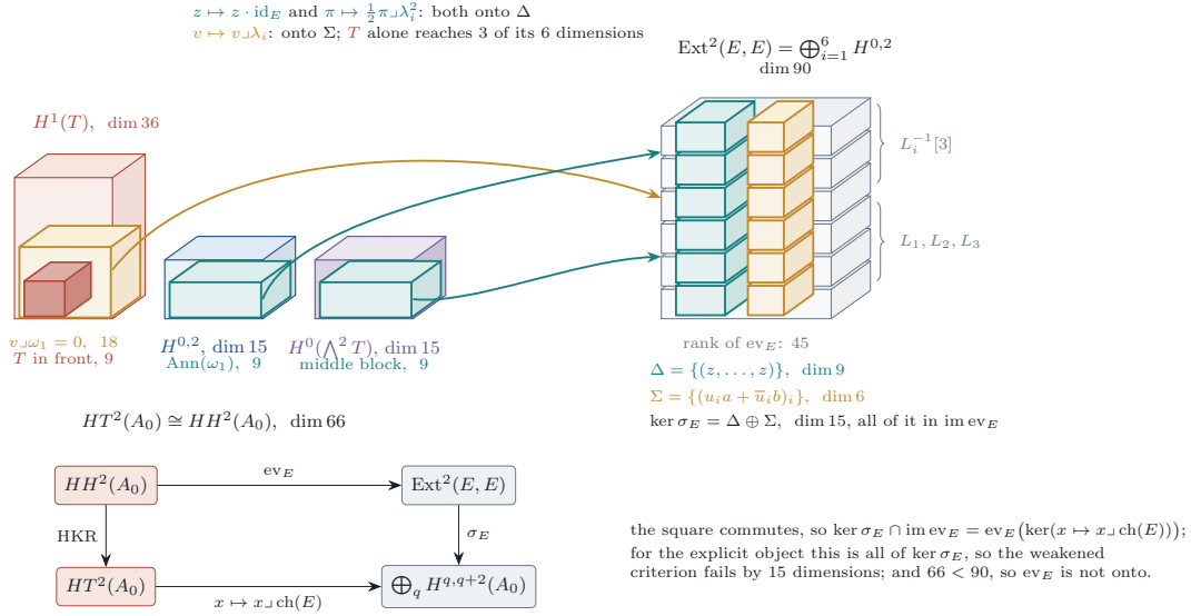
FIGURE 25. Proposition 18.18 for the explicit object at n = 3 . Left: the three summands of HT^2(A_0) , drawn with heights proportional to their dimensions, and inside each the part that preserves \text{ch}(E) to first order: the annihilator of \omega_1 , the deformations killing \omega_1 with the polarised K -commuting tangent space T in front, and the middle block of bivectors. Right: \text{Ext}^2(E, E) as six stacked copies of H^{0,2} , one per summand of E , and inside it the kernel of \sigma_E : the column \Delta , one and the same class in every layer, and the column \Sigma , whose entries depend on the summand through u_i . The three arrows are the evaluation map on the three kernels; the two teal ones both land on \Delta , the ochre one on \Sigma , and together they cover the kernel. Below, the commutative square that makes this a statement about the weakened criterion of [Mar25b, Question 11.4] .
