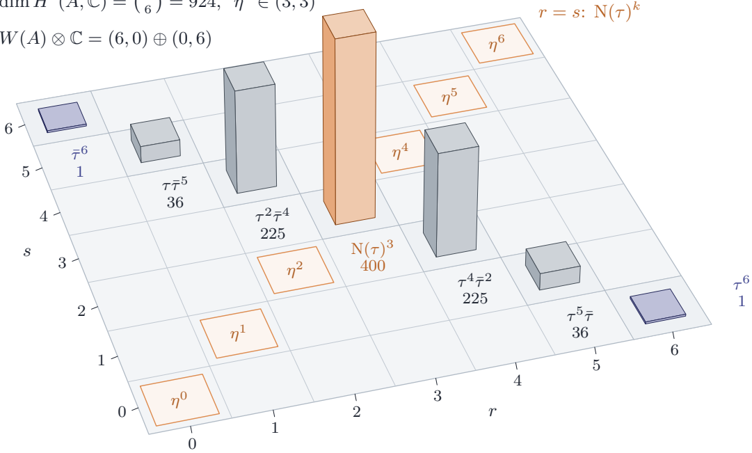
FIGURE 6. The K^\times -grading at n = 3 on the grid of pairs (r, s) , 0 \leq r, s \leq 6 . The summands \bigwedge^r V_+ \otimes \bigwedge^s V_- of H^6(A, \mathbb{C}) lie on the antidiagonal r + s = 6 and are drawn at their dimensions \binom{6}{r}\binom{6}{s} , which sum to \binom{12}{6} = 924 ; on the summand (r, s) the group K^\times acts by \tau^r \bar{\tau}^s . The two end cells (6, 0) and (0, 6) , with characters \tau^6 and \bar{\tau}^6 , span the Weil line; the middle cell (3, 3) , with character N(\tau)^3 , contains \eta^3 . The outlined cells on the diagonal r = s are the summands on which K^\times acts through a power of the norm, and they carry the powers \eta^k . That the end cells and the middle cell differ is the content of Theorem 5.6 .
