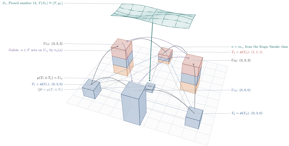
FIGURE 54. Proposition 21.2 and Lemma 21.3, drawn over the triangle of the three factors of the Hodge group; every height is a dimension. At the corners stand the summands T_i = \mathfrak{sl}(V_i) of T = \text{Lie } G , banded by Hodge type after the Tate twist T(-1) : blue for (1, 1) , clay for (2, 0) and amber for (0, 2) , so that only T_3 carries the K3 type. On the edges stand the three summands U_{ij} of the primitive part of H^2(X) , of dimension nine, U_{12} of pure type (1, 1) and the other two in three bands of three; in the middle is the line of \theta . The solid arcs are the product map \mu , which carries T_i \otimes T_j onto U_{ij} , and the dashed ones carry T_i \otimes T_i to \mathbb{Q}\theta . The violet arcs are the Galois group permuting the U_{ij} as it permutes the embeddings of F , which is why the two exceptional classes may be taken to be the trace-zero part of a cubic field. Above, the K3 surface S_\lambda of Theorem 21.4, whose Kuga–Satake class, if algebraic, comes down to T as the map \kappa = m_e .
