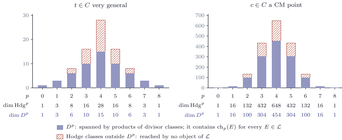
FIGURE 59. Theorem 21.36(ii). The Hodge classes of X_t \times X_t degree by degree, against the subring D^p generated by divisor classes, which contains the Chern character of every object of \mathcal{L} : at a very general point of the Mumford curve (left) and at a CM point (right). The hatched classes, the exceptional ones among them, are reached by no object of \mathcal{L} .
