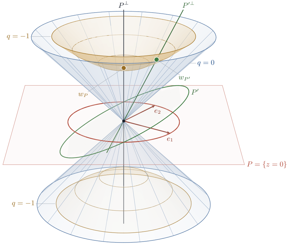
FIGURE 12. The geometry from which the Kuga–Satake construction starts, in the smallest case b = 3 . The quadratic form is q = x^2 + y^2 - z^2 , of signature (2, 1) , with its null cone q = 0 ; the horizontal plane P = \{z = 0\} is positive definite and meets the cone only at the origin. The construction needs such a plane, and Setup 11.1 supplies one: P = \langle \Re\sigma, \Im\sigma \rangle for the period \sigma spanning T^{2,0} . An orthonormal basis e_1, e_2 of P gives J = e_1 e_2 with J^2 = -1 by Lemma 11.4 , and J is the complex structure of \text{KS}(T) . A positive definite plane P is determined by the negative line P^\perp , which meets the upper sheet of the hyperboloid q = -1 in one point w_P ; that sheet is the period domain, and a second plane P' with its point w_{P'} is drawn for comparison. The hypothesis behind all of this is \dim T^{2,0} = 1 , and by Proposition 11.11 an abelian variety of Weil type with Hodge group \text{SU}(V, H) supplies it in H^2 only when n = 1 , or n = 2 at trivial discriminant.
