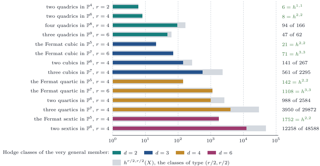
FIGURE 48. The dimension of the space of Hodge classes of degree r on the very general member, from Theorem 20.66(iii) , against the Hodge number h^{r/2, r/2} , on a logarithmic scale. Where the two agree, the space H^{r/2, r/2} is spanned by Hodge classes at every configuration; elsewhere the very general member has fewer Hodge classes, and the members with more lie over a countable union of proper closed subsets of the space of configurations.
