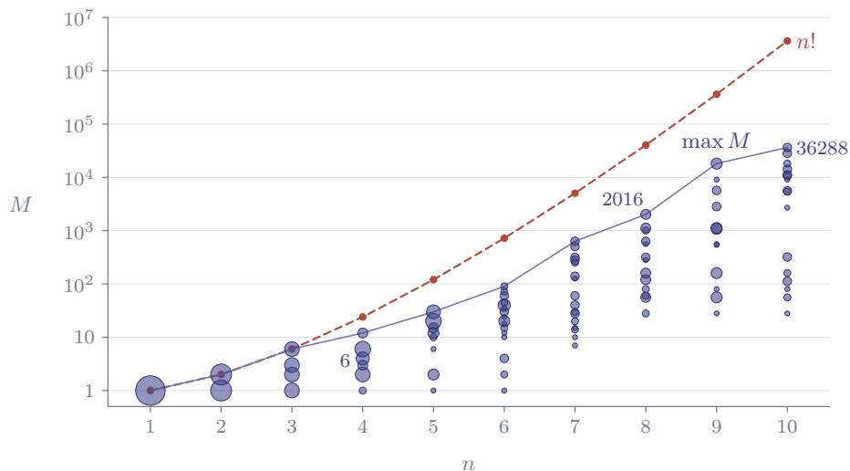
FIGURE 14. Remark 14.14 . The least multiple M of Theorem 14.13 for 1 \leq n \leq 10 , over the seventy-two cases d \in \{1, 2, 3, 5, 7, 11\} , a \in \{1, 2, 3\} , b \in \{\pm 1, \pm 2\} for each n , read off from the solution of the Vandermonde system, on a logarithmic scale; the area of a disc counts the cases with that value. The solid line joins the largest values and the dashed one is n! , which every M divides by the remark: the quotient of \mathbb{Z}^{n+1} by the lattice of the characters (1, j, \dots, j^n) of the powers of a line bundle is dual to the integer-valued polynomials of degree at most n , spanned by the \binom{x}{k} , whose coefficients have denominators dividing n! .
