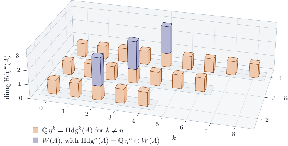
FIGURE 4. The dimensions of \text{Hdg}^k(A) for a general abelian variety of (K, -1, n) -Weil type, 0 \leq k \leq 2n , at n = 2, 3, 4 , as computed in Theorem 4.14 . Every degree carries the line \mathbb{Q}\eta^k ; the middle degree k = n carries in addition the two dimensions of the Weil line W(A) , and nothing else occurs. The profile is the same for every n .
