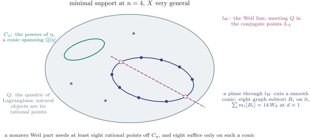
FIGURE 24. Theorem 17.27. The quadric Q of Lagrangians; the rational points are the Chern characters of the natural objects on the split member at n = 4 , up to the Veronese map \nu_4 . The powers of the polarisation fill the conic C_\eta (teal), and the Weil line is spanned by the conjugate points L_\pm (open circles) in which the line l_W (dashed) meets Q . A combination of natural characters with a nonzero Weil part needs at least eight rational points off C_\eta , and with eight they lie on one conic cut out by a plane through l_W (indigo), such as the eight graph subvarieties B_i of Example 17.28 ; the grey points are natural objects off any such conic, which no relation of this size can use.
