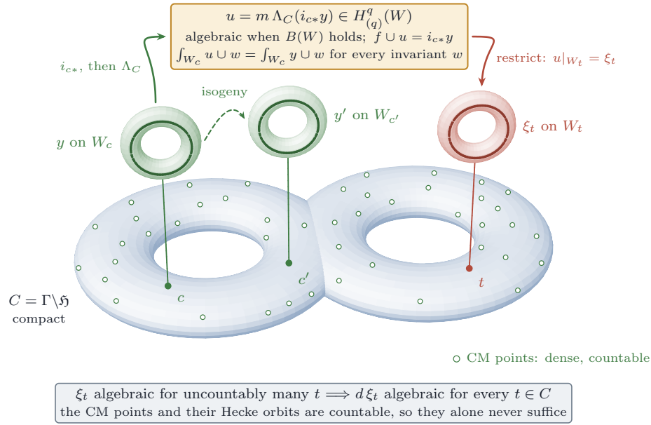
FIGURE 41. Theorem 20.28(ii) along a compact Shimura curve C . An algebraic class y on one fibre, at a base point of a Weil family or at a CM point of a Mumford family (hollow dots: the CM points, countable and dense), is pushed into W by the Gysin map and brought back to the invariant summand by the base operator \Lambda_C . When B(W) holds the result u is an algebraic class on W , pinned down by the displayed pairing against the invariant classes, and its restriction to a very general fibre is the invariant part of y . The dashed arcs are isogenies between CM members along Hecke orbits: they carry algebraic classes to algebraic classes but reach only countably many points, and Lemma 20.27 , in the box, needs uncountably many. This is how Corollary 20.31 and Corollary 20.30 turn each target into one case of (L).
