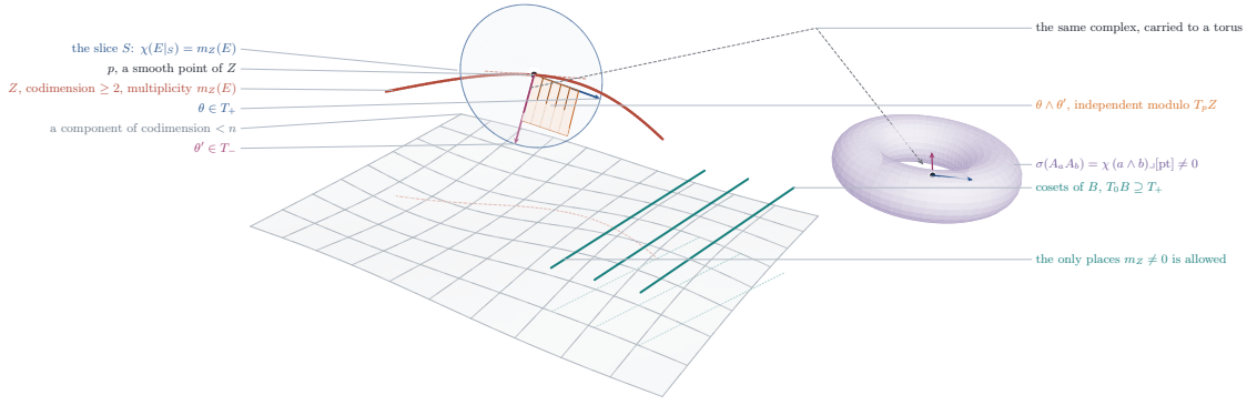
FIGURE 21. The proof of Theorem 16.39 . The grey sheet stands for a component of the support of codimension less than n , which the theorem forces to exist; the clay curve Z for a component of codimension at least two. At a smooth point p of Z the directions \theta \in T_+ and \theta' \in T_- span the slice S , transverse to Z , on which E restricts to a complex of finite length with Euler characteristic m_Z(E) ; the amber parallelogram is the bivector \theta \wedge \theta' , independent modulo T_p Z . Carried to a torus of the same dimension, the product of the two jet classes is seen by the semiregularity map as m_Z(E) times the class of a point contracted with the bivector, which is not zero, so m_Z(E) = 0 or the bivector degenerates. The teal lines are cosets of an abelian subvariety B tangent to T_+ , the only components of codimension at least two on which a nonzero multiplicity survives. The scene is schematic in the dimensions and exact in the incidences.
