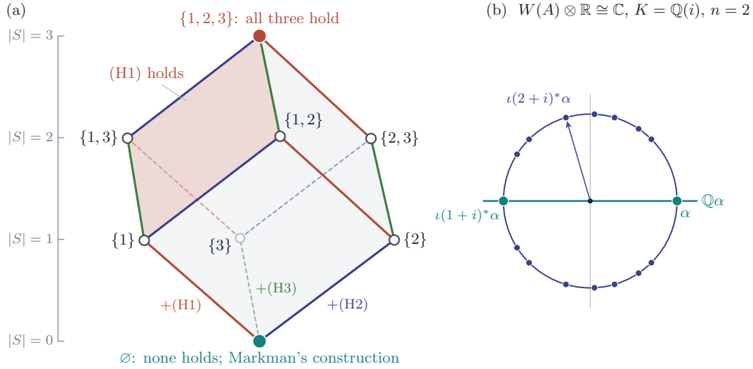
FIGURE 13. (a) The eight positions a construction can occupy, drawn as the Boolean lattice of the subsets S of three hypotheses: (H1) the Chern character of the input lies in the subring generated by divisor classes; (H2) the output is a K^\times -eigenclass; (H3) the output spans a single line rather than a plane. (H1) and (H2) are the hypotheses negated in (i) and (iii) of Proposition 13.5, and (H3) is what Corollary 13.2 excludes for a nonzero Weil class. At the top vertex all three hold, and both Theorem 7.3 and Theorem 5.6 apply; on the shaded face (H1) holds, and Theorem 7.3 alone already applies. Markman's construction sits at the bottom vertex, where none of the three holds. (b) The orbit of a Weil class \alpha under K^\times for K = \mathbb{Q}(i) and n = 2 , in W(A) \otimes \mathbb{R} \cong \mathbb{C} and normalised to the unit circle. Since \iota(\tau)^* acts through \tau^4 , the class \iota(1+i)^*\alpha = -4\alpha stays on the line \mathbb{Q}\alpha , while \iota(2+i)^*\alpha , with (2+i)^4 = -7 + 24i , does not; the orbit spans the plane, as Proposition 13.1 asserts.
