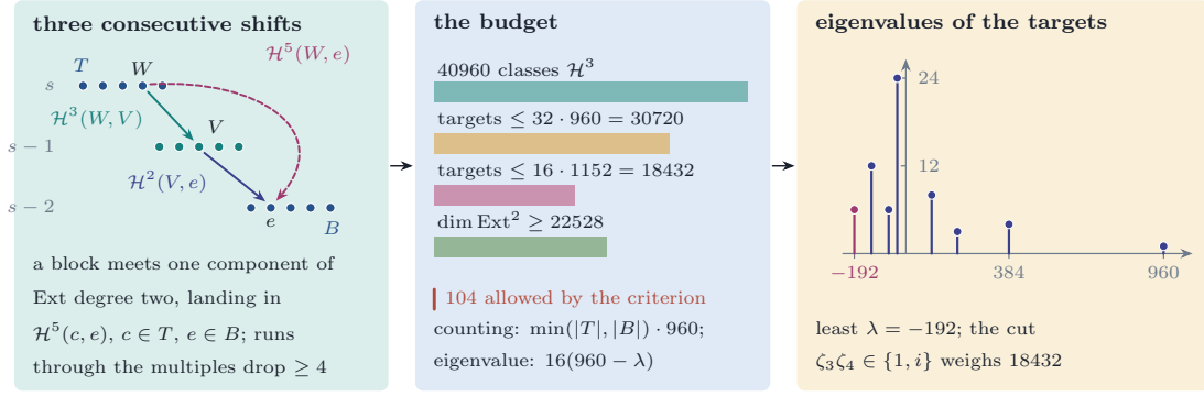
FIGURE 29. Theorem 18.38 . Left: the pieces L_\zeta at three consecutive shifts, those of one parity at s - 1 and the others split between T at s and B at s - 2 ; a group \mathcal{H}^3 between two pieces that differ in three coordinates (teal) can meet a component of Ext degree two (indigo) only in a group \mathcal{H}^5(c, e) with c \in T and e \in B (magenta). Middle: the 40960 classes against the targets, at most 30720 by counting and 18432 by the least eigenvalue, against the 104 that the criterion allows. Right: the eigenvalues of the Cayley graph of the targets.
