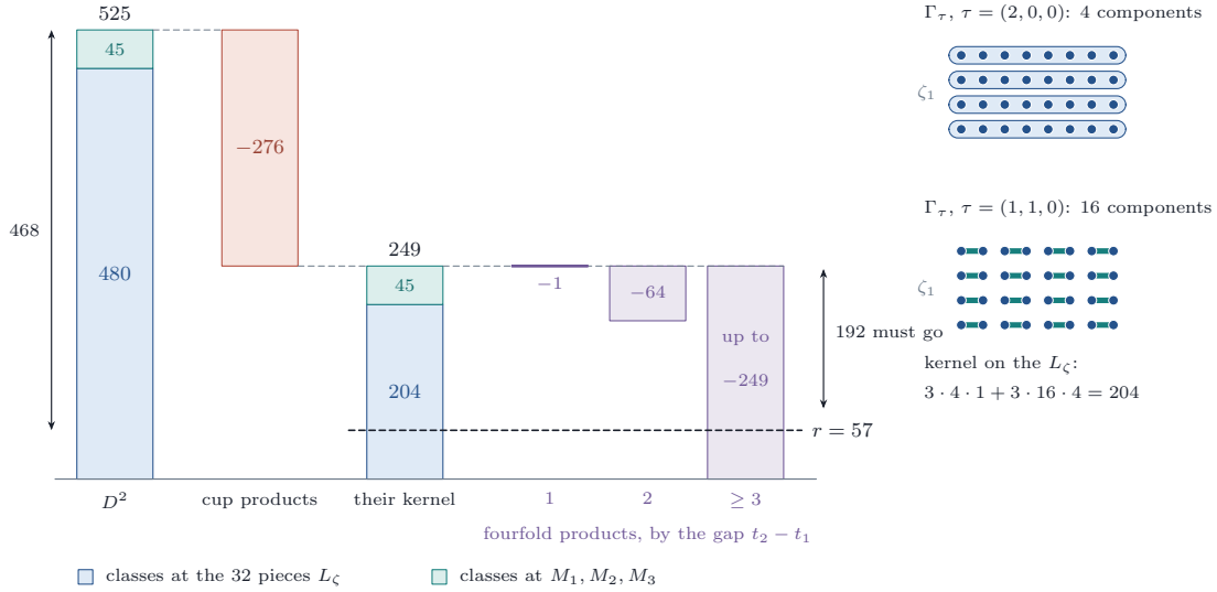
FIGURE 27. The 525 diagonal classes of degree two at n = 3 (Proposition 18.30 and Theorem 18.31). The cup products remove 276 of them for general components, and at most that many in any case, leaving 204 at the pieces L_\zeta and the 45 at the M_i ; when the t_i lie on one side of p , the fourfold products of the surviving path remove at most (t_2 - t_1)^6 more, which is 1 or 64 for the gaps 1 and 2 and no constraint from the third gap on. The criterion asks for 57, so 468 classes must disappear in all and 192 after the cup products. On the right, the graphs \Gamma_\tau on the 32 pieces, one row for each value of \zeta_1 : for \tau = (2, 0, 0) each row is a component, for \tau = (1, 1, 0) the components are the pairs differing in the sign of \zeta_3 ; a class constant on the components of every \Gamma_\tau has vanishing cup products.
