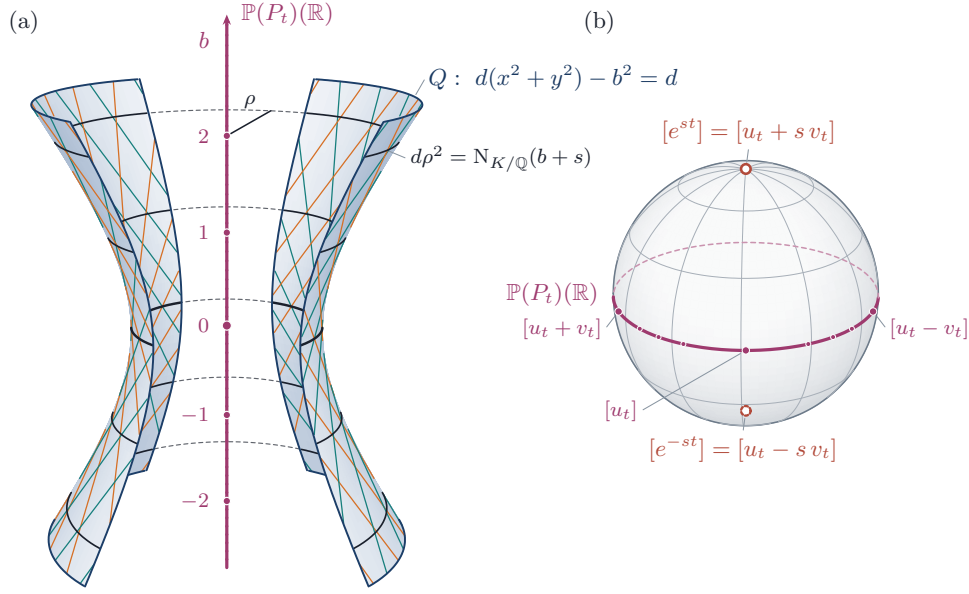
FIGURE 16. The geometry of Theorem 14.5 in the first case, n = 2 . The even spinor variety is then the smooth six-dimensional quadric of classes isotropic for the Mukai pairing in \mathbb{P}(H^{\text{ev}}(X, \mathbb{C})) \cong \mathbb{P}^7 , and the figure shows a real two-dimensional section of it, a quadric surface with its two rulings. The line \mathbb{P}(P_t) of Definition 14.4 is defined over \mathbb{Q} and meets the quadric only in the two points [e^{\pm st}] , which are conjugate over K and not individually rational; they are drawn as real points. This is the configuration the Weil line demands: a class defined over \mathbb{Q} cannot single out one of the two points, so the construction must carry the pair, and the pair spans a plane rather than a line. Proposition 13.1 is the same statement on the cohomological side, and Figure 13 places it among the hypotheses a construction can satisfy.
