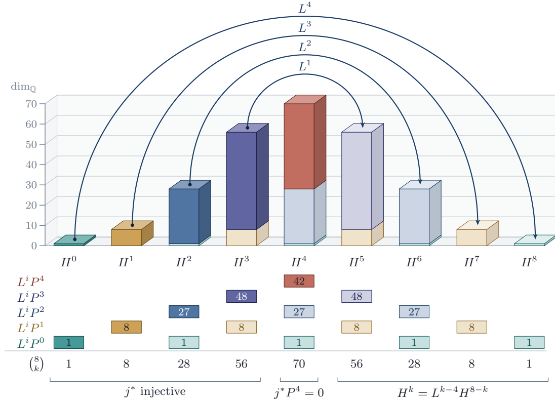
FIGURE 11. The Betti numbers \binom{8}{k} of an abelian fourfold, drawn as prisms and divided according to the Lefschetz decomposition H^k = \bigoplus_i L^i P^{k-2i} : the primitive part P^k is drawn dark, and each image L^i P^{k-2i} is drawn light in the colour of P^{k-2i} . The arcs are the hard Lefschetz isomorphisms L^{4-k}: H^k \rightarrow H^{8-k} . Below the middle degree the restriction j^* to a smooth ample hypersurface is injective and a class descends, but the return trip j_* j^* multiplies by L , and recovering the class is the Lefschetz standard conjecture; above the middle degree a class is carried to the lower half by an arc. The primitive middle cohomology P^4 , of dimension 70 - 28 = 42 , is annihilated by j^* (Theorem 10.3), and neither an arc nor a restriction reaches it.
