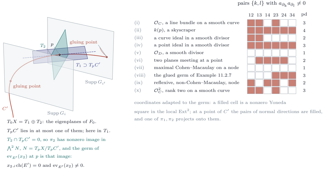
FIGURE 38. Theorem 19.43 and Corollary 19.45 . Left: the support of Markman's sheaf E' near a point p of the glued curve C' , between two of the translated supports that the curve crosses at its gluing points. The tangent space at p is the sum of the eigenplanes T_1 and T_2 of the real multiplication; the tangent line of C' lies in at most one of them, here in T_1 , so \pi_2 has nonzero image in \wedge^2 N , N = T_p X / T_p C' , which is the germ of \text{ev}_{E'}(x_2) at p . Right: for ten germs at the origin of \mathbb{C}^4 , the pairs \{k, l\} of coordinate directions whose jet classes have nonzero product in the local \text{Ext}^2 , and the projective dimension; rows (i), (ii) and (x) are Lemma 19.41 , row (iii) is Lemma 19.42 , row (vi) is Lemma 18.60 .
