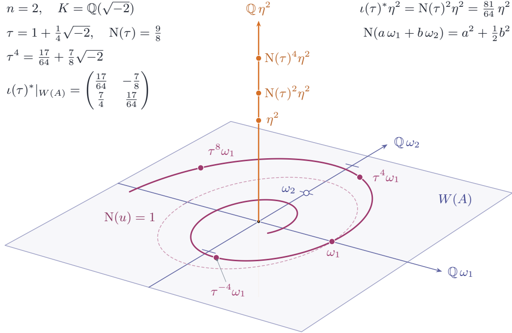
FIGURE 7. The linear algebra behind Theorem 7.3 , drawn inside H^{2n}(A, \mathbb{Q}) . The Weil line W(A) is a plane, free of rank one over K and of rank two over \mathbb{Q} , and K^\times acts on it through \tau^{2n} , so the orbit of any nonzero class is a spiral that spans the plane and lies on no line in it. The transverse axis carries \eta^n , on which K^\times acts through the norm. A construction returning a single eigenclass returns a line, and by Proposition 13.1 no line inside W(A) is stable.
