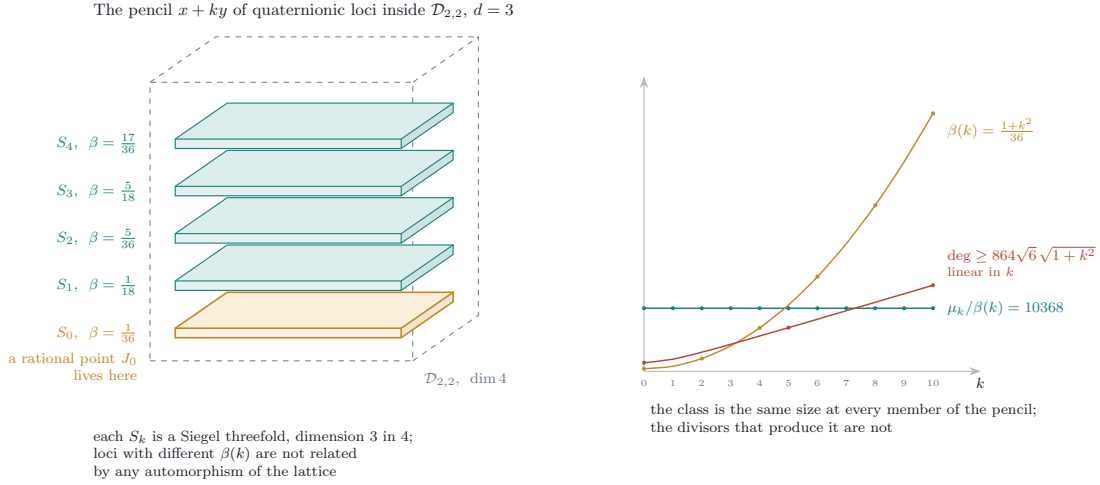
FIGURE 20. Proposition 16.25 at d = 3 . Left: the members S_k of the pencil, each a Siegel threefold inside the four-dimensional family, with the member k = 0 , where \beta = \frac{1}{36} is a square and a rational point J_0 can be written down, drawn apart. Right: along the pencil the ratio \mu_k/\beta(k) is the constant 10368 = \int \eta^4/3 , so \mu_k grows like k^2 and the least degree of a divisor not proportional to \eta grows linearly in k . The Weil class is a flat class of the one fixed lattice and does not change; the divisors that produce it must.
