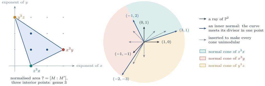
FIGURE 44. The Klein quartic x^3y + y^3z + z^3x in the proof of Theorem 20.52 . Left: its Newton triangle in the lattice M of the torus of \mathbb{P}^2 , in the chart z = 1 , with normalised area 7 = [M : M'] and three interior points, the genus. Right: the rays of a smooth fan adapted to it, the three rays of \mathbb{P}^2 , the three inner normals of the triangle and the six rays inserted to make every cone unimodular. The curve meets only the three divisors of the inner normals, in one point each, the lattice length of the edge, so its Euler number is -7 + 3 = -4 . With e_A = 7 the isogeny of the proof makes it the quotient of the Fermat septic by a group of order seven.
