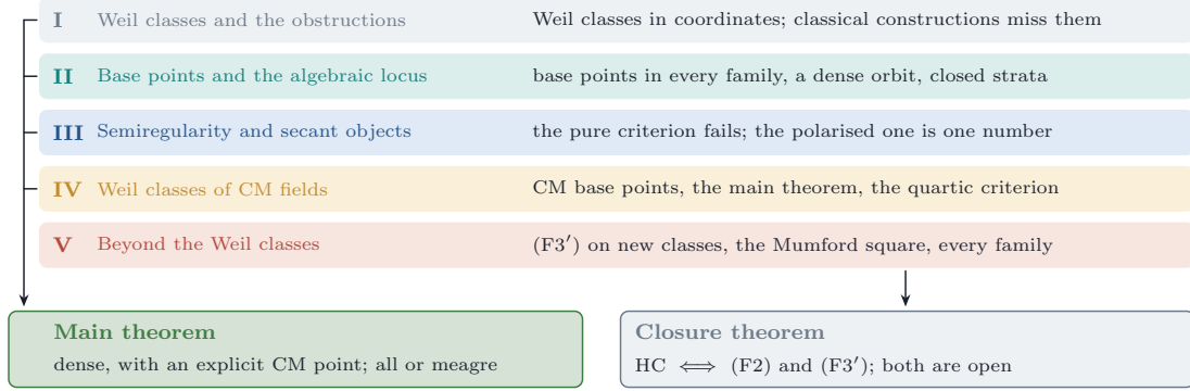
FIGURE 1. The five parts of the paper. Parts I to IV lead to Theorem 1.1 ; all five lead to the closure theorem of Section 23 , by which the Hodge conjecture is equivalent to the two statements (F2) and (F3'), both of which remain open.
