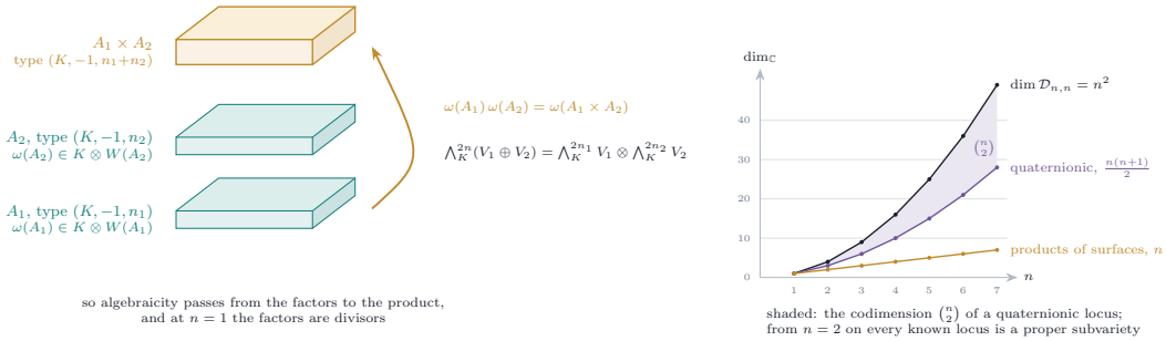
FIGURE 17. Theorem 15.7 and its reach. Left: the Weil line of each factor is a K -line, the Weil line of the product is the tensor product of the two over K , and the K -valued Weil class is multiplicative. Algebraicity therefore passes from the factors to the product, and at n = 1 the factors are divisor classes, so a product of n abelian surfaces of Weil type carries an explicit algebraic Weil class in every dimension. Right: the dimensions of the loci on which the class is known to be algebraic, against the dimension n^2 of the family. Both the quaternionic locus and the product locus are proper subvarieties once n \geq 2 , and a general member lies on neither.
