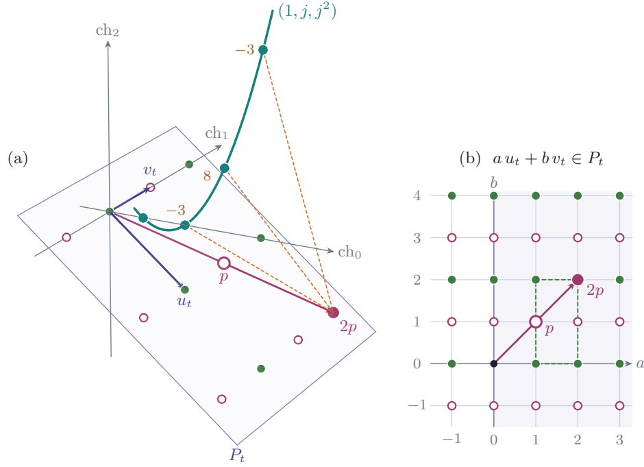
FIGURE 15. Theorem 14.13 at n = 2 and d = 2 . (a) The coordinates (ch_0, ch_1, ch_2) in the basis 1, t, t^2/2 . The Chern characters of the powers of one line bundle lie on the moment curve j \mapsto (1, j, j^2) , and the Vandermonde determinant says that any three of its points are affinely independent. The integral points of P_t = \mathbb{Q}u_t \oplus \mathbb{Q}v_t split by the criterion ch_2 \equiv ch_1 \pmod{2} into those reached by integer combinations of line bundles, drawn filled, and those missed, drawn open. The point p = u_t + v_t is missed and 2p is reached, by the witness -3[\mathcal{O}_X] + 8[\mathcal{O}_X(t)] - 3[\mathcal{O}_X(2t)] , whose three terms are joined to 2p by dashed segments. (b) The same points in the coordinates (a, b) of au_t + bv_t \in P_t . Here ch_1 = b and ch_2 = -2a , so the criterion reads b \equiv 0 \pmod{2} ; the shaded half-plane a > 0 is the range of Theorem 14.13 .
