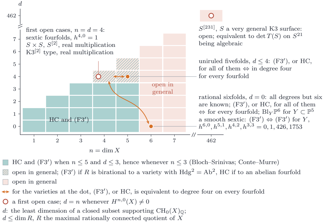
FIGURE 50. What arguments on zero-cycles and on rationally connected fibrations give for (F3') and for the Hodge conjecture (HC in the figure) on a variety X , over the plane of n = \dim X and the least dimension d of a closed subset supporting \text{CH}_0(X)_{\mathbb{Q}} ; d is at most the dimension of the maximal rationally connected quotient R of X , and d = n whenever H^{n,0}(X) \neq 0 (Remark 20.45). Both hold when n \leq 5 and d \leq 3 (Proposition 20.43), hence on every variety of dimension at most three. In the hatched cells (F3') holds when R is birational to a variety with \text{Hdg}^2 = \text{Ab}^2 , for instance a member of \mathcal{A} , and the Hodge conjecture when R is birational to an abelian fourfold (Proposition 20.44). The double arrows are the equivalences of Remark 20.45: (F3'), and the Hodge conjecture, hold for every uniruled fivefold, and for every rational sixfold, if and only if they hold in degree four for every fourfold; the sixfold \text{Bly } \mathbb{P}^6 of a smooth sextic fourfold Y in a hyperplane carries the Hodge numbers listed. The rings are the frontier cases (Remark 20.68): the sextic fourfolds, the first family of smooth hypersurfaces beyond these results (the 29 Delsarte sextics lie in \mathcal{A} by Corollary 20.53); S \times S and S^{[2]} for a K3 surface S with real multiplication, such as S_{\lambda} ; the fourfolds of K3^{[2]} type with real multiplication, among them F(Y) ; and, beyond the breaks of the axes, S^{[231]} for a very general K3 surface, which is equivalent to the algebraicity of \det T(S) on S^{21} (Proposition 20.39, Figure 42).
