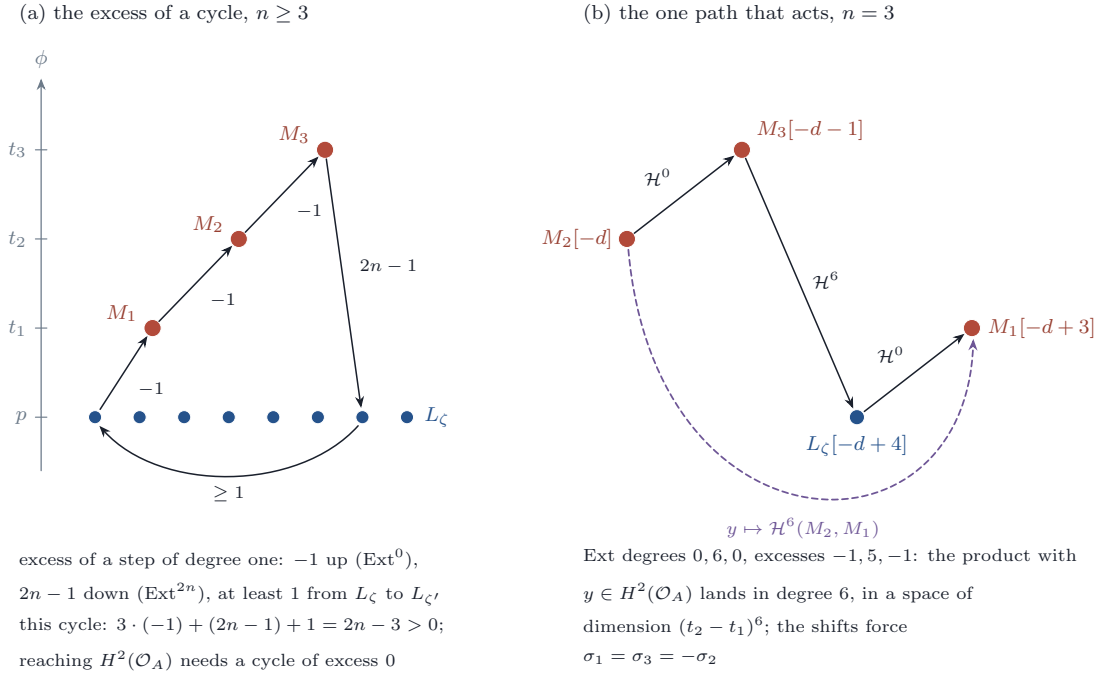
FIGURE 26. The pieces of Proposition 18.27 at their values \phi , with \phi(L_\zeta) = p and \phi(M_i) = t_i . (a) A step of degree one between pieces with a definite difference has Ext degree 0 going up and 2n going down, so excess -1 or 2n-1 ; a step between two L_\zeta has excess at least 1. The cycle drawn runs up through all three M_i and down once, the worst case, and still has excess 2n-3 > 0 , so for n \geq 3 no term reaches the diagonal ( Proposition 18.29 ). (b) The one path whose products act on the diagonal at n = 3 when the t_i lie above p ( Theorem 18.31(i) ), drawn at the same heights and in the order of the convolution, with the Ext degrees of its steps and the shifts they force; the dashed arrow is the value of the product with a diagonal class y .
