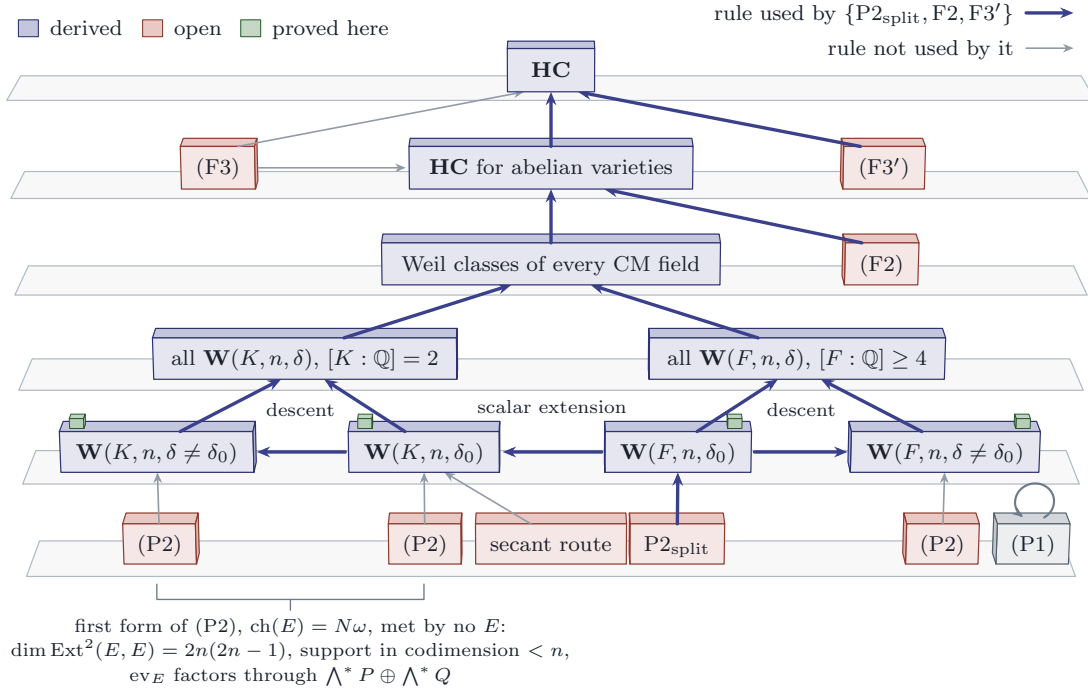
FIGURE 52. The route of this paper through the rule set of Theorem 20.70 , drawn as a stack of plates, one per level of the derivation; the other routes are drawn in Figure 51 . Heavy arrows are the rules used by the minimal set \{P2_{\text{split}}, F2, F3'\} , light arrows the rules it does not use. The bottom plate carries the propagation statement, read in the polarised form of Remark 17.6 , once for each of the four kinds of Weil family, with the secant route beside it. The small grass blocks on the next plate are the base points of Theorem 15.27 and Theorem 19.5 , one in every family. The three arrows inside that plate are Proposition 20.13 : descent from the trivial discriminant to the others, and scalar extension from the fields of degree at least four to the quadratic fields. With them (P2) is needed only for the split families of the fields of higher degree, and the other three (P2) blocks are not used. (F2) is the conjecture for the Hodge classes that no Weil line reaches, and (F3) is the whole conjecture ( Proposition 20.33 ), so the route is minimal only with (F3) replaced by (F3') of Definition 20.34 . The bracket under the two quadratic (P2) blocks records the first form of the criterion, in which the Chern character is exactly a Weil class, as Theorem 16.37 , Theorem 16.39 and Corollary 16.35 describe it; by Theorem 17.5 that form is met by no complex. The secant route reaches the trivial discriminant, since the member it is built on is split, and through descent the rest of the quadratic case; it has no edge to the fields of higher degree. The bounded criterion (P1) stands apart, closed on itself: it is equivalent to its own conclusion.
