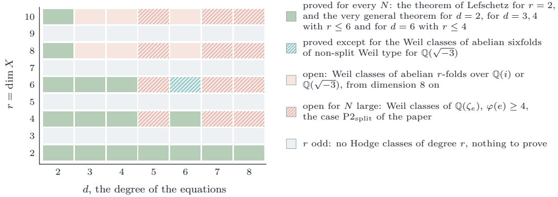
FIGURE 49. The Hodge conjecture for the very general complete intersection X_{d,r}(\lambda) of Vandermonde type, for every N . Grass: proved, by the theorem of Lefschetz for r = 2 and by Theorem 20.66 for d = 2 , for d = 3, 4 with r \leq 6 and for d = 6 with r \leq 4 . Teal hatching: proved except for the Weil classes of abelian sixfolds of non-split Weil type for \mathbb{Q}(\sqrt{-3}) . Clay: open, the Weil classes of abelian varieties of Weil type over \mathbb{Q}(i) or \mathbb{Q}(\sqrt{-3}) in dimension at least eight, or, hatched, of a CM field of degree at least four (Remark 20.67). For odd r there is nothing to prove.
