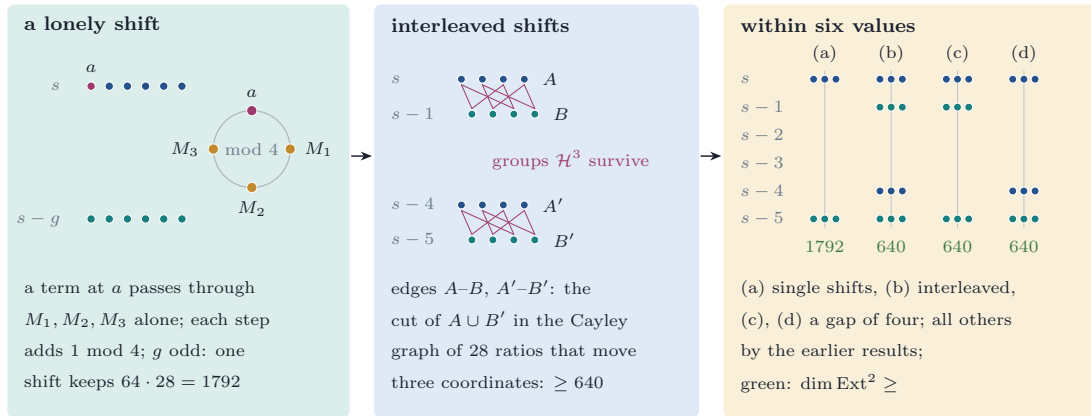
FIGURE 31. The arrangements within six consecutive values on E_0^8 . Left: the parities at single shifts s and s-g , g odd and at least five; a term on a diagonal class at a piece a runs through M_1, M_2, M_3 and no other piece, and since each step adds one to the shift modulo 4 the four nodes have distinct residues, so the multiples serve at most one of the two shifts and the 1792 diagonal classes at the other survive (Lemma 18.45, Proposition 18.46). Middle: the interleaved shifts; the groups \mathcal{H}^3 between A and B and between A' and B' survive and form a cut of the Cayley graph of the 28 ratios that move three coordinates, of weight at least 640 (Proposition 18.47). Right: the four arrangements left within six values by the results for five values, each with its bound on \dim \text{Ext}^2 (Corollary 18.48).
