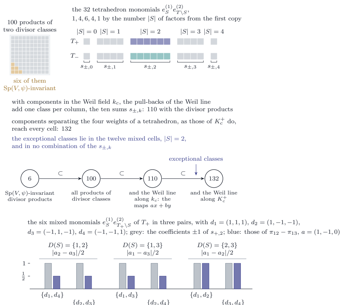
FIGURE 57. Proposition 21.29(ii) and (iii). Top: the 132 Hodge classes of degree four on the square at a CM point, one cell per monomial of weight zero. The 100 products of divisor classes are the cells with an opposite pair; the 32 tetrahedron monomials e_S^{(1)} e_{T \setminus S}^{(2)} are arranged by tetrahedron and by the number |S| of factors from the first copy. Pull-backs of the Weil line along homomorphisms with components in k_c add only the ten symmetric sums s_{\pm,k} , one per column, giving 110; components separating the four weights of a tetrahedron, as those of K_c^+ do, separate the monomials and give all 132. Bottom: on the six mixed monomials of one tetrahedron, grouped in the three pairs by the coordinates in which the two weights of S differ, the symmetric sum s_{+,2} has coefficients \pm 1 throughout, while an exceptional class \omega_a has coefficients of absolute value |a_2 - a_3|/2 , |a_1 - a_3|/2 , |a_1 - a_2|/2 , drawn for \pi_{12} - \pi_{13} ; two equal absolute values would be a linear relation among the conjugates of an irrational element of F .
