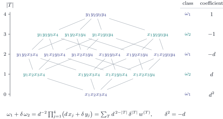
FIGURE 3. The 2^{2n} = 16 monomials w^{(T)} of Notation 4.8 at n = 2 , as the vertices of the 4-cube, projected so that the height of w^{(T)} is |T| . An edge joins two monomials whose index sets differ in one element, that is, two monomials related by a single substitution x_j \mapsto y_j . The two colours are the bipartition by the parity of |T| : the eight even vertices carry \omega_1 and the eight odd ones carry \omega_2 . The coefficient of w^{(T)} depends only on |T| and is given by (13) and (14).
