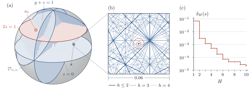
FIGURE 19. The dichotomy of Corollary 16.5. Each stratum \Sigma_{P,q} is Zariski closed by Theorem 16.4, and there are countably many of them; the base point s_0 of Theorem 15.27 lies on one. By Proposition 16.7 the union of the strata is dense, so every neighbourhood of a point s lying off all of them meets infinitely many strata. The conjecture for the family is the assertion that no such s exists, and by Corollary 16.5 it is enough that one stratum has nonempty interior.
