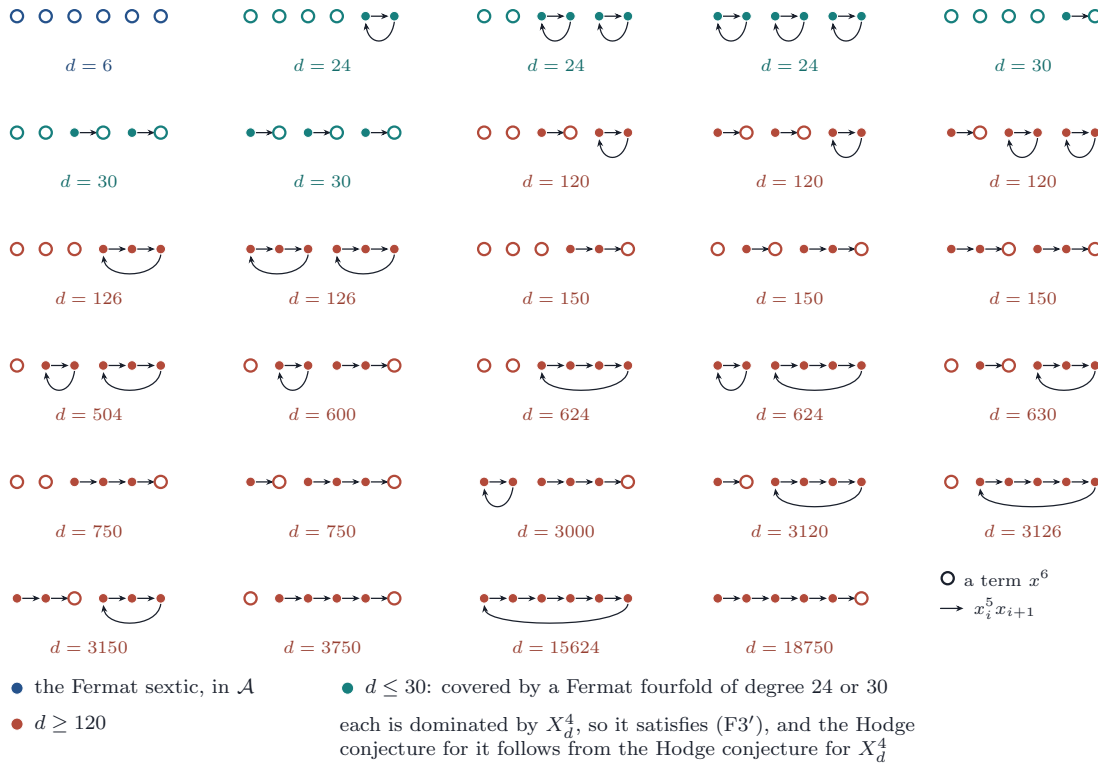
FIGURE 43. The 29 smooth sextic fourfolds of Proposition 20.48(iii), up to a renumbering of the variables. Each is drawn on its six variables: an arrow from x_i to x_j is a term x_i^5 x_j , and a ring is a term x^6 , so a chain is a path of arrows ending at a ring and a loop is a cycle of arrows. Under each is the least d with dA^{-1} integral, the degree of the Fermat fourfold that covers it. All of them satisfy (F3').
