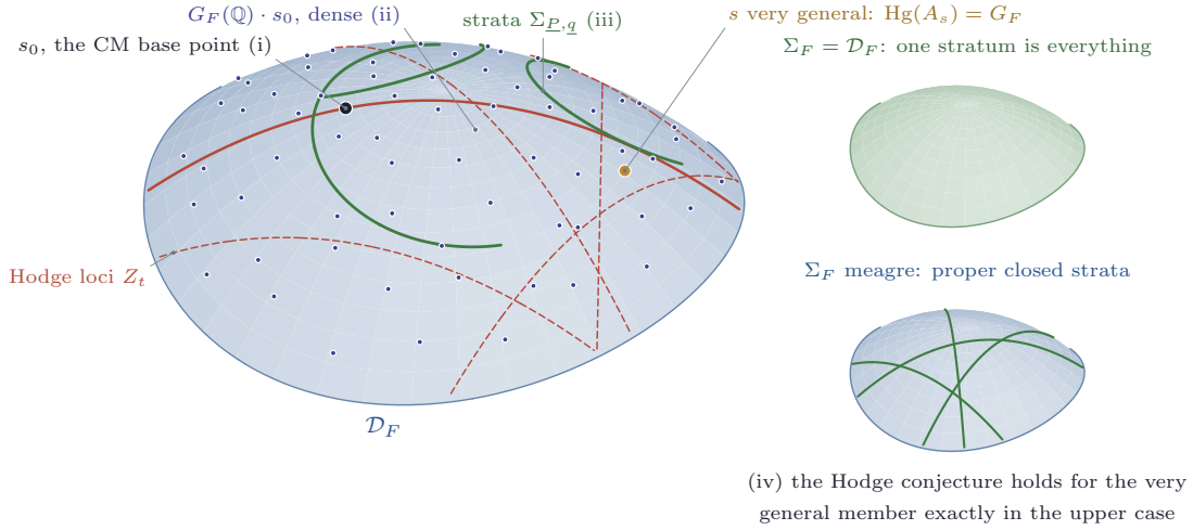
FIGURE 2. The algebraic locus of Theorem 1.1 , drawn over a real slice of the period domain \mathcal{D}_F . Left: the explicit CM base point s_0 of part (i); its Hecke orbit G_F(\mathbb{Q}) \cdot s_0 , which is dense by part (ii); three of the strata \Sigma_{P,q} of part (iii), each closed and algebraic, through points of the orbit; the Hodge loci Z_t , dashed, one of them through s_0 , off which the Hodge group of the member is all of G_F ( Lemma 19.4 ); and a very general point s . Right: the two cases of the dichotomy of part (iii). By part (iv) the Hodge conjecture holds for the very general member exactly in the upper case, where one stratum is the whole domain.
