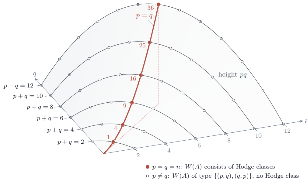
FIGURE 64. The signatures (p, q) of an imaginary quadratic action, with p + q = \dim A , drawn on the surface of height pq , which is the dimension of the family of abelian varieties carrying that action, the unitary Shimura variety of signature (p, q) . Each curve on the surface collects the signatures available in one dimension, and on it the diagonal point is the highest. The divisibility conditions of Theorem C.3 put no constraint on which of them occur when \text{End}^0(A) = K , by Proposition C.9(i) . By Proposition C.7 the Weil line consists of Hodge classes exactly at the filled points on the ridge p = q , and at every open point it is a rational sub-Hodge structure of type \{(p, 2n - p), (2n - p, p)\} carrying no Hodge class at all. The diagonal is the locus that Corollary B.9 shows to be an algebraic subvariety of the moduli.
