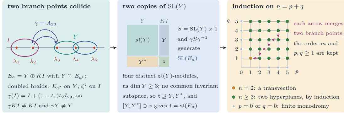
FIGURE 46. The proof of Proposition 20.64. Left: two branch points \lambda_1, \lambda_2 collide inside a disc (Lemma 20.60); the cycles outside the disc form the hyperplane Y \cong E_{a'} , the cycle I of the disc spans the complementary line, and the twist \gamma of the second and third points moves both. Middle: the two copies of SL(Y) of Lemma 20.61, which generate SL(E_a) when \dim Y \geq 3 . Right: the induction on n = k - 2 , each merge lowering p or q by one (Lemma 20.62, Lemma 20.63), down to n = 2 , where the full twist of two points with opposite exponents is a transvection.
