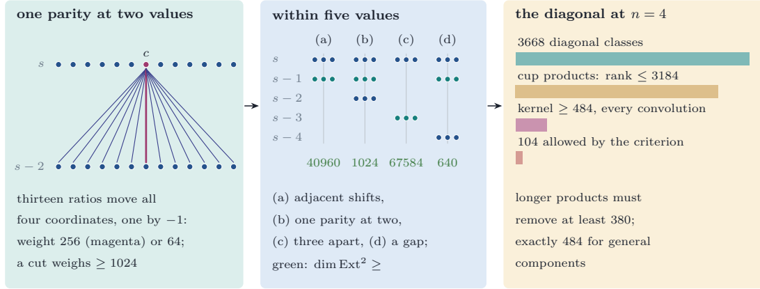
FIGURE 30. The shift arrangements of the pieces L_\zeta on E_0^8 . Left: one parity at two values two apart; a piece c is joined to the thirteen pieces whose ratio moves every coordinate, one by -1 , and the groups \mathcal{H}^4 of the edges crossing between the values survive, weighing at least 1024 (Lemma 18.39(ii), Lemma 18.40). Middle: the four kinds of arrangement within five consecutive values, with the result that excludes each and its bound on \dim \text{Ext}^2 . Right: the diagonal at n = 4 ; the cup products leave at least 484 of the 3668 classes, and the criterion allows 104 (Proposition 18.49).
