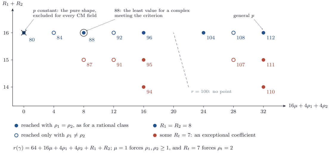
FIGURE 37. The rank r(\gamma) of Theorem 19.29 , over the plane of the Hankel part 16\mu + 4\rho_1 + 4\rho_2 and of R_1 + R_2 . The fifteen points are the tuples allowed by the two conditions of the theorem, and each carries its value. Filled points are reached with \rho_1 = \rho_2 , as the character of a complex with rational coefficients is ( Corollary 19.30(ii) ); red points need an exceptional coefficient at one place at least. The value 80 is the pure shape, excluded for every CM field by Theorem 19.19 ; so 88 is the least rank a complex meeting the criterion can have. The level r = 100 meets no point.
