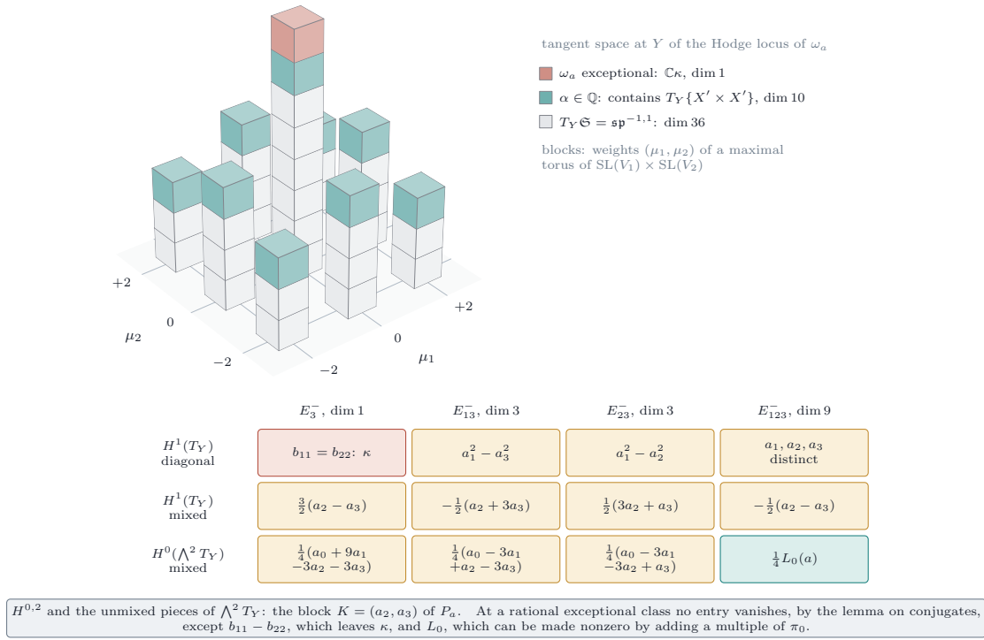
FIGURE 55. Theorem 21.21. Top: the tangent space \mathfrak{sp}^{-1,1} of the Siegel space \mathfrak{S} at Y = X_c \times X_c , of dimension 36, split into nine blocks by the weights of a maximal torus of \mathrm{SL}(V_1) \times \mathrm{SL}(V_2) , one cube for each dimension. The tangent space of the Hodge locus of an exceptional class is the line \mathbb{C}\kappa of the Mumford curve, in the block of weight (0, 0) ; for \alpha \in \mathbb{Q} it contains the tangent space of the diagonal Siegel space, of dimension 10 ( Remark 21.22 ). Bottom: the scalars of Steps 4 to 6 of the proof on the pieces E_J^- of HT^2(Y) ; the pieces of H^{0,2} and the unmixed pieces of H^0(\wedge^2 T_Y) are controlled by the block K of P_a (Steps 3 and 4).
