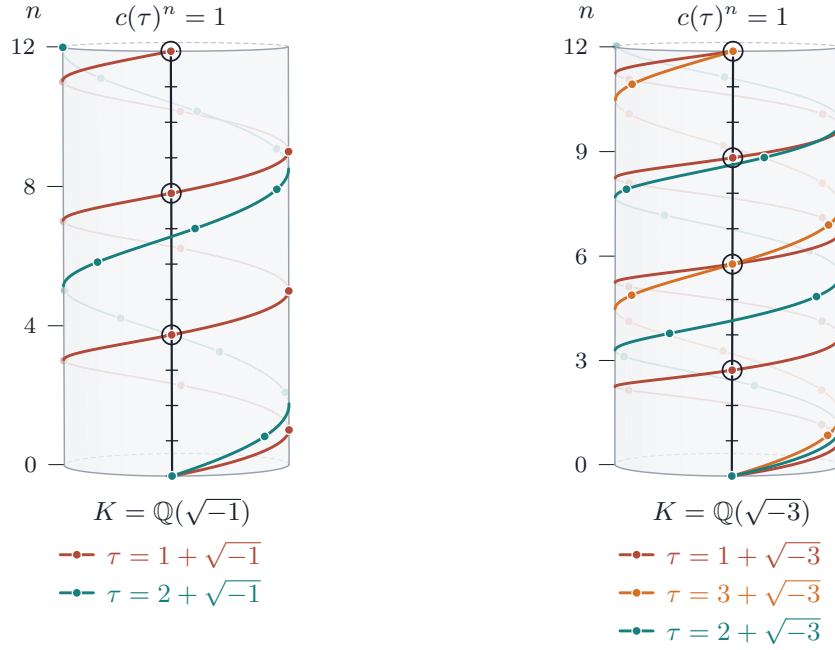
FIGURE 5. Remark 5.5. The values c(\tau)^n = (\tau/\bar{\tau})^n , 0 \leq n \leq 12 , on the unit circle, stacked over n as a helix; the characters \tau^{2n} and N^n agree at \tau exactly where the helix meets the vertical line c^n = 1 (circled). Left, K = \mathbb{Q}(\sqrt{-1}) : the candidate 1 + \sqrt{-1} returns every fourth step, and 2 + \sqrt{-1} never. Right, K = \mathbb{Q}(\sqrt{-3}) : 1 + \sqrt{-3} returns every third step, 3 + \sqrt{-3} every sixth, and 2 + \sqrt{-3} never.
