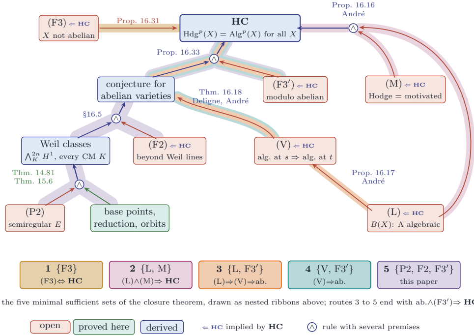
FIGURE 25. The rule set of Setup 16.39 with the rules of Section 16.6 , drawn as a hypergraph. A rule with several premises is a junction marked \wedge , with arrows from its premises and one arrow to its conclusion; each rule carries the result that proves it, and the junction marked §16.5 is the closure map of Section 16.5 . Clay marks an open statement, grass what this paper proves, indigo a derived statement, and the tag \Leftarrow \text{HC} an open statement that the conjecture implies: every clay node except (P2). The arrow from (F3) to the conjecture is Proposition 16.35 , and the junction above the conjecture for abelian varieties is Proposition 16.37(i) . The five minimal sufficient sets of Theorem 16.40(ii) are drawn as nested ribbons under the arrows they use, widest first, and listed in the cards below: (F3) alone; (L) with (M); (L) through (V) with (F3'); (V) with (F3'); and, on the left, (P2) with (F2) and (F3'). A shared arrow shows the bands of every route through it. The secant route, which reaches the imaginary quadratic families only, is drawn in Figure 26 .
