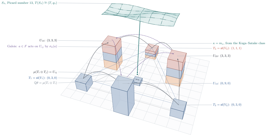
FIGURE 43. Proposition 21.2 and Lemma 21.3 , drawn over the triangle of the three factors of the Hodge group; every height is a dimension. At the corners stand the summands T_i = \mathfrak{sl}(V_i) of T = \text{Lie } G , banded by Hodge type after the Tate twist T(-1) : blue for (1, 1) , clay for (2, 0) and amber for (0, 2) , so that only T_3 carries the K3 type. On the edges stand the three summands U_{ij} of the primitive part of H^2(X) , of dimension nine, U_{12} of pure type (1, 1) and the other two in three bands of three; in the middle is the line of \theta . The solid arcs are the product map \mu , which carries T_i \otimes T_j onto U_{ij} , and the dashed ones carry T_i \otimes T_i to \mathbb{Q}\theta . The violet arcs are the Galois group permuting the U_{ij} as it permutes the embeddings of F , which is why the two exceptional classes may be taken to be the trace-zero part of a cubic field. Above, the K3 surface S_\lambda of Theorem 21.4 , whose Kuga–Satake class, if algebraic, comes down to T as the map \kappa = m_e .
