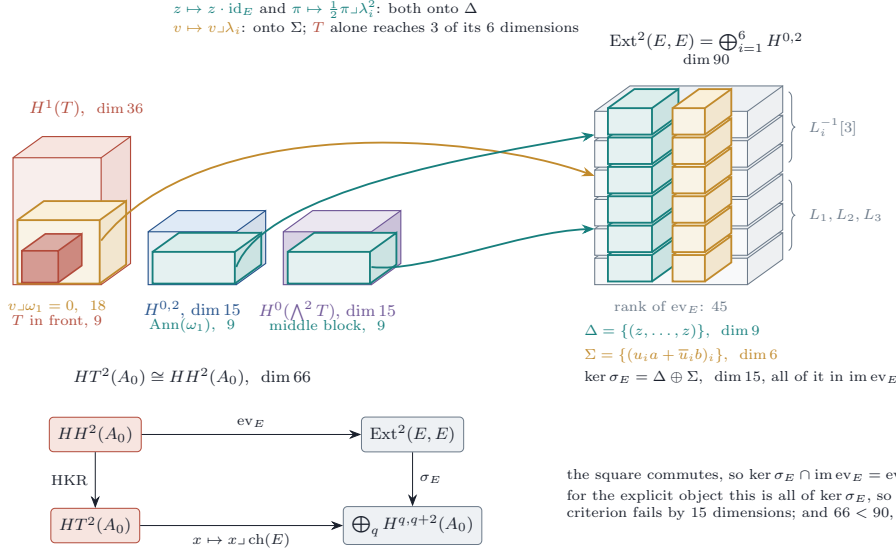
FIGURE 23. Proposition 18.18 for the explicit object at n = 3 . Left: the three summands of HT^2(A_0) , drawn with heights proportional to their dimensions, and inside each the part that preserves \text{ch}(E) to first order: the annihilator of \omega_1 , the deformations killing \omega_1 with the polarised K -commuting tangent space T in front, and the middle block of bivectors. Right: \text{Ext}^2(E, E) as six stacked copies of H^{0,2} , one per summand of E , and inside it the kernel of \sigma_E : the column \Delta , one and the same class in every layer, and the column \Sigma , whose entries depend on the summand through u_i . The three arrows are the evaluation map on the three kernels; the two teal ones both land on \Delta , the ochre one on \Sigma , and together they cover the kernel. Below, the commutative square that makes this a statement about the weakened criterion of [Mar25b, Question 11.4] .
