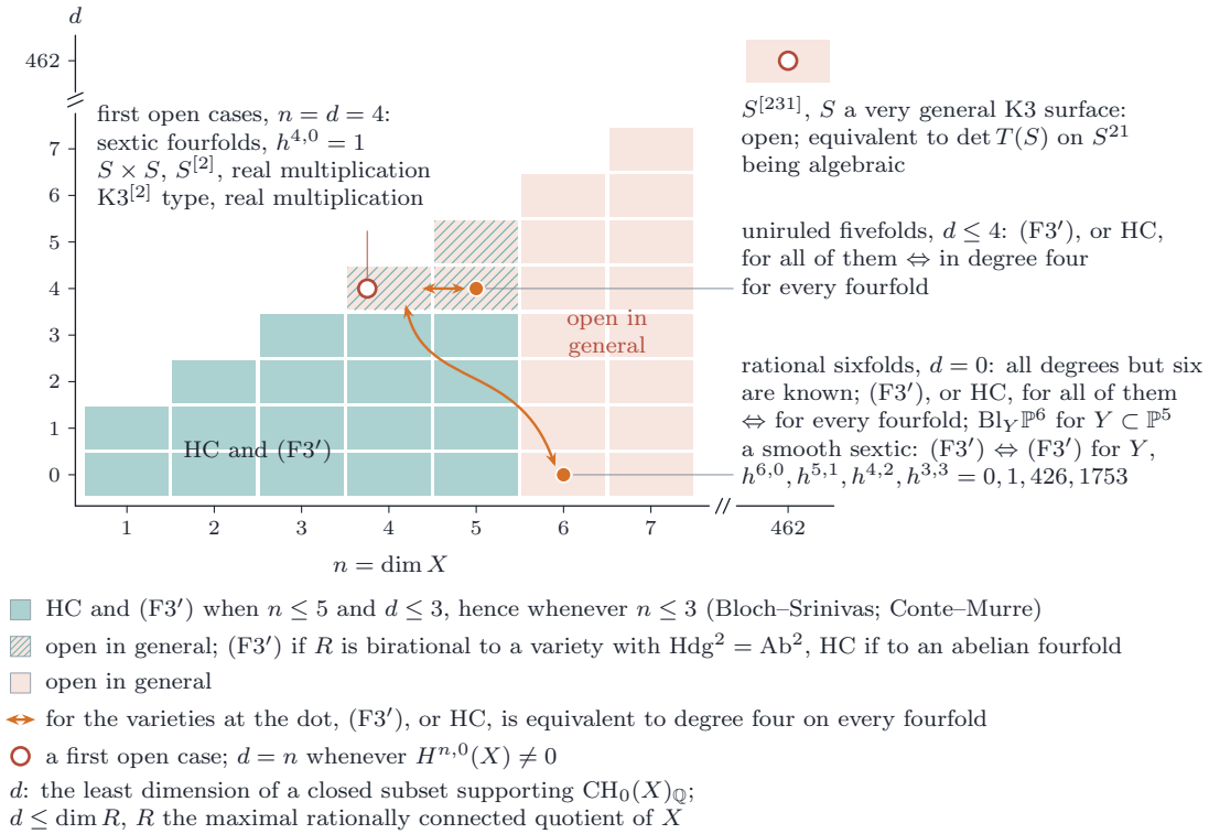
FIGURE 39. What arguments on zero-cycles and on rationally connected fibrations give for (F3') and for the Hodge conjecture (HC in the figure) on a variety X , over the plane of n = \dim X and the least dimension d of a closed subset supporting \text{CH}_0(X)_{\mathbb{Q}} ; d is at most the dimension of the maximal rationally connected quotient R of X , and d = n whenever H^{n,0}(X) \neq 0 (Remark 20.47). Both hold when n \leq 5 and d \leq 3 (Proposition 20.45), hence on every variety of dimension at most three. In the hatched cells (F3') holds when R is birational to a variety with \text{Hdg}^2 = \text{Ab}^2 , for instance a member of \mathcal{A} , and the Hodge conjecture when R is birational to an abelian fourfold (Proposition 20.46). The double arrows are the equivalences of Remark 20.47: (F3') , and the Hodge conjecture, hold for every uniruled fivefold, and for every rational sixfold, if and only if they hold in degree four for every fourfold; the sixfold Bly \mathbb{P}^6 of a smooth sextic fourfold Y in a hyperplane carries the Hodge numbers listed. The rings are the frontier cases (Remark 20.56): the sextic fourfolds, the first family of smooth hypersurfaces beyond these results (the 29 Delsarte sextics lie in \mathcal{A} by Corollary 20.54); S \times S and S^{[2]} for a K3 surface S with real multiplication, such as S_{\lambda} ; the fourfolds of K3^{[2]} type with real multiplication, among them F(Y) ; and, beyond the breaks of the axes, S^{[231]} for a very general K3 surface, which is equivalent to the algebraicity of \det T(S) on S^{21} (Proposition 20.41, Figure 36).
