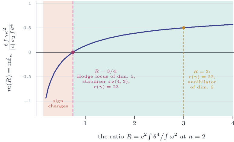
FIGURE 21. The exceptional ratio of Remark 17.12. By the identity displayed there, which is linear in \gamma , the infimum over the Kähler cone of 6 \int \gamma \kappa^2 / (|c| \sigma_2(h) \int \theta^4) is m(R) = 1 - \sqrt{3/(4R)} , approached at the boundary of the cone by a positive hermitian form of rank two whose Plücker coordinates satisfy |\xi_{01} \xi_{23}| = \frac{1}{4} . It is negative exactly for R < 3/4 , and R = 3/4 is also where the Hodge locus of \gamma jumps from dimension 4 to 5 and its stabiliser becomes \mathfrak{so}(4, 3) , with r(\gamma) = 23 ; at R = 3 the annihilator has dimension 6 and r(\gamma) = 22 . The computations of [BMB26] check these values.
