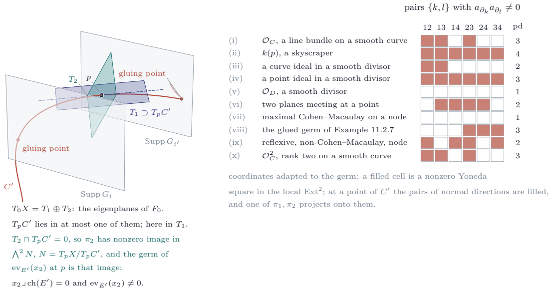
FIGURE 31. Theorem 19.44 and Corollary 19.46 . Left: the support of Markman's sheaf E' near a point p of the glued curve C' , between two of the translated supports that the curve crosses at its gluing points. The tangent space at p is the sum of the eigenplanes T_1 and T_2 of the real multiplication; the tangent line of C' lies in at most one of them, here in T_1 , so \pi_2 has nonzero image in \wedge^2 N , N = T_pX/T_pC' , which is the germ of \text{ev}_{E'}(x_2) at p . Right: for ten germs at the origin of \mathbb{C}^4 , the pairs \{k, l\} of coordinate directions whose jet classes have nonzero product in the local \text{Ext}^2 , and the projective dimension; rows (i), (ii) and (x) are Lemma 19.42 , row (iii) is Lemma 19.43 , row (vi) is Lemma 18.48 .
