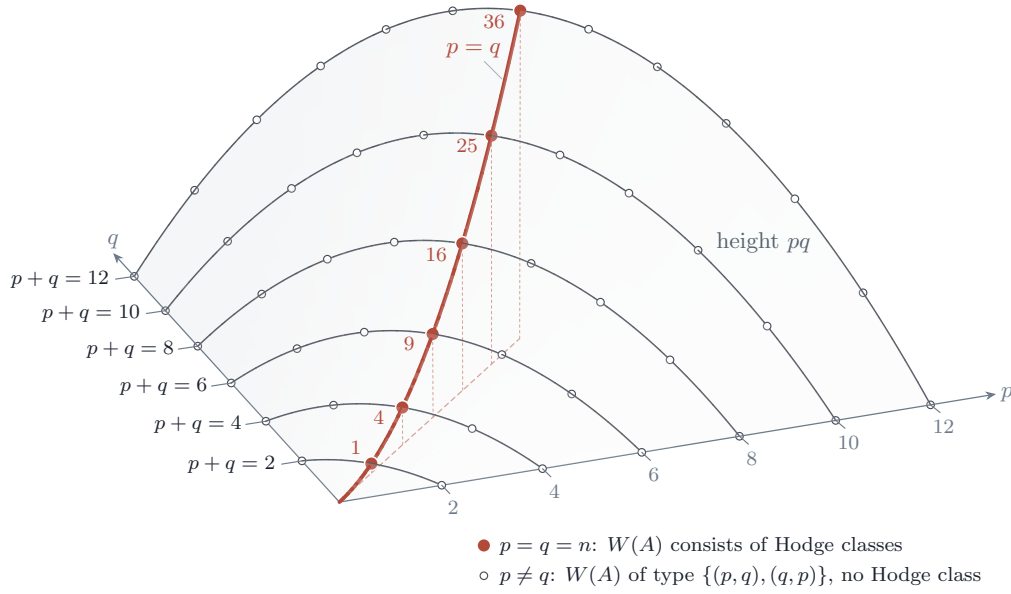
FIGURE 52. The signatures (p, q) of an imaginary quadratic action, with p + q = \dim A , drawn on the surface of height pq , which is the dimension of the family of abelian varieties carrying that action, the unitary Shimura variety of signature (p, q) . Each curve on the surface collects the signatures available in one dimension, and on it the diagonal point is the highest. The divisibility conditions of Theorem C.3 put no constraint on which of them occur when \text{End}^0(A) = K , by Proposition C.9(i) . By Proposition C.7 the Weil line consists of Hodge classes exactly at the filled points on the ridge p = q , and at every open point it is a rational sub-Hodge structure of type \{(p, 2n - p), (2n - p, p)\} carrying no Hodge class at all. The diagonal is the locus that Corollary B.9 shows to be an algebraic subvariety of the moduli.
