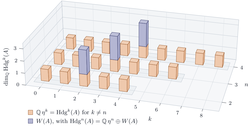
FIGURE 3. The dimensions of \text{Hdg}^k(A) for a general abelian variety of (K, -1, n) -Weil type, 0 \leq k \leq 2n , at n = 2, 3, 4 , as computed in Theorem 4.14 . Every degree carries the line \mathbb{Q}\eta^k ; the middle degree k = n carries in addition the two dimensions of the Weil line W(A) , and nothing else occurs. The profile is the same for every n .
