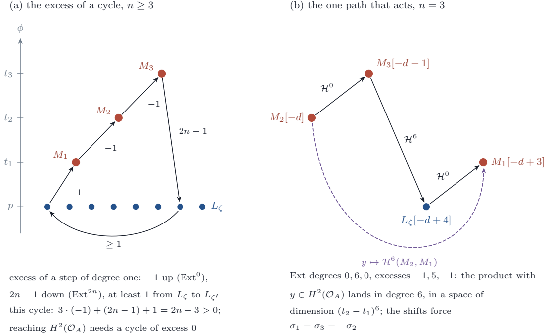
FIGURE 24. The pieces of Proposition 18.28 at their values \phi , with \phi(L_\zeta) = p and \phi(M_i) = t_i . (a) A step of degree one between pieces with a definite difference has Ext degree 0 going up and 2n going down, so excess -1 or 2n - 1 ; a step between two L_\zeta has excess at least 1. The cycle drawn runs up through all three M_i and down once, the worst case, and still has excess 2n - 3 > 0 , so for n \geq 3 no term reaches the diagonal ( Proposition 18.30 ). (b) The one path whose products act on the diagonal at n = 3 when the t_i lie above p ( Theorem 18.32(i) ), drawn at the same heights and in the order of the convolution, with the Ext degrees of its steps and the shifts they force; the dashed arrow is the value of the product with a diagonal class y .
