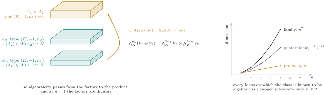
FIGURE 15. Theorem 15.7 and its reach. Left: the Weil line of each factor is a K -line, the Weil line of the product is the tensor product of the two over K , and in the K -valued notation the class is multiplicative up to the factor 2. Algebraicity therefore passes from the factors to the product, and at n = 1 the factors are divisor classes, so a product of n abelian surfaces of Weil type carries an explicit algebraic Weil class in every dimension. Right: the dimensions of the loci on which the class is known to be algebraic, against the dimension n^2 of the family. Both the quaternionic locus and the product locus are proper subvarieties once n \geq 2 , and a general member lies on neither.
