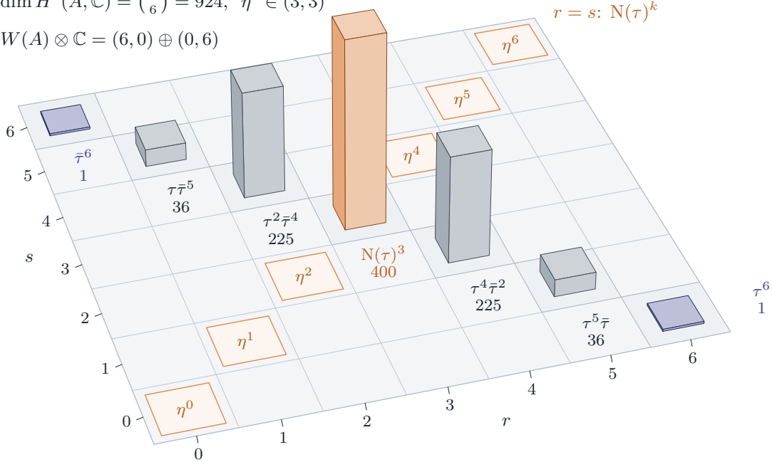
FIGURE 4. The K^\times -grading at n = 3 on the grid of pairs (r, s) , 0 \leq r, s \leq 6 . The summands \bigwedge^r V_+ \otimes \bigwedge^s V_- of H^6(A, \mathbb{C}) lie on the antidiagonal r + s = 6 and are drawn at their dimensions \binom{6}{r}\binom{6}{s} , which sum to \binom{12}{6} = 924 ; on the summand (r, s) the group K^\times acts by \tau^r \bar{\tau}^s . The two end cells (6, 0) and (0, 6) , with characters \tau^6 and \bar{\tau}^6 , span the Weil line; the middle cell (3, 3) , with character N(\tau)^3 , contains \eta^3 . The outlined cells on the diagonal r = s are the summands on which K^\times acts through a power of the norm, and they carry the powers \eta^k . That the end cells and the middle cell differ is the content of Theorem 5.6 .
