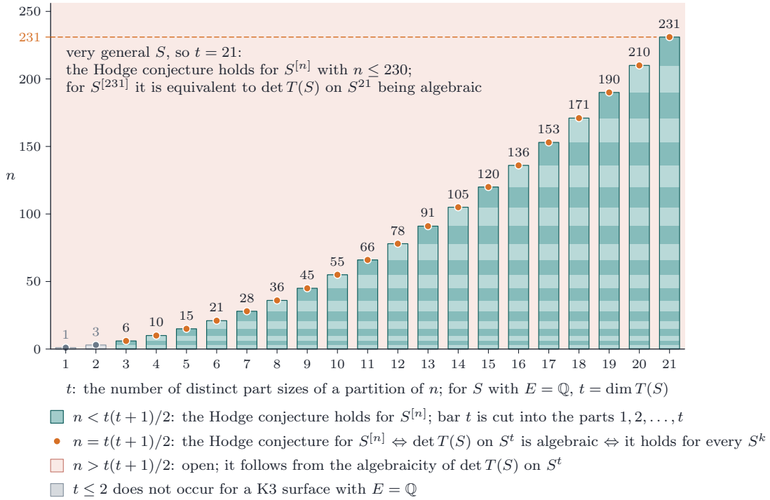
FIGURE 36. The threshold of Proposition 20.41(ii). For t = 1, \dots, 21 the bar rises to t(t+1)/2 , the least n that has a partition with t distinct part sizes, and is cut into the parts 1, 2, \dots, t of the partition that attains it. For a K3 surface S with E = \text{End}_{\text{Hdg}}(T(S)) = \mathbb{Q} and t = \dim T(S) , which is at least 3, the Hodge conjecture holds for S^{[n]} with n below the bar; at its top it is equivalent to the algebraicity of the class \det T(S) on S^t of Proposition 20.40, and to the Hodge conjecture for every power of S ; above it, it follows from that algebraicity. A very general S has t = 21 : the conjecture holds for S^{[n]} with n \leq 230 , and for S^{[231]} it is equivalent to the algebraicity of \det T(S) on S^{21} , one of the frontier cases of (F3') (Remark 20.56).
