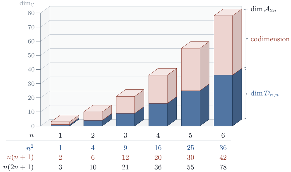
FIGURE 11. The Weil locus inside the moduli of principally polarised abelian 2n -folds, for n = 1, \dots, 6 . Each prism has the height n(2n+1) of the moduli space \mathcal{A}_{2n} ; its lower part, of height n^2 , is the dimension of the period domain \mathcal{D}_{n,n} of Proposition B.8, and its upper part is the codimension n(n+1) . The codimension grows quadratically, so the Weil locus is thin, and by Corollary B.9 it is an algebraic subvariety. Both facts matter for propagation: the locus along which one would have to deform is small and is a variety, but neither fact produces a cycle on it.
