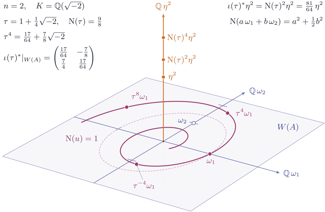
FIGURE 5. The linear algebra behind Theorem 7.3 , drawn inside H^{2n}(A, \mathbb{Q}) . The Weil line W(A) is a plane, free of rank one over K and of rank two over \mathbb{Q} , and K^\times acts on it through \tau^{2n} , so the orbit of any nonzero class is a spiral that spans the plane and lies on no line in it. The transverse axis carries \eta^n , on which K^\times acts through the norm. A construction returning a single eigenclass returns a line, and by Proposition 13.1 no line inside W(A) is stable.
