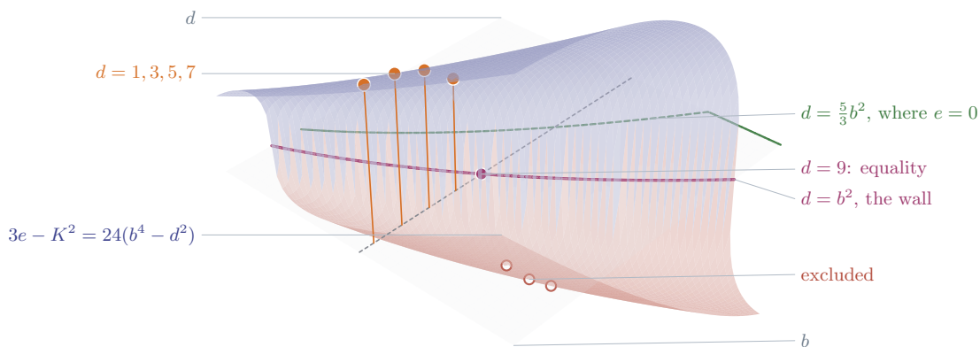
FIGURE 22. Theorem 14.135 over the quarter plane of (b, d) . The height of the surface is the defect 3e(S) - K_S^2 = 24(b^4 - d^2) in the Bogomolov–Miyaoka–Yau inequality for the surface the theorem attaches to the pair, compressed by a signed cube root so that four orders of magnitude fit one frame; the compression is odd and monotone, so the zero locus and the sign are the true ones. The surface is drawn indigo where the defect is positive and clay where it is negative, and it crosses zero along d = b^2 , which is therefore the whole content of the inequality. The weaker wall d = \frac{5}{3}b^2 , where e(S) itself changes sign, is drawn dashed and lies above it. On the line b = 3 , which is the value Proposition 14.120(iii) forces on the fourfold, the four squarefree discriminants d = 1, 3, 5, 7 with N an integer sit above the wall and are marked with their drop lines; d = 9 sits exactly on it, the equality case, and d = 11, 13, 15 sit below and are excluded.
