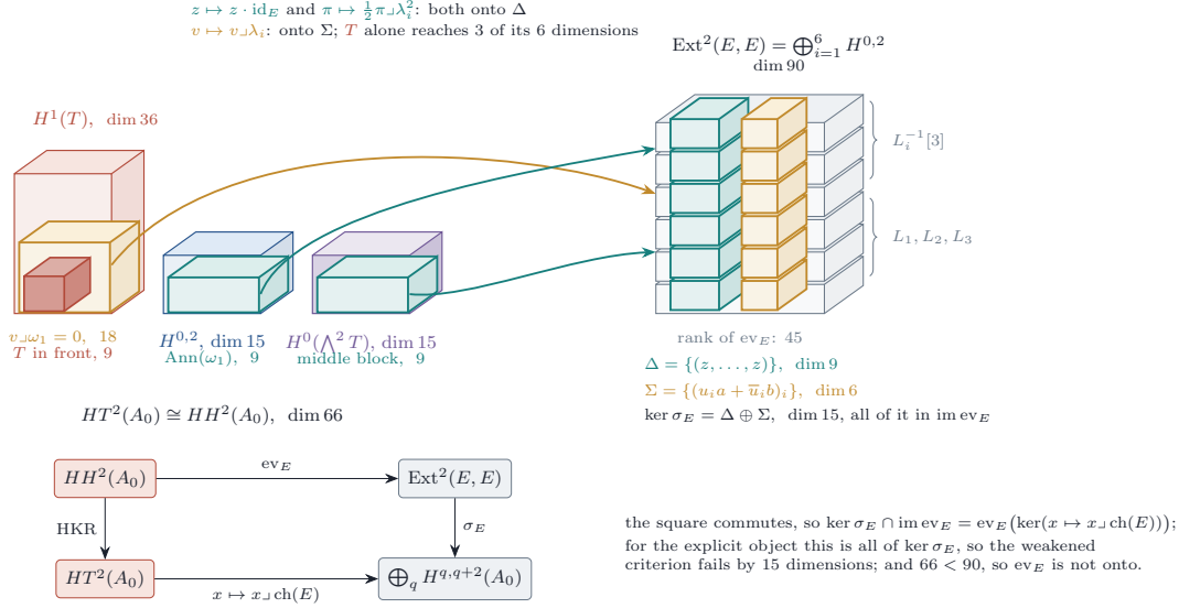
FIGURE 19. Proposition 14.113 for the explicit object at n = 3 . Left: the three summands of HT^2(A_0) , drawn with heights proportional to their dimensions, and inside each the part that preserves \text{ch}(E) to first order: the annihilator of \omega_1 , the deformations killing \omega_1 with the polarised K -commuting tangent space T in front, and the middle block of bivectors. Right: \text{Ext}^2(E, E) as six stacked copies of H^{0,2} , one per summand of E , and inside it the kernel of \sigma_E : the column \Delta , one and the same class in every layer, and the column \Sigma , whose entries depend on the summand through u_i . The three arrows are the evaluation map on the three kernels; the two teal ones both land on \Delta , the ochre one on \Sigma , and together they cover the kernel. Below, the commutative square that makes this a statement about the weakened criterion of [Mar25b, Question 11.4] .
