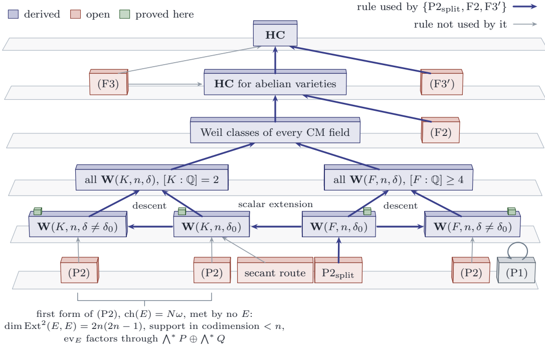
FIGURE 37. The route of this paper through the rule set of Theorem 20.58 , drawn as a stack of plates, one per level of the derivation; the other routes are drawn in Figure 36 . Heavy arrows are the rules used by the minimal set \{P2_{\text{split}}, F2, F3'\} , light arrows the rules it does not use. The bottom plate carries the propagation statement, read in the corrected form of Remark 17.6 , once for each of the four kinds of Weil family, with the secant route beside it. The small grass blocks on the next plate are the base points of Theorem 15.27 and Theorem 19.4 , one in every family. The three arrows inside that plate are Proposition 20.13 : descent from the trivial discriminant to the others, and scalar extension from the fields of degree at least four to the quadratic fields. With them (P2) is needed only for the split families of the fields of higher degree, and the other three (P2) blocks are not used. (F2) is the conjecture for the Hodge classes that no Weil line reaches, and (F3) is the whole conjecture ( Proposition 20.35 ), so the route is minimal only with (F3) replaced by (F3') of Definition 20.36 . The bracket under the two quadratic (P2) blocks records the first form of the criterion, in which the Chern character is exactly a Weil class, as Theorem 16.36 , Theorem 16.38 and Corollary 16.34 describe it; by Theorem 17.5 that form is met by no complex. The secant route reaches the trivial discriminant, since the member it is built on is split, and through descent the rest of the quadratic case; it has no edge to the fields of higher degree. The bounded criterion (P1) stands apart, closed on itself: it is equivalent to its own conclusion.
