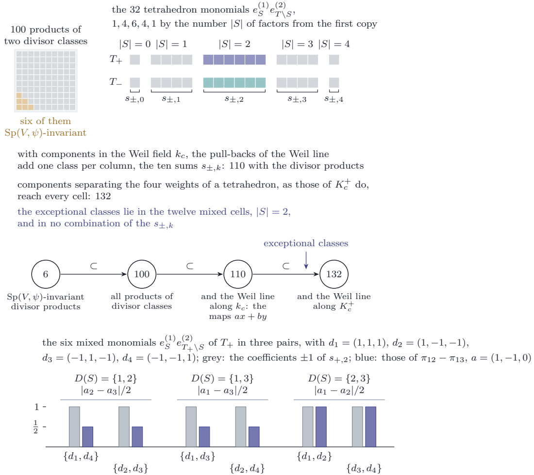
FIGURE 42. Proposition 21.29(ii) and (iii). Top: the 132 Hodge classes of degree four on the square at a CM point, one cell per monomial of weight zero. The 100 products of divisor classes are the cells with an opposite pair; the 32 tetrahedron monomials e_S^{(1)} e_{T \setminus S}^{(2)} are arranged by tetrahedron and by the number |S| of factors from the first copy. Pull-backs of the Weil line along homomorphisms with components in k_c add only the ten symmetric sums s_{\pm,k} , one per column, giving 110; components separating the four weights of a tetrahedron, as those of K_c^+ do, separate the monomials and give all 132. Bottom: on the six mixed monomials of one tetrahedron, grouped in the three pairs by the coordinates in which the two weights of S differ, the symmetric sum s_{+,2} has coefficients \pm 1 throughout, while an exceptional class \omega_a has coefficients of absolute value |a_2 - a_3|/2 , |a_1 - a_3|/2 , |a_1 - a_2|/2 , drawn for \pi_{12} - \pi_{13} ; two equal absolute values would be a linear relation among the conjugates of an irrational element of F .
