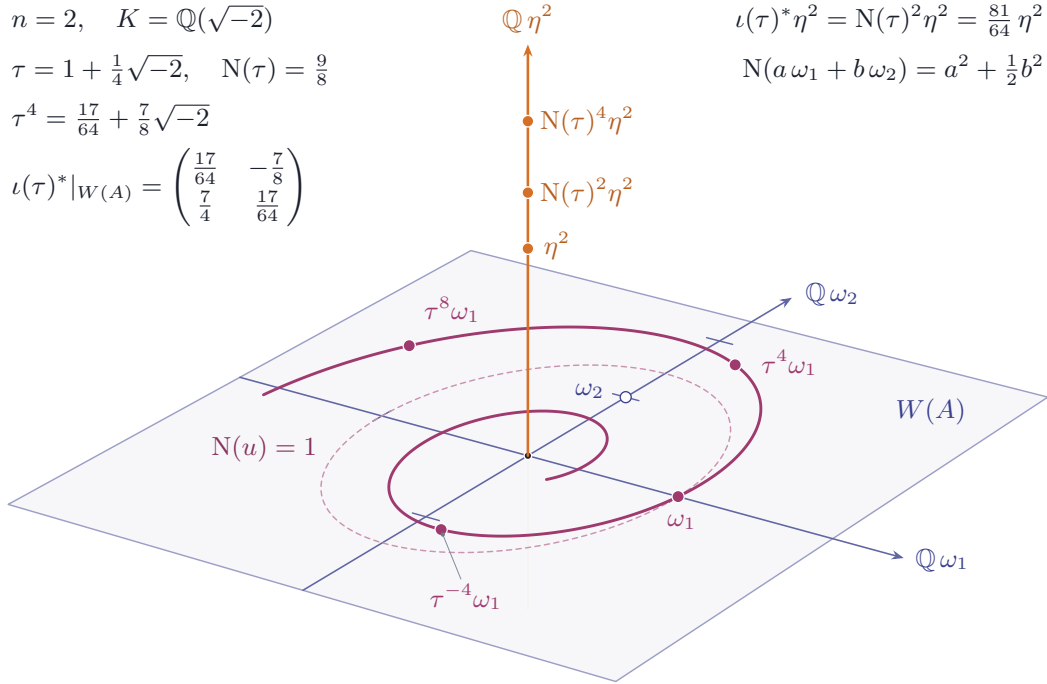
FIGURE 4. The linear algebra behind Theorem 1.1 , drawn inside H^{2n}(A, \mathbb{Q}) . The Weil line W(A) is a plane, free of rank one over K and of rank two over \mathbb{Q} , and K^\times acts on it through \tau^{2n} , so the orbit of any nonzero class is a spiral that spans the plane and lies on no line in it. The transverse axis carries \eta^n , on which K^\times acts through the norm. A construction returning a single eigenclass returns a line, and by Proposition 13.1 no line inside W(A) is stable.
