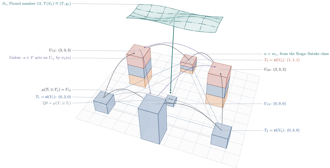
FIGURE 39. Proposition 21.2 and Lemma 21.3, drawn over the triangle of the three factors of the Hodge group; every height is a dimension. At the corners stand the summands T_i = \mathfrak{sl}(V_i) of T = \text{Lie } G , banded by Hodge type after the Tate twist T(-1) : blue for (1, 1) , clay for (2, 0) and amber for (0, 2) , so that only T_3 carries the K3 type. On the edges stand the three summands U_{ij} of the primitive part of H^2(X) , of dimension nine, U_{12} of pure type (1, 1) and the other two in three bands of three; in the middle is the line of \theta . The solid arcs are the product map \mu , which carries T_i \otimes T_j onto U_{ij} , and the dashed ones carry T_i \otimes T_i to \mathbb{Q}\theta . The violet arcs are the Galois group permuting the U_{ij} as it permutes the embeddings of F , which is why the two exceptional classes may be taken to be the trace-zero part of a cubic field. Above, the K3 surface S_\lambda of Theorem 21.4, whose Kuga–Satake class, if algebraic, comes down to T as the map \kappa = m_e .
