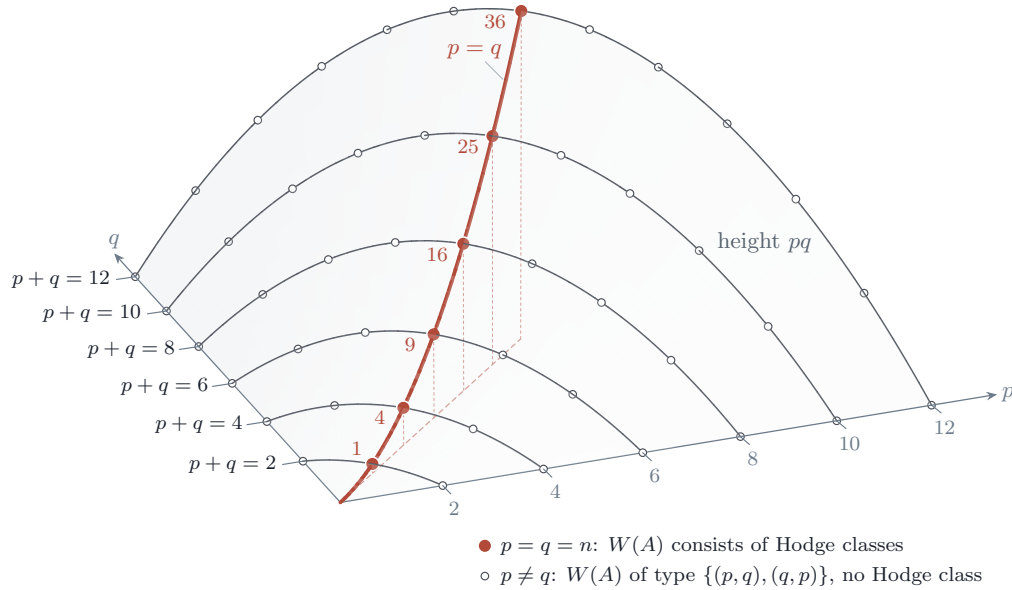
FIGURE 46. The signatures (p, q) of an imaginary quadratic action, with p + q = \dim A , drawn on the surface of height pq , which is the dimension of the family of abelian varieties carrying that action, the unitary Shimura variety of signature (p, q) . Each curve on the surface collects the signatures available in one dimension, and on it the diagonal point is the highest. The divisibility conditions of Theorem C.3 put no constraint on which of them occur when \text{End}^0(A) = K , by Proposition C.9(i) . By Proposition C.7 the Weil line consists of Hodge classes exactly at the filled points on the ridge p = q , and at every open point it is a rational sub-Hodge structure of type \{(p, 2n - p), (2n - p, p)\} carrying no Hodge class at all. The diagonal is the locus that Corollary B.9 shows to be an algebraic subvariety of the moduli.
