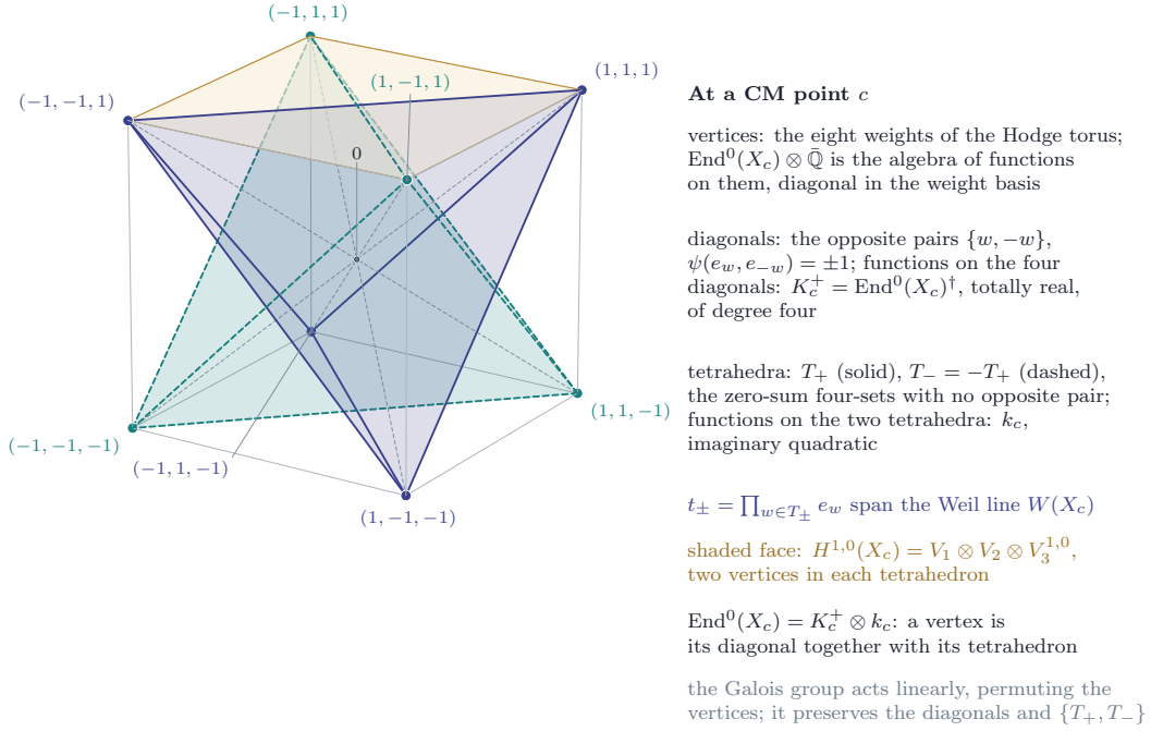
FIGURE 41. Proposition 21.29(i) . The eight weights (\pm 1, \pm 1, \pm 1) of the Hodge torus at a CM point are the vertices of a cube. The four diagonals are the pairs of opposite weights, paired by the polarisation; the two inscribed tetrahedra T_+ (an even number of entries -1 ) and T_- = -T_+ are the only zero-sum four-sets without an opposite pair, and t_{\pm} = \prod_{w \in T_{\pm}} e_w span the Weil line. The Galois group acts by linear maps permuting the vertices, so it preserves the diagonals and the pair of tetrahedra: the functions constant on the tetrahedra form the imaginary quadratic Weil field k_c , those constant on the diagonals the totally real quartic algebra K_c^+ of Rosati-fixed endomorphisms, and \text{End}^0(X_c) = K_c^+ \otimes k_c because a vertex is determined by its diagonal and its tetrahedron.
