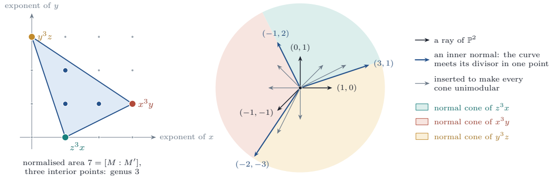
FIGURE 34. The Klein quartic x^3y + y^3z + z^3x in the proof of Theorem 20.53 . Left: its Newton triangle in the lattice M of the torus of \mathbb{P}^2 , in the chart z = 1 , with normalised area 7 = [M : M'] and three interior points, the genus. Right: the rays of a smooth fan adapted to it, the three rays of \mathbb{P}^2 , the three inner normals of the triangle and the six rays inserted to make every cone unimodular. The curve meets only the three divisors of the inner normals, in one point each, the lattice length of the edge, so its Euler number is -7 + 3 = -4 . With e_A = 7 the isogeny of the proof makes it the quotient of the Fermat septic by a group of order seven.
