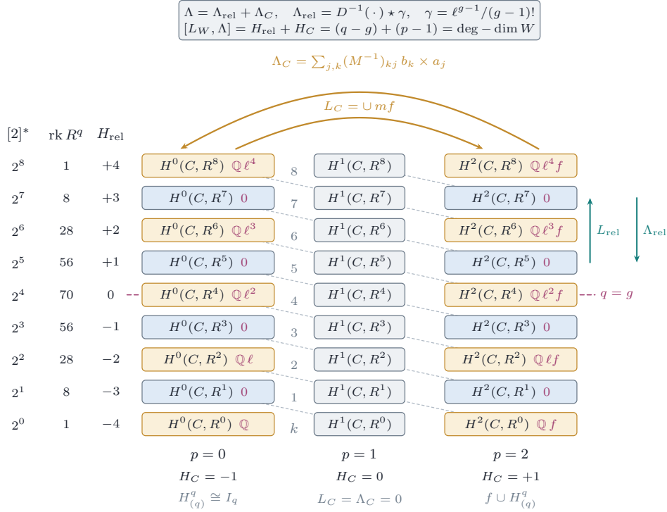
FIGURE 30. The proof of Theorem 20.22 for relative dimension four. The boxes are the summands H^p(C, R^q \pi_* \mathbb{Q}) of H^*(W, \mathbb{Q}) , split off by the eigenvalue 2^q of [2]^* shown on the left; the dotted diagonals join the summands of one H^k(W, \mathbb{Q}) , k = p + q , and the dashed magenta line is the axis q = g of hard Lefschetz on the fibres. The relative operators L_{\text{rel}} and \Lambda_{\text{rel}} , in teal, move within a column; \Lambda_{\text{rel}} is a Pontryagin product with an algebraic class on every abelian scheme ( Proposition 20.21 ). The base operators L_C and \Lambda_C , in ochre, move along a row between the outer columns and kill the middle one; \Lambda_C is the displayed cycle built from bases (a_j) , (b_k) of the invariant summands, and is algebraic exactly when the invariant cycles are. Below each column is the weight of H = [L_W, \Lambda] on it, and the panel at the top is Step 6 of the proof. The ochre boxes carry the invariant cycles and their images under L_C ; for a Mumford family they are the lines listed in magenta on the right, spanned by \ell^i f (and by \ell^i in the left column), and the other boxes of the outer columns are zero ( Corollary 20.23 ).
