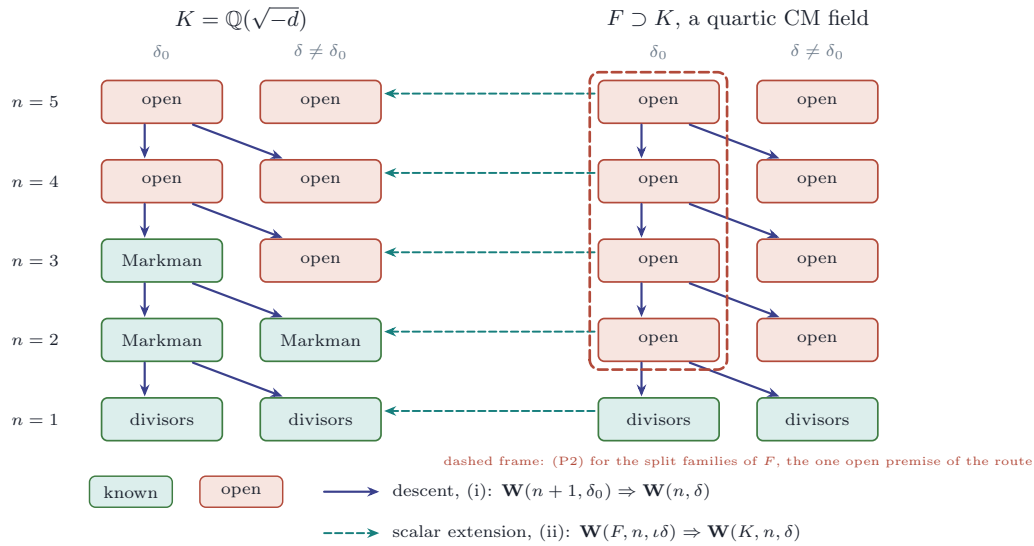
FIGURE 29. The Weil families of an imaginary quadratic field K and of a quartic CM field F \supset K , one cell for each n and each kind of discriminant, grass where the Weil classes are known to be algebraic (divisor classes at n = 1 ; Markman [Mar25a, Mar25b] at n = 2 and at n = 3 , \delta = \delta_0 ) and clay where they are not. The indigo arrows are the descent of Proposition 20.13(i), from the trivial discriminant in dimension n + 1 to every discriminant in dimension n ; the dashed teal arrows are the scalar extension of Proposition 20.13(ii). The dashed frame is the propagation statement for the split families of the field of higher degree, which by Theorem 20.58(ii) is the only form of (P2) that any minimal route to the conjecture uses: every clay cell of the left panel lies below it.
