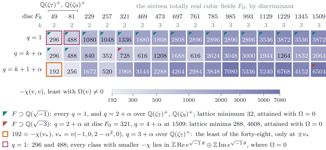
FIGURE 28. Proposition 19.39 case by case. For each of the sixteen totally real cubic fields F_0 of Proposition 19.36(v) , ordered by discriminant, and each of q = 1 , k + \alpha and k + 1 + \alpha , the cell gives the least -\chi(v, v) of an integral point v of S(0, q) whose Orlov square has a nonzero F -Weil part, that is with \Omega(v) \neq 0 ( Lemma 19.38 ), as computed in item (LVIII) of Appendix D ; the shading is logarithmic in this value, which lies between 192 and 7080, and between 296 and 3872 for q = 1 . A corner mark shows that F = F_0(\sqrt{-q}) contains an imaginary quadratic field, \mathbb{Q}(\sqrt{-1}) in eighteen cases and \mathbb{Q}(\sqrt{-3}) in two ( Proposition 19.39(ii) ); in those cases the lattice has classes of smaller -\chi , namely 32, respectively 288 and 4608, all with \Omega = 0 . The heavy frame marks the least value 192, attained only at \pm v_* over \mathbb{Q}(\zeta_7)^+ with q = 3 + \alpha , the target of Remark 19.40 ; the dashed frames mark the values 296 and 488 for q = 1 over \mathbb{Q}(\zeta_7)^+ and \mathbb{Q}(\zeta_9)^+ , below which every integral class lies in \mathbb{Z} \operatorname{Re} e^{\sqrt{-1}\theta} \oplus \mathbb{Z} \operatorname{Im} e^{\sqrt{-1}\theta} ( Proposition 19.39(iii) ). These are least values over the lattices computed, not bounds, and a character does not give a complex; P2_{\text{split}} remains open.
