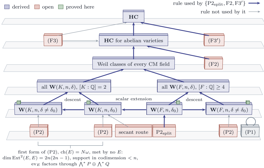
FIGURE 37. The route of this paper through the rule set of Theorem 20.57, drawn as a stack of plates, one per level of the derivation; the other routes are drawn in Figure 36. Heavy arrows are the rules used by the minimal set \{P2_{\text{split}}, F2, F3'\} , light arrows the rules it does not use. The bottom plate carries the propagation statement, read in the corrected form of Remark 17.6, once for each of the four kinds of Weil family, with the secant route beside it. The small grass blocks on the next plate are the base points of Theorem 15.27 and Theorem 19.4, one in every family. The three arrows inside that plate are Proposition 20.13: descent from the trivial discriminant to the others, and scalar extension from the fields of degree at least four to the quadratic fields. With them (P2) is needed only for the split families of the fields of higher degree, and the other three (P2) blocks are not used. (F2) is the conjecture for the Hodge classes that no Weil line reaches, and (F3) is the whole conjecture (Proposition 20.35), so the route is minimal only with (F3) replaced by (F3') of Definition 20.36. The bracket under the two quadratic (P2) blocks records the first form of the criterion, in which the Chern character is exactly a Weil class, as Theorem 16.36, Theorem 16.38 and Corollary 16.34 describe it; by Theorem 17.5 that form is met by no complex. The secant route reaches the trivial discriminant, since the member it is built on is split, and through descent the rest of the quadratic case; it has no edge to the fields of higher degree. The bounded criterion (P1) stands apart, closed on itself: it is equivalent to its own conclusion.
