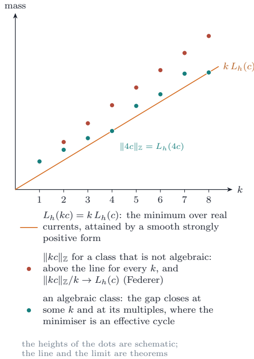
FIGURE 38. Theorem 20.67 and Example 20.68. Left: the mass of a current in the class dual to kc against k . The line k L_h(c) is the minimum over closed real normal currents, attained by a smooth strongly positive form; the minima over closed integral currents lie on or above it, with \|kc\|_{\mathbb{Z}}/k \rightarrow L_h(c) by Federer's theorem, and for M large the class is algebraic exactly when one of them lies on the line, where the minimiser is an effective algebraic cycle. The heights of the dots are schematic. Right: the numbers of the Mumford square, computed in the split model of item (LXIII). Of the seven terms \binom{6}{k} \theta^k \otimes \theta^{6-k} of \theta_Y^6 only k = 3 pairs with \pi_0 = \frac{1}{4} \theta \otimes \theta , giving 20 \cdot 144 = 2880 , and none pairs with the primitive summands; so L_{\theta_Y}(\omega_a) = 4a_0 , the Wirtinger bound of an exceptional class with a_0 = 0 is zero, and the perturbation of NM\theta_Y^2 by N\omega changes the bound 56NM by nothing.
