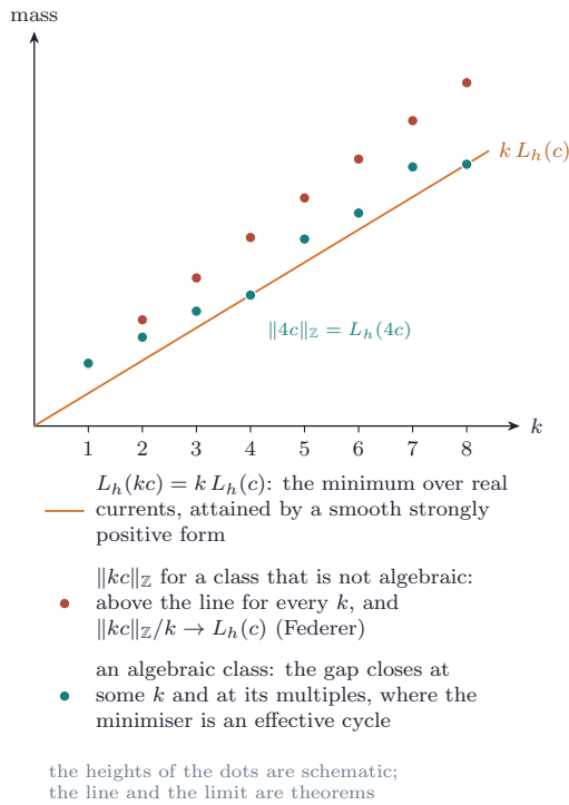
FIGURE 52. Theorem 20.76 and Example 20.77 . Left: the mass of a current in the class dual to kc against k . The line k L_h(c) is the minimum over closed real normal currents, attained by a smooth strongly positive form; the minima over closed integral currents lie on or above it, with \|kc\|_{\mathbb{Z}}/k \rightarrow L_h(c) by Federer's theorem, and for M large the class is algebraic exactly when one of them lies on the line, where the minimiser is an effective algebraic cycle. The heights of the dots are schematic. Right: the numbers of the Mumford square, computed in the split model of [BMB26] . Of the seven terms \binom{6}{k} \theta^k \otimes \theta^{6-k} of \theta_Y^6 only k = 3 pairs with \pi_0 = \frac{1}{4} \theta \otimes \theta , giving 20 \cdot 144 = 2880 , and none pairs with the primitive summands; so L_{\theta_Y}(\omega_a) = 4a_0 , the Wirtinger bound of an exceptional class with a_0 = 0 is zero, and the perturbation of NM\theta_Y^2 by N\omega changes the bound 56NM by nothing.
