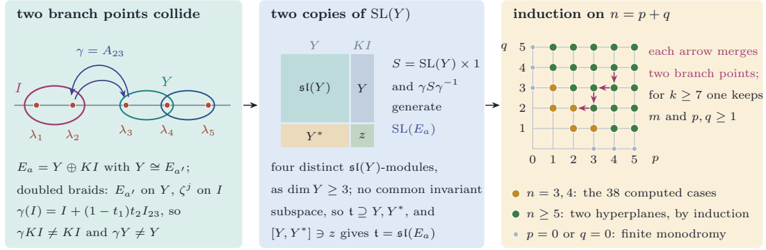
FIGURE 45. The proof of Proposition 20.62. Left: two branch points \lambda_1, \lambda_2 collide inside a disc (Lemma 20.59); the cycles outside the disc form the hyperplane Y \cong E_{a'} , the cycle I of the disc spans the complementary line, and the twist \gamma of the second and third points moves both. Middle: the two copies of SL(Y) of Lemma 20.60 generate SL(E_a) . Right: the induction on n = k - 2 , each merge lowering p or q by one (Lemma 20.61), down to the 38 computed cases with n = 3, 4 .
