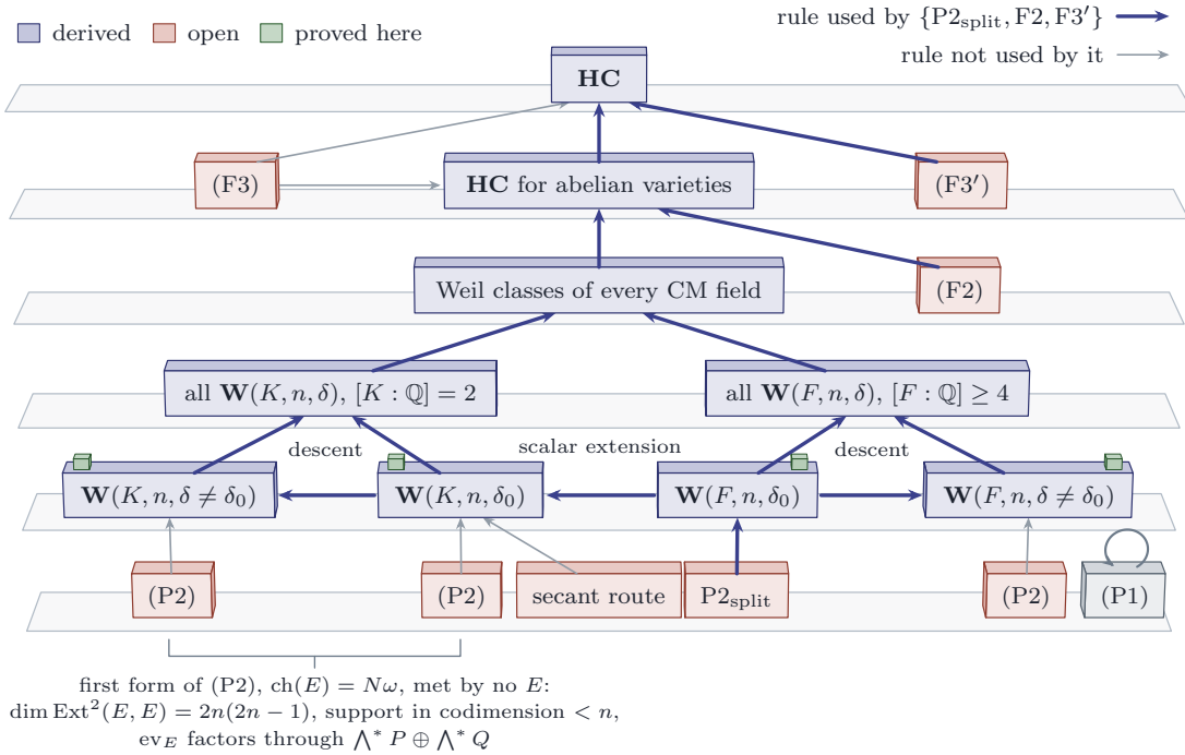
FIGURE 51. The route of this paper through the rule set of Theorem 20.68, drawn as a stack of plates, one per level of the derivation; the other routes are drawn in Figure 50. Heavy arrows are the rules used by the minimal set \{P2_{\text{split}}, F2, F3'\} , light arrows the rules it does not use. The bottom plate carries the propagation statement, read in the polarised form of Remark 17.6, once for each of the four kinds of Weil family, with the secant route beside it. The small grass blocks on the next plate are the base points of Theorem 15.27 and Theorem 19.5, one in every family. The three arrows inside that plate are Proposition 20.13: descent from the trivial discriminant to the others, and scalar extension from the fields of degree at least four to the quadratic fields. With them (P2) is needed only for the split families of the fields of higher degree, and the other three (P2) blocks are not used. (F2) is the conjecture for the Hodge classes that no Weil line reaches, and (F3) is the whole conjecture (Proposition 20.33), so the route is minimal only with (F3) replaced by (F3') of Definition 20.34. The bracket under the two quadratic (P2) blocks records the first form of the criterion, in which the Chern character is exactly a Weil class, as Theorem 16.36, Theorem 16.38 and Corollary 16.34 describe it; by Theorem 17.5 that form is met by no complex. The secant route reaches the trivial discriminant, since the member it is built on is split, and through descent the rest of the quadratic case; it has no edge to the fields of higher degree. The bounded criterion (P1) stands apart, closed on itself: it is equivalent to its own conclusion.
