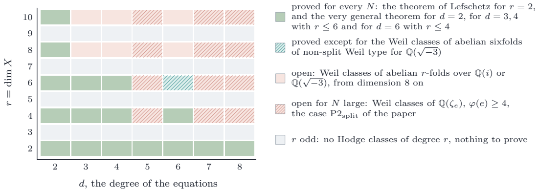
FIGURE 48. The Hodge conjecture for the very general complete intersection X_{d,r}(\lambda) of Vandermonde type, for every N . Grass: proved, by the theorem of Lefschetz for r = 2 and by Theorem 20.64 for d = 2 , for d = 3, 4 with r \leq 6 and for d = 6 with r \leq 4 . Teal hatching: proved except for the Weil classes of abelian sixfolds of non-split Weil type for \mathbb{Q}(\sqrt{-3}) . Clay: open, the Weil classes of abelian varieties of Weil type over \mathbb{Q}(i) or \mathbb{Q}(\sqrt{-3}) in dimension at least eight, or, hatched, of a CM field of degree at least four (Remark 20.65). For odd r there is nothing to prove.
