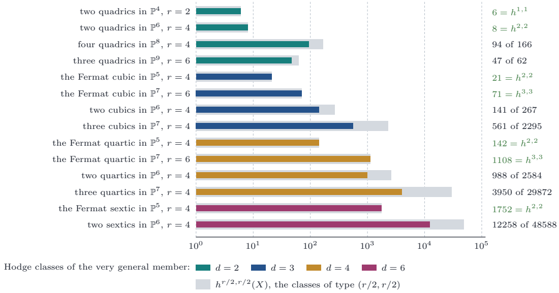
FIGURE 47. The dimension of the space of Hodge classes of degree r on the very general member, from Theorem 20.64(iii), against the Hodge number h^{r/2, r/2} , on a logarithmic scale. Where the two agree, the space H^{r/2, r/2} is spanned by Hodge classes at every configuration; elsewhere the very general member has fewer Hodge classes, and the members with more lie over a countable union of proper closed subsets of the space of configurations.
