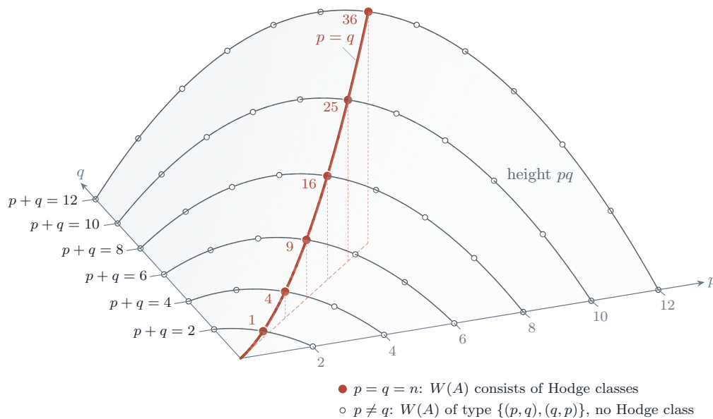
FIGURE 63. The signatures (p, q) of an imaginary quadratic action, with p + q = \dim A , drawn on the surface of height pq , which is the dimension of the family of abelian varieties carrying that action, the unitary Shimura variety of signature (p, q) . Each curve on the surface collects the signatures available in one dimension, and on it the diagonal point is the highest. The divisibility conditions of Theorem C.3 put no constraint on which of them occur when \text{End}^0(A) = K , by Proposition C.9(i) . By Proposition C.7 the Weil line consists of Hodge classes exactly at the filled points on the ridge p = q , and at every open point it is a rational sub-Hodge structure of type \{(p, 2n - p), (2n - p, p)\} carrying no Hodge class at all. The diagonal is the locus that Corollary B.9 shows to be an algebraic subvariety of the moduli.
