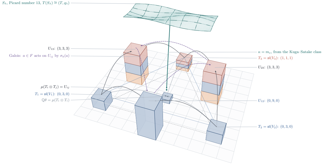
FIGURE 53. Proposition 21.2 and Lemma 21.3 , drawn over the triangle of the three factors of the Hodge group; every height is a dimension. At the corners stand the summands T_i = \mathfrak{sl}(V_i) of T = \text{Lie } G , banded by Hodge type after the Tate twist T(-1) : blue for (1, 1) , clay for (2, 0) and amber for (0, 2) , so that only T_3 carries the K3 type. On the edges stand the three summands U_{ij} of the primitive part of H^2(X) , of dimension nine, U_{12} of pure type (1, 1) and the other two in three bands of three; in the middle is the line of \theta . The solid arcs are the product map \mu , which carries T_i \otimes T_j onto U_{ij} , and the dashed ones carry T_i \otimes T_i to \mathbb{Q}\theta . The violet arcs are the Galois group permuting the U_{ij} as it permutes the embeddings of F , which is why the two exceptional classes may be taken to be the trace-zero part of a cubic field. Above, the K3 surface S_\lambda of Theorem 21.4 , whose Kuga–Satake class, if algebraic, comes down to T as the map \kappa = m_e .
