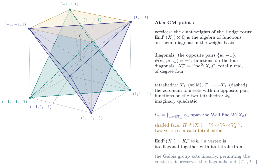
FIGURE 42. Proposition 21.29(i) . The eight weights (\pm 1, \pm 1, \pm 1) of the Hodge torus at a CM point are the vertices of a cube. The four diagonals are the pairs of opposite weights, paired by the polarisation; the two inscribed tetrahedra T_+ (an even number of entries -1 ) and T_- = -T_+ are the only zero-sum four-sets without an opposite pair, and t_{\pm} = \prod_{w \in T_{\pm}} e_w span the Weil line. The Galois group acts by linear maps permuting the vertices, so it preserves the diagonals and the pair of tetrahedra: the functions constant on the tetrahedra form the imaginary quadratic Weil field k_c , those constant on the diagonals the totally real quartic algebra K_c^+ of Rosati-fixed endomorphisms, and \text{End}^0(X_c) = K_c^+ \otimes k_c because a vertex is determined by its diagonal and its tetrahedron.
