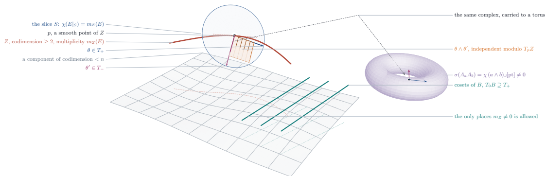
FIGURE 18. The proof of Theorem 16.38 . The grey sheet stands for a component of the support of codimension less than n , which the theorem forces to exist; the clay curve Z for a component of codimension at least two. At a smooth point p of Z the directions \theta \in T_+ and \theta' \in T_- span the slice S , transverse to Z , on which E restricts to a complex of finite length with Euler characteristic m_Z(E) ; the amber parallelogram is the bivector \theta \wedge \theta' , independent modulo T_p Z . Carried to a torus of the same dimension, the product of the two jet classes is seen by the semiregularity map as m_Z(E) times the class of a point contracted with the bivector, which is not zero, so m_Z(E) = 0 or the bivector degenerates. The teal lines are cosets of an abelian subvariety B tangent to T_+ , the only components of codimension at least two on which a nonzero multiplicity survives. The scene is schematic in the dimensions and exact in the incidences.
