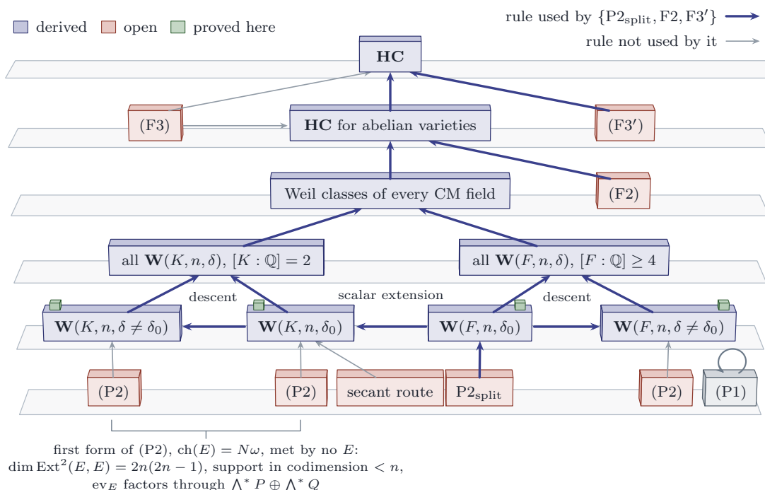
FIGURE 38. The route of this paper through the rule set of Theorem 20.58, drawn as a stack of plates, one per level of the derivation; the other routes are drawn in Figure 37. Heavy arrows are the rules used by the minimal set \{P2_{\text{split}}, F2, F3'\} , light arrows the rules it does not use. The bottom plate carries the propagation statement, read in the corrected form of Remark 17.6, once for each of the four kinds of Weil family, with the secant route beside it. The small grass blocks on the next plate are the base points of Theorem 15.27 and Theorem 19.4, one in every family. The three arrows inside that plate are Proposition 20.13: descent from the trivial discriminant to the others, and scalar extension from the fields of degree at least four to the quadratic fields. With them (P2) is needed only for the split families of the fields of higher degree, and the other three (P2) blocks are not used. (F2) is the conjecture for the Hodge classes that no Weil line reaches, and (F3) is the whole conjecture (Proposition 20.35), so the route is minimal only with (F3) replaced by (F3') of Definition 20.36. The bracket under the two quadratic (P2) blocks records the first form of the criterion, in which the Chern character is exactly a Weil class, as Theorem 16.36, Theorem 16.38 and Corollary 16.34 describe it; by Theorem 17.5 that form is met by no complex. The secant route reaches the trivial discriminant, since the member it is built on is split, and through descent the rest of the quadratic case; it has no edge to the fields of higher degree. The bounded criterion (P1) stands apart, closed on itself: it is equivalent to its own conclusion.
