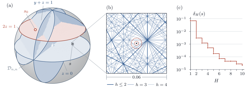
FIGURE 16. The dichotomy of Corollary 16.5. Each stratum \Sigma_{\underline{P},\underline{q}} is Zariski closed by Theorem 16.4, and there are countably many of them; the base point s_0 of Theorem 15.27 lies on one. By Proposition 16.7 the union of the strata is dense, so every neighbourhood of a point s lying off all of them meets infinitely many strata. The conjecture for the family is the assertion that no such s exists, and by Corollary 16.5 it is enough that one stratum has nonempty interior.
