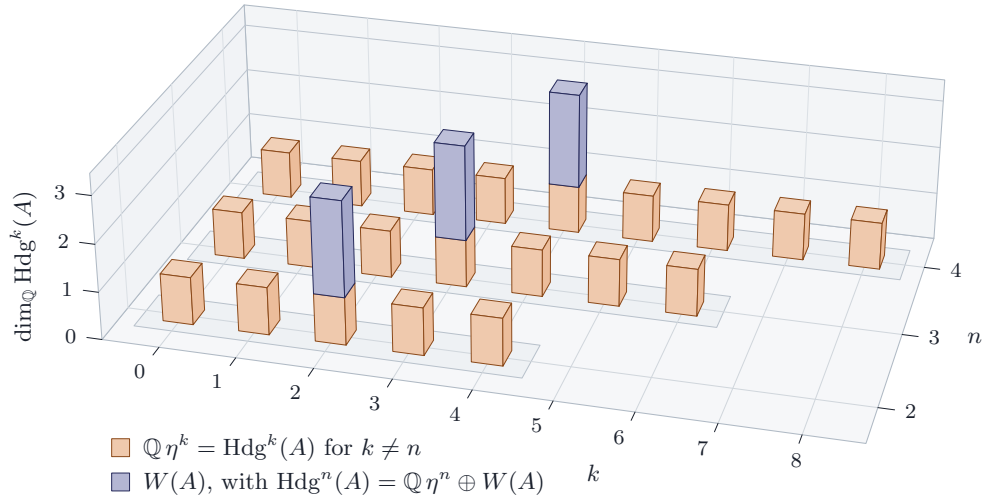
FIGURE 2. The dimensions of \text{Hdg}^k(A) for a general abelian variety of (K, -1, n) -Weil type, 0 \leq k \leq 2n , at n = 2, 3, 4 , as computed in Theorem 4.14 . Every degree carries the line \mathbb{Q}\eta^k ; the middle degree k = n carries in addition the two dimensions of the Weil line W(A) , and nothing else occurs. The profile is the same for every n .
