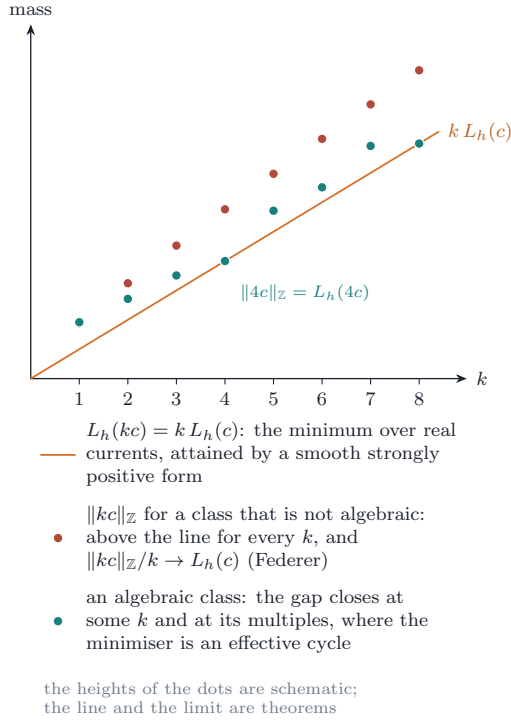
FIGURE 39. Theorem 20.68 and Example 20.69. Left: the mass of a current in the class dual to kc against k . The line k L_h(c) is the minimum over closed real normal currents, attained by a smooth strongly positive form; the minima over closed integral currents lie on or above it, with \|kc\|_{\mathbb{Z}}/k \rightarrow L_h(c) by Federer's theorem, and for M large the class is algebraic exactly when one of them lies on the line, where the minimiser is an effective algebraic cycle. The heights of the dots are schematic. Right: the numbers of the Mumford square, computed in the split model of item (LXIII). Of the seven terms \binom{6}{k} \theta^k \otimes \theta^{6-k} of \theta_Y^6 only k = 3 pairs with \pi_0 = \frac{1}{4} \theta \otimes \theta , giving 20 \cdot 144 = 2880 , and none pairs with the primitive summands; so L_{\theta_Y}(\omega_a) = 4a_0 , the Wirtinger bound of an exceptional class with a_0 = 0 is zero, and the perturbation of NM\theta_Y^2 by N\omega changes the bound 56NM by nothing.
