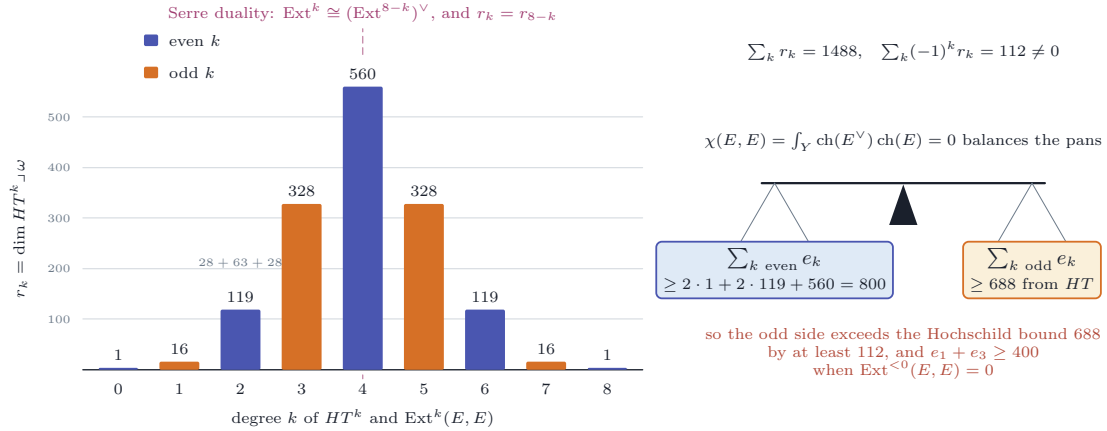
FIGURE 33. Theorem 16.66. Left: the lower bounds r_k for \dim \text{Ext}^k(E, E) when \text{ch}(E) = N\omega , one bar per degree, symmetric about k = 4 as Lemma 16.65 predicts; the bar at k = 2 is the 119 of Theorem 16.56 , made of 28 classes in H^{0,2} , 63 in H^1(T) and 28 bivectors. On the hyperplane L_0 = 0 the bars at 2, 4 and 6 drop to 110, 548 and 110 at a sample point. Right: \chi(E, E) = 0 balances the even and the odd degrees, so the odd side, which Hochschild cohomology fills only to 688, carries at least 800.
