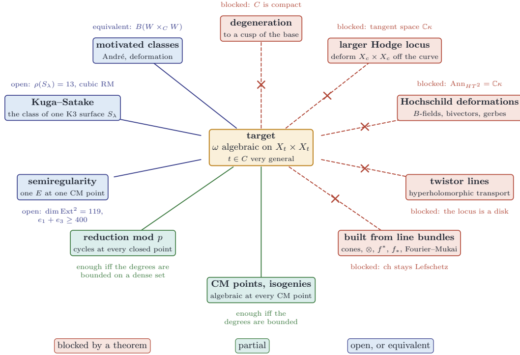
FIGURE 32. Remark 16.64: the ten routes to the Mumford target that avoid the Lefschetz standard conjecture. Clay, with a crossed dashed spoke: a route closed off by a theorem of Section 16.11 or Section 16.12 . Grass: a route that works at special points only, at the CM points or at the closed points of the reductions modulo p , and suffices exactly when a degree bound holds ( Corollary 16.63 , Theorem 16.73 ). Indigo: a route reduced to one open statement, of the same kind as the target or equivalent to it.
