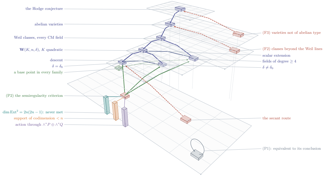
FIGURE 29. The route of this paper in Theorem 16.40 , drawn as a stack of plates, one per level of the derivation; the other routes of the literature are drawn in Figure 28 . The spine in indigo runs from the Weil families at the bottom to the conjecture at the top. The two statements (F2) and (F3) enter in clay from the right, each at the level where it is needed; (F2) is the conjecture for a class of Hodge classes that no Weil line reaches, not a reduction, and (F3) is the whole conjecture ( Proposition 16.35 ), so the route drawn is minimal only with (F3) replaced by (F3') of Definition 16.36 . From below, the propagation statement (P2) in grass reaches the two discriminant cases of the quadratic fields and the fields of higher degree alike, because Theorem 14.48 and Theorem 15.4 put a base point in every family; it is read in the corrected form of Remark 14.100 . The two edges inside the levels are Proposition 16.13 : descent from the trivial discriminant to the others, and scalar extension from the fields of degree at least four to the quadratic fields; with them (P2) is needed only for the split families of the fields of higher degree. The three pillars under the grass node are the results of Theorem 14.89 , Theorem 14.91 and Corollary 14.87 on the first form, in which the Chern character is exactly a Weil class; by Theorem 14.99 that form is never met, so the number on the first pillar is attained by no complex. The secant route in clay reaches the trivial discriminant, since the member it is built on is split, and through descent the rest of the quadratic case; it has no edge to the fields of higher degree. The bounded criterion (P1) is drawn apart, in slate, closed on itself: it is equivalent to its own conclusion.
