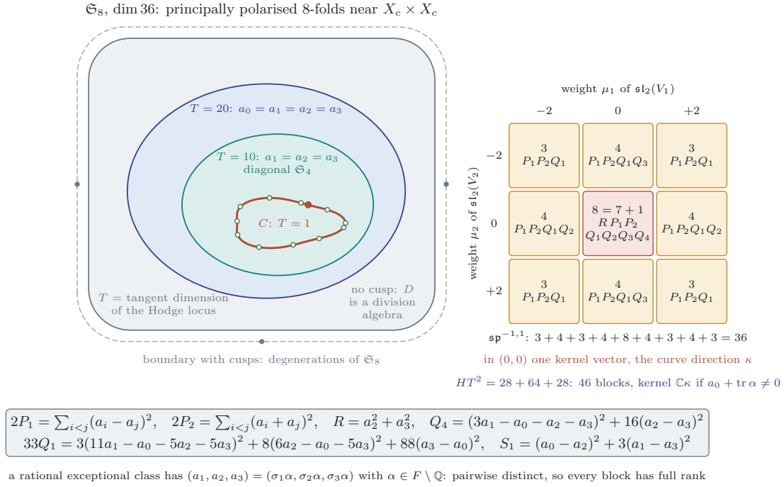
FIGURE 31. Theorem 16.56. Left: the Siegel space \mathfrak{S} of dimension 36 near Y = X_c \times X_c and three Hodge loci through it, labelled by the tangent dimension T at Y : the class with equal coefficients ( T = 20 ), the products of divisor classes with a_1 = a_2 = a_3 ( T = 10 , the diagonal Siegel space), and a rational exceptional class ( T = 1 ), whose locus is the compact Mumford curve with its CM points (hollow). The dashed rim is the boundary of \mathfrak{S} , which the curve does not reach. Right: the nine weight blocks of \mathfrak{sp}^{-1,1} under the torus of the first two factors, with their dimensions and the forms whose product is the Gram determinant of each; only the block of weight (0, 0) has a kernel, the direction \kappa of the curve. The same holds in the 46 blocks of HT^2(Y) off the hyperplane L_0 = 0 . Below: the sums of squares that make the determinants nonzero at the conjugates of an irrational element of F .
