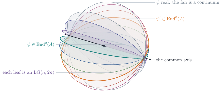
FIGURE 15. Proposition 14.45 , drawn as a pencil. Each admissible \psi gives one leaf, an open piece of \text{LG}(n, V_+, \omega_\psi) of dimension n(n+1)/2 , and the leaves through a common axis form a continuous family as \psi varies over the reals, so they sweep \mathcal{D}_{n,n} . The two drawn heavy are the ones whose \psi is rational, and only those are quaternionic loci of an actual abelian variety. The picture is exact for the pencil it draws; in the family the leaves have dimension n(n+1)/2 inside n^2 and the parameter is not one real number but a variety of them. 27
