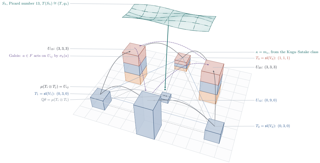
FIGURE 30. Proposition 16.49 and Lemma 16.50 , drawn over the triangle of the three factors of the Hodge group; every height is a dimension. At the corners stand the summands T_i = \mathfrak{sl}(V_i) of T = \text{Lie } G , banded by Hodge type after the Tate twist T(-1) : blue for (1, 1) , clay for (2, 0) and amber for (0, 2) , so that only T_3 carries the K3 type. On the edges stand the three summands U_{ij} of the primitive part of H^2(X) , of dimension nine, U_{12} of pure type (1, 1) and the other two in three bands of three; in the middle is the line of \theta . The solid arcs are the product map \mu , which carries T_i \otimes T_j onto U_{ij} , and the dashed ones carry T_i \otimes T_i to \mathbb{Q}\theta . The violet arcs are the Galois group permuting the U_{ij} as it permutes the embeddings of F , which is why the two exceptional classes may be taken to be the trace-zero part of a cubic field. Above, the K3 surface S_\lambda of Theorem 16.51 , whose Kuga–Satake class, if algebraic, comes down to T as the map \kappa = m_e .
