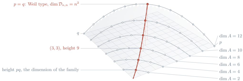
FIGURE 34. The signatures (p, q) of an imaginary quadratic action, with p + q = \dim A , drawn on the surface of height pq , which is the dimension of the family of abelian varieties carrying that action, the unitary Shimura variety of signature (p, q) . Each curve on the surface collects the signatures available in one dimension, and on it the diagonal point is the highest. The divisibility conditions of Theorem C.3 put no constraint on which of them occur when \text{End}^0(A) = K , by Proposition C.9(i). By Proposition C.7 the Weil line consists of Hodge classes exactly at the filled points on the ridge p = q , and at every open point it is a rational sub-Hodge structure of type \{(p, 2n - p), (2n - p, p)\} carrying no Hodge class at all. The diagonal is the locus that Corollary B.9 shows to be an algebraic subvariety of the moduli.
