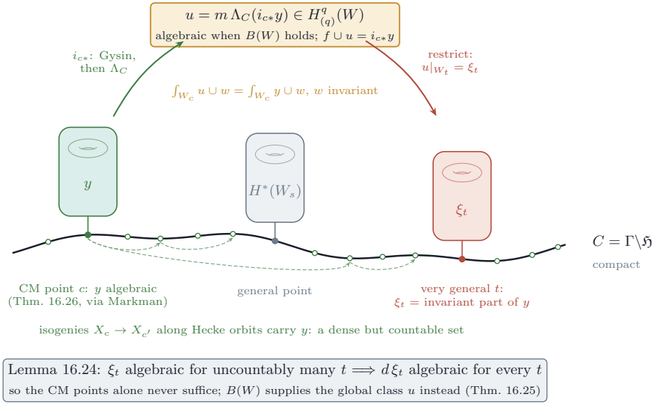
FIGURE 27. Theorem 16.29(ii) along a compact Shimura curve C . An algebraic class y on one fibre, at a base point of a Weil family or at a CM point of a Mumford family (hollow dots: the CM points, countable and dense), is pushed into W by the Gysin map and brought back to the invariant summand by the base operator \Lambda_C . When B(W) holds the result u is an algebraic class on W , pinned down by the displayed pairing against the invariant classes, and its restriction to a very general fibre is the invariant part of y . The dashed arcs are isogenies between CM members along Hecke orbits: they carry algebraic classes to algebraic classes but reach only countably many points, and Lemma 16.28 , in the box, needs uncountably many. This is how Corollary 16.32 and Corollary 16.31 turn each target into one case of (L).
