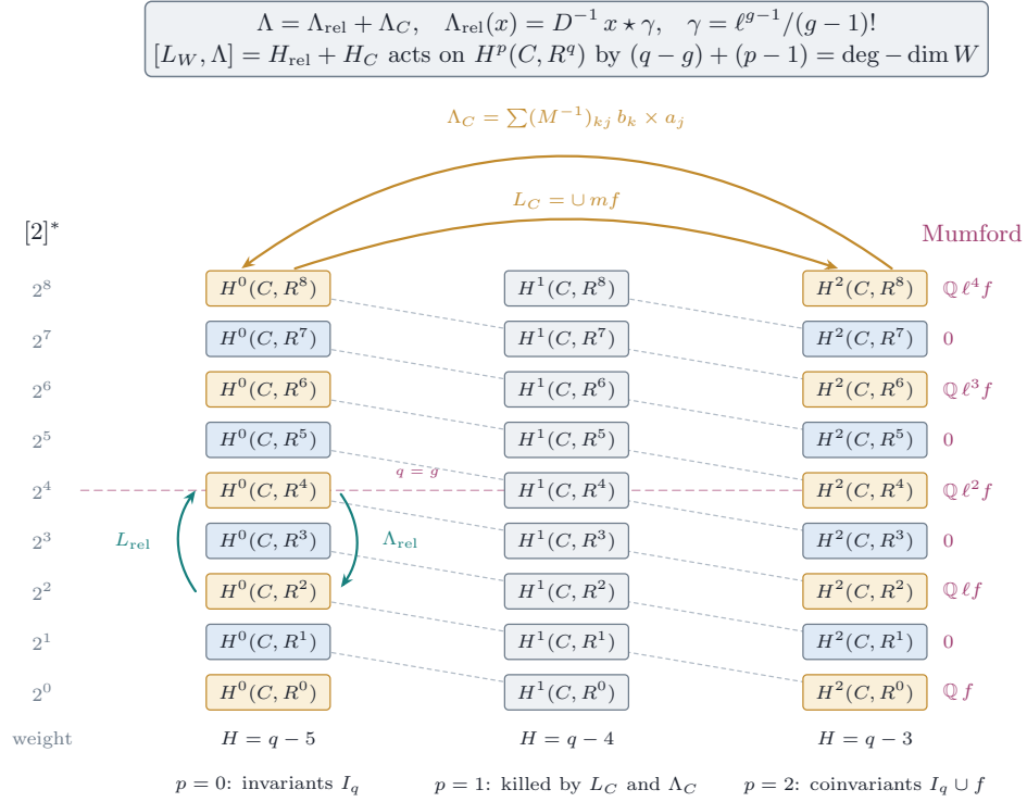
FIGURE 26. The proof of Theorem 16.22 for relative dimension four. The boxes are the summands H^p(C, R^q \pi_* \mathbb{Q}) of H^*(W, \mathbb{Q}) , split off by the eigenvalue 2^q of [2]^* shown on the left; the dotted diagonals join the summands of one H^k(W, \mathbb{Q}) , k = p + q , and the dashed magenta line is the axis q = g of hard Lefschetz on the fibres. The relative operators L_{\text{rel}} and \Lambda_{\text{rel}} , in teal, move within a column; \Lambda_{\text{rel}} is a Pontryagin product with an algebraic class on every abelian scheme ( Proposition 16.21 ). The base operators L_C and \Lambda_C , in ochre, move along a row between the outer columns and kill the middle one; \Lambda_C is the displayed cycle built from bases (a_j) , (b_k) of the invariant summands, and is algebraic exactly when the invariant cycles are. Below each column is the weight of H = [L_W, \Lambda] on it, and the panel at the top is Step 6 of the proof. The ochre boxes carry the invariant cycles and their images under L_C ; for a Mumford family they are the lines listed in magenta on the right, spanned by \ell^i f (and by \ell^i in the left column), and the other boxes of the outer columns are zero ( Corollary 16.23 ).
