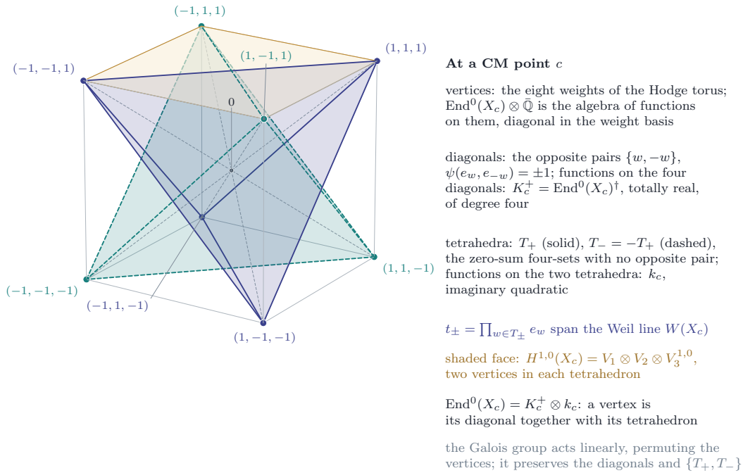
FIGURE 40. Proposition 21.29(i) . The eight weights (\pm 1, \pm 1, \pm 1) of the Hodge torus at a CM point are the vertices of a cube. The four diagonals are the pairs of opposite weights, paired by the polarisation; the two inscribed tetrahedra T_+ (an even number of entries -1 ) and T_- = -T_+ are the only zero-sum four-sets without an opposite pair, and t_{\pm} = \prod_{w \in T_{\pm}} e_w span the Weil line. The Galois group acts by linear maps permuting the vertices, so it preserves the diagonals and the pair of tetrahedra: the functions constant on the tetrahedra form the imaginary quadratic Weil field k_c , those constant on the diagonals the totally real quartic algebra K_c^+ of Rosati-fixed endomorphisms, and \text{End}^0(X_c) = K_c^+ \otimes k_c because a vertex is determined by its diagonal and its tetrahedron.
