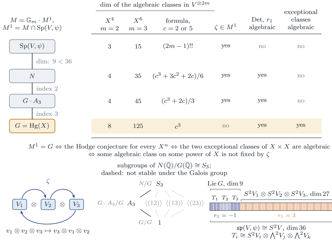
FIGURE 44. The four possible groups M^1 = M \cap \mathrm{Sp}(V, \psi) of Proposition 21.47, where M = \mathbb{G}_m \cdot M^1 , as the chain G \subset G \cdot A_3 \subset N \subset \mathrm{Sp}(V, \psi) : the first two inclusions have index 3 and 2, and N , whose identity component is G , has dimension 9 against 36. For each case the table gives the dimension of the algebraic classes in the multilinear part V^{\otimes 2m} of H^{2m}(X^{2m}, \mathbb{Q}) for m = 2 and m = 3 , from the c = 2 , respectively c = 5 , non-crossing pairings (item (LX) of Appendix D); whether M^1 contains the cyclic permutation \zeta of the three tensor factors; whether Det and r_1 are algebraic; and whether the two exceptional classes of X \times X are. Only M^1 = G makes the exceptional classes algebraic, and it is equivalent to the Hodge conjecture for every power of X (Proposition 21.47(ii)); the proposition does not decide which of the four cases occurs. Below, from left to right: \zeta ; the subgroups of N(\bar{\mathbb{Q}})/G(\bar{\mathbb{Q}}) \cong S_3 , of which only 1, A_3 and S_3 are stable under the Galois group, which acts transitively on the three factors; and \mathfrak{sp}(V, \psi) = \mathrm{Lie} G \oplus S^2 V_1 \otimes S^2 V_2 \otimes S^2 V_3 , 36 = 9 + 27 , the second summand irreducible under G , with the eigenvalues -1 and 3 of r_1 on the two summands.
