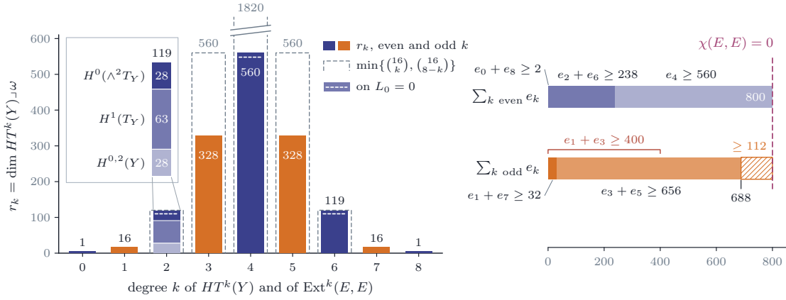
FIGURE 43. Theorem 21.34. Left: the lower bounds r_k for \dim \text{Ext}^k(E, E) when \text{ch}(E) = N\omega , one bar per degree, symmetric about k = 4 as Lemma 21.33 predicts; the bar at k = 2 is the 119 of Theorem 21.21 , made of 28 classes in H^{0,2} , 63 in H^1(T) and 28 bivectors. On the hyperplane L_0 = 0 the bars at 2, 4 and 6 drop to 110, 548 and 110 at a sample point. Right: \chi(E, E) = 0 balances the even and the odd degrees, so the odd side, which Hochschild cohomology fills only to 688, carries at least 800.
