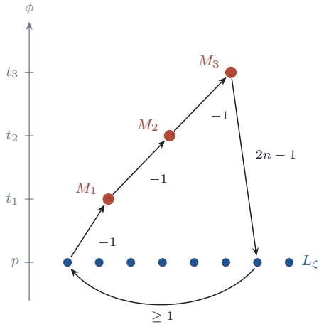
(a) the excess of a cycle, n \geq 3
