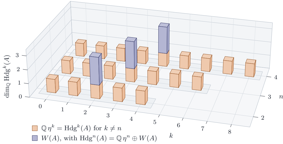
FIGURE 4. The dimensions of \text{Hdg}^k(A) for a general abelian variety of (K, -1, n) -Weil type, 0 \leq k \leq 2n , at n = 2, 3, 4 , as computed in Theorem 4.14 . Every degree carries the line \mathbb{Q}\eta^k ; the middle degree k = n carries in addition the two dimensions of the Weil line W(A) , and nothing else occurs. The profile is the same for every n .
