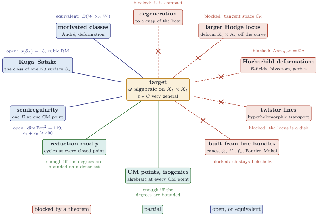
FIGURE 29. Remark 16.57: the ten routes to the Mumford target that avoid the Lefschetz standard conjecture. Clay, with a crossed dashed spoke: a route closed off by a theorem of Section 16.11 or Section 16.12 . Grass: a route that works at special points only, at the CM points or at the closed points of the reductions modulo p , and suffices exactly when a degree bound holds ( Corollary 16.56 , Theorem 16.66 ). Indigo: a route reduced to one open statement, of the same kind as the target or equivalent to it.
