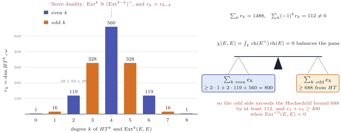
FIGURE 30. Theorem 16.59. Left: the lower bounds r_k for \dim \text{Ext}^k(E, E) when \text{ch}(E) = N\omega , one bar per degree, symmetric about k = 4 as Lemma 16.58 predicts; the bar at k = 2 is the 119 of Theorem 16.49 , made of 28 classes in H^{0,2} , 63 in H^1(T) and 28 bivectors. On the hyperplane L_0 = 0 the bars at 2, 4 and 6 drop to 110, 548 and 110 at a sample point. Right: \chi(E, E) = 0 balances the even and the odd degrees, so the odd side, which Hochschild cohomology fills only to 688, carries at least 800.
