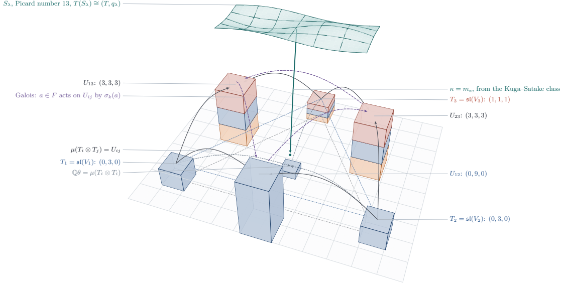
FIGURE 27. Proposition 16.42 and Lemma 16.43 , drawn over the triangle of the three factors of the Hodge group; every height is a dimension. At the corners stand the summands T_i = \mathfrak{sl}(V_i) of T = \text{Lie } G , banded by Hodge type after the Tate twist T(-1) : blue for (1, 1) , clay for (2, 0) and amber for (0, 2) , so that only T_3 carries the K3 type. On the edges stand the three summands U_{ij} of the primitive part of H^2(X) , of dimension nine, U_{12} of pure type (1, 1) and the other two in three bands of three; in the middle is the line of \theta . The solid arcs are the product map \mu , which carries T_i \otimes T_j onto U_{ij} , and the dashed ones carry T_i \otimes T_i to \mathbb{Q}\theta . The violet arcs are the Galois group permuting the U_{ij} as it permutes the embeddings of F , which is why the two exceptional classes may be taken to be the trace-zero part of a cubic field. Above, the K3 surface S_\lambda of Theorem 16.44 , whose Kuga–Satake class, if algebraic, comes down to T as the map \kappa = m_e .
