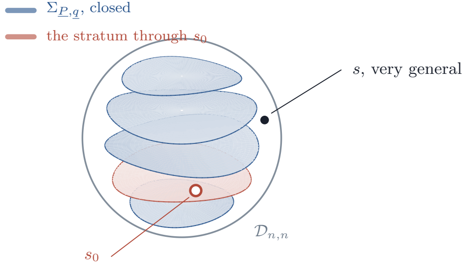
FIGURE 16. The dichotomy of Corollary 14.58. Each stratum \Sigma_{\underline{P},q} is Zariski closed by Theorem 14.57, and there are countably many of them; the base point s_0 of Theorem 14.48 lies on one. By Proposition 14.60 the union of the strata is dense, so a point s off all of them is squeezed between strata however small a neighbourhood is taken. The conjecture for the family is the assertion that no such s exists, and by Corollary 14.58 it is enough that one stratum has nonempty interior.
