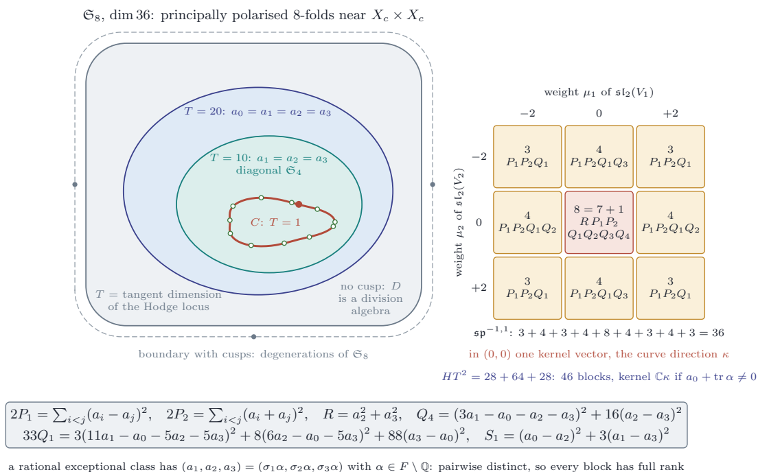
FIGURE 28. Theorem 16.49. Left: the Siegel space \mathfrak{S} of dimension 36 near Y = X_c \times X_c and three Hodge loci through it, labelled by the tangent dimension T at Y : the class with equal coefficients ( T = 20 ), the products of divisor classes with a_1 = a_2 = a_3 ( T = 10 , the diagonal Siegel space), and a rational exceptional class ( T = 1 ), whose locus is the compact Mumford curve with its CM points (hollow). The dashed rim is the boundary of \mathfrak{S} , which the curve does not reach. Right: the nine weight blocks of \mathfrak{sp}^{-1,1} under the torus of the first two factors, with their dimensions and the forms whose product is the Gram determinant of each; only the block of weight (0, 0) has a kernel, the direction \kappa of the curve. The same holds in the 46 blocks of HT^2(Y) off the hyperplane L_0 = 0 . Below: the sums of squares that make the determinants nonzero at the conjugates of an irrational element of F .
