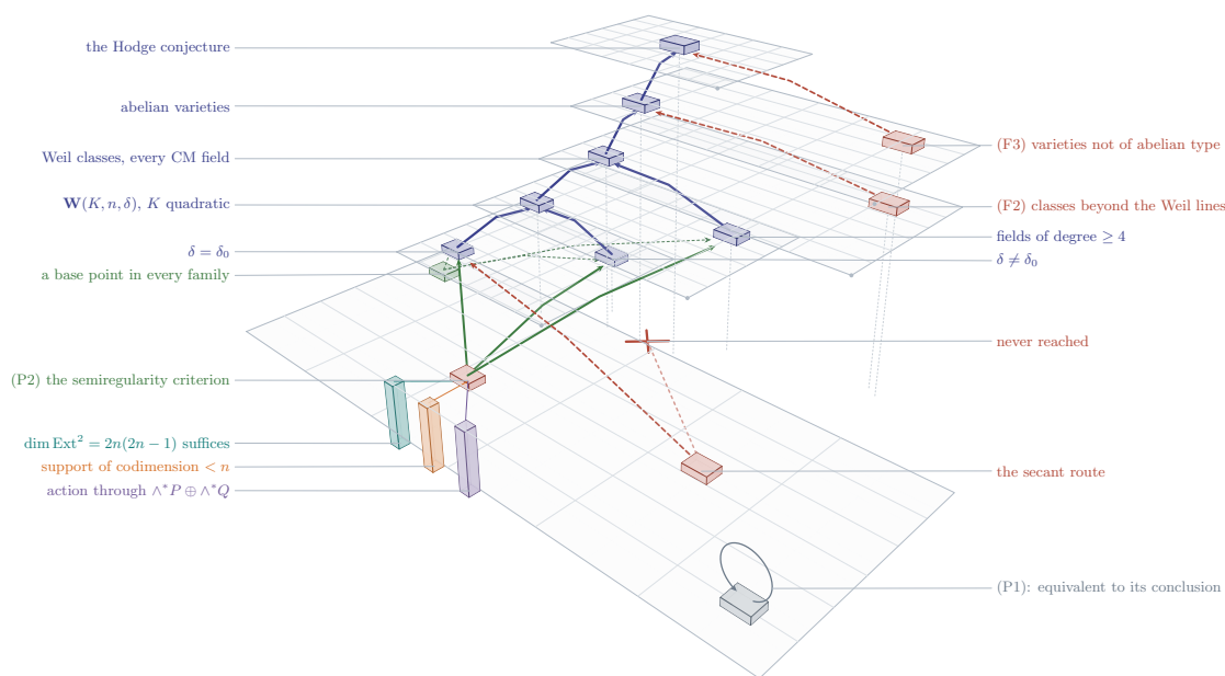
FIGURE 26. The route of this paper in Theorem 16.33 , drawn as a stack of plates, one per level of the derivation; the other routes of the literature are drawn in Figure 25 . The spine in indigo runs from the Weil families at the bottom to the conjecture at the top. The two statements (F2) and (F3) enter in clay from the right, each at the level where it is needed; (F2) is the conjecture for a class of Hodge classes that no Weil line reaches, not a reduction, and (F3) is the whole conjecture ( Proposition 16.31 ), so the route drawn is sufficient and not minimal. From below, the propagation statement (P2) in grass reaches the two discriminant cases of the quadratic fields and the fields of higher degree alike, because Theorem 14.48 and Theorem 15.4 put a base point in every family; the three constraints on it proved in Theorem 14.89 , Theorem 14.91 and Corollary 14.87 are drawn as the pillars under the grass node. The secant route in clay reaches the trivial discriminant and stops there, since the member it is built on is split; the crossed edge is the one implication it would need and does not have. The bounded criterion (P1) is drawn apart, in slate, closed on itself: it is equivalent to its own conclusion.
