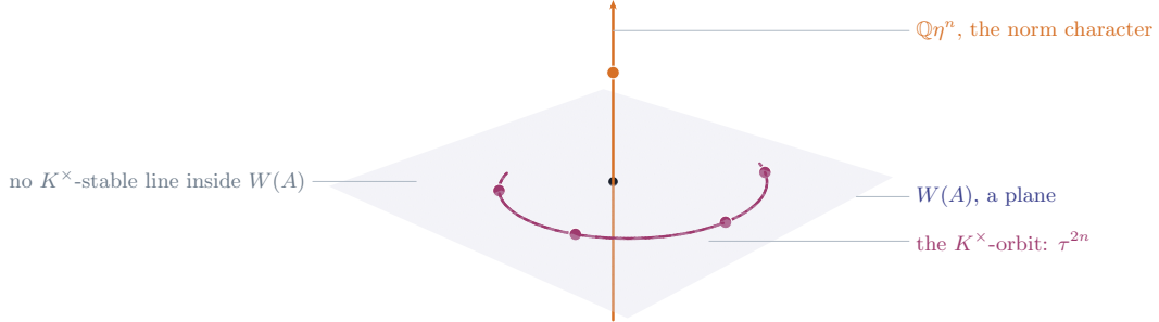
FIGURE 4. The linear algebra behind Theorem 1.1 , drawn inside H^{2n}(A, \mathbb{Q}) . The Weil line W(A) is a plane, free of rank one over K and of rank two over \mathbb{Q} , and K^\times acts on it through \tau^{2n} , so the orbit of any nonzero class is a spiral that spans the plane and lies on no line in it. The transverse axis carries \eta^n , on which K^\times acts through the norm. A construction returning a single eigenclass returns a line, and by Proposition 13.1 no line inside W(A) is stable.
