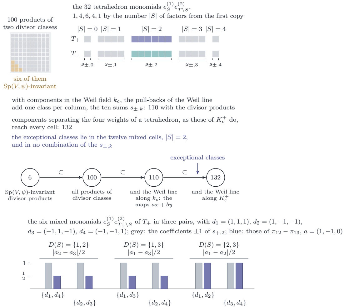
FIGURE 39. Proposition 21.29(ii) and (iii). Top: the 132 Hodge classes of degree four on the square at a CM point, one cell per monomial of weight zero. The 100 products of divisor classes are the cells with an opposite pair; the 32 tetrahedron monomials e_S^{(1)} e_{T \setminus S}^{(2)} are arranged by tetrahedron and by the number |S| of factors from the first copy. Pull-backs of the Weil line along homomorphisms with components in k_c add only the ten symmetric sums s_{\pm,k} , one per column, giving 110; components separating the four weights of a tetrahedron, as those of K_c^+ do, separate the monomials and give all 132. Bottom: on the six mixed monomials of one tetrahedron, grouped in the three pairs by the coordinates in which the two weights of S differ, the symmetric sum s_{+,2} has coefficients \pm 1 throughout, while an exceptional class \omega_a has coefficients of absolute value |a_2 - a_3|/2 , |a_1 - a_3|/2 , |a_1 - a_2|/2 , drawn for \pi_{12} - \pi_{13} ; two equal absolute values would be a linear relation among the conjugates of an irrational element of F .
