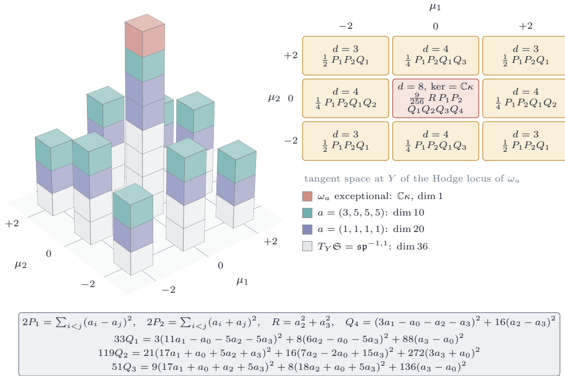
FIGURE 37. Theorem 21.21 . Left: the Siegel space \mathfrak{S} of dimension 36 near Y = X_c \times X_c and three Hodge loci through it, labelled by the tangent dimension T at Y : the class with equal coefficients ( T = 20 ), the products of divisor classes with a_1 = a_2 = a_3 ( T = 10 , the diagonal Siegel space), and a rational exceptional class ( T = 1 ), whose locus is the compact Mumford curve with its CM points (hollow). The dashed rim is the boundary of \mathfrak{S} , which the curve does not reach. Right: the nine weight blocks of \mathfrak{sp}^{-1,1} under the torus of the first two factors, with their dimensions and the forms whose product is the Gram determinant of each; only the block of weight (0, 0) has a kernel, the direction \kappa of the curve. The same holds in the 46 blocks of HT^2(Y) off the hyperplane L_0 = 0 . Below: the sums of squares that make the determinants nonzero at the conjugates of an irrational element of F .
